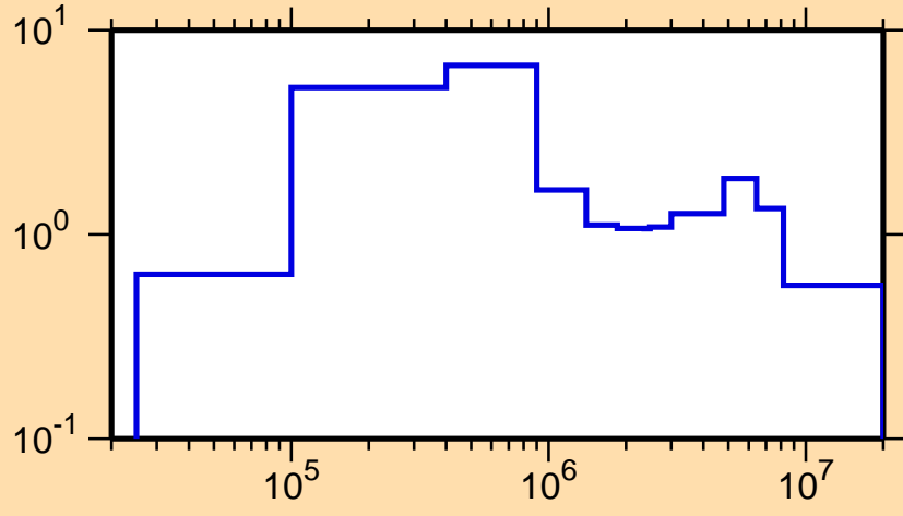
\sigma vs. E for ^{225}\text{Fr}(n,\text{inel.})
