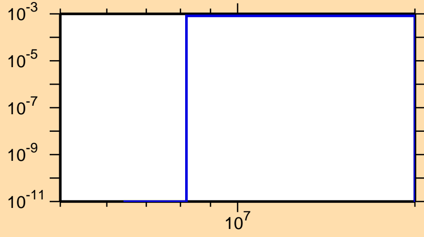
\sigma vs. E for ^{225}\text{Fr}(n,d)
