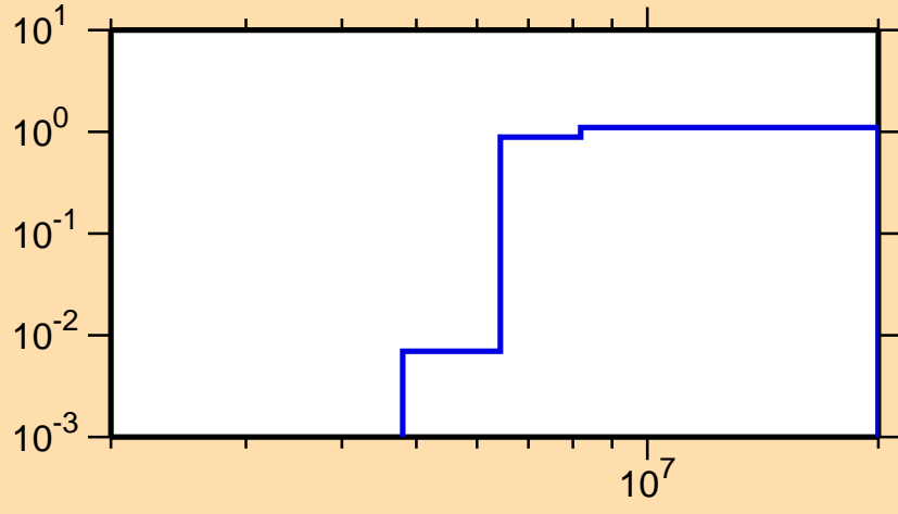
\sigma vs. E for ^{225}\text{Fr}(n,2n)
