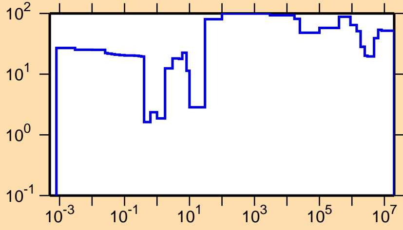
\Delta\sigma/\sigma vs. E for ^{225}\text{Fr}(n,\text{tot.})
