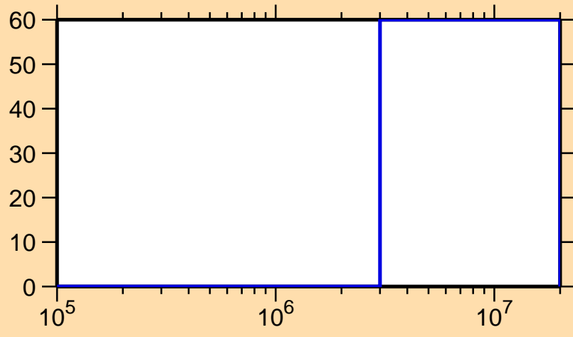
\Delta\sigma/\sigma vs. E for ^{225}\text{Fr}(n,f)
