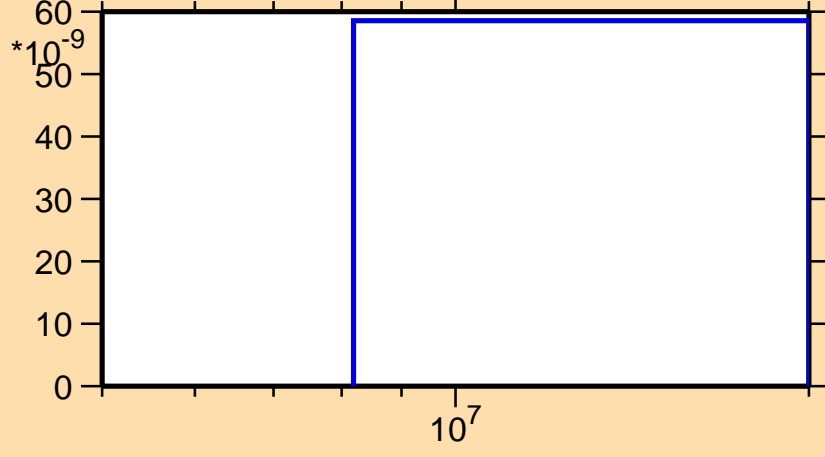
\sigma vs. E for ^{225}\text{Fr}(n,nt)
