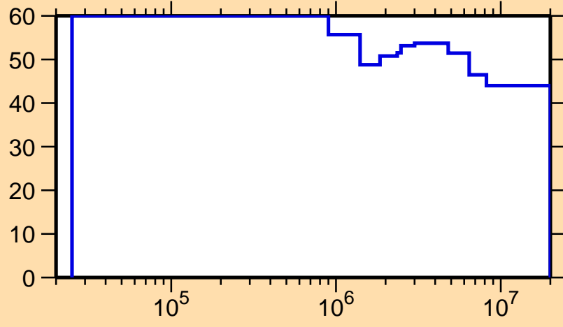
\Delta\sigma/\sigma vs. E for ^{225}\text{Fr}(n,\text{nonel.})
