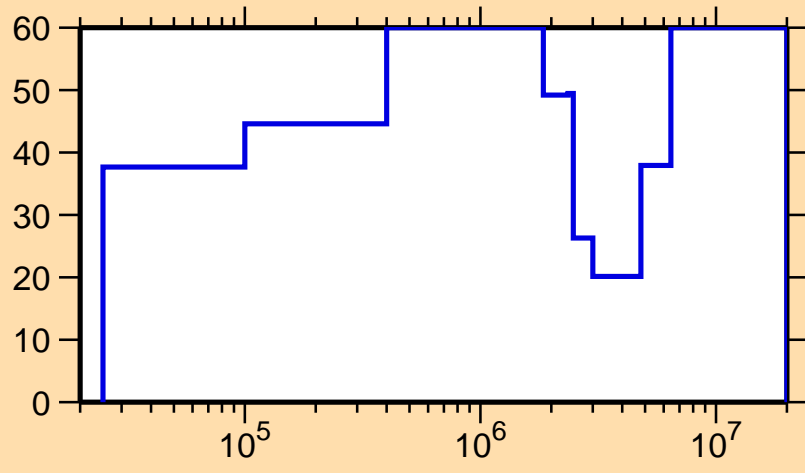
\Delta\sigma/\sigma vs. E for ^{225}\text{Fr}(n,\text{el.})
