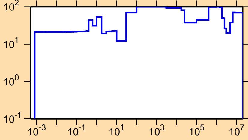
\Delta\sigma/\sigma vs. E for ^{225}\text{Fr}(n,el.)
