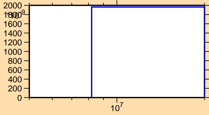
\sigma vs. E for ^{225}\text{Fr}(n,\text{nd})
