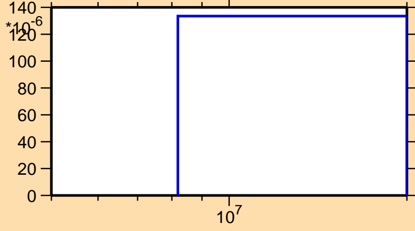
\sigma vs. E for ^{225}\text{Fr}(n,t)
