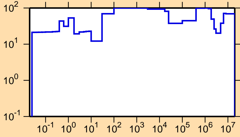
\Delta\sigma/\sigma vs. E for ^{225}\text{Fr}(n,\text{el.})
