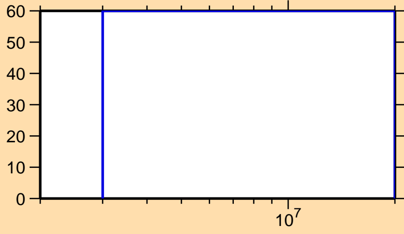
\Delta\sigma/\sigma vs. E for ^{225}\text{Fr}(n,p)
