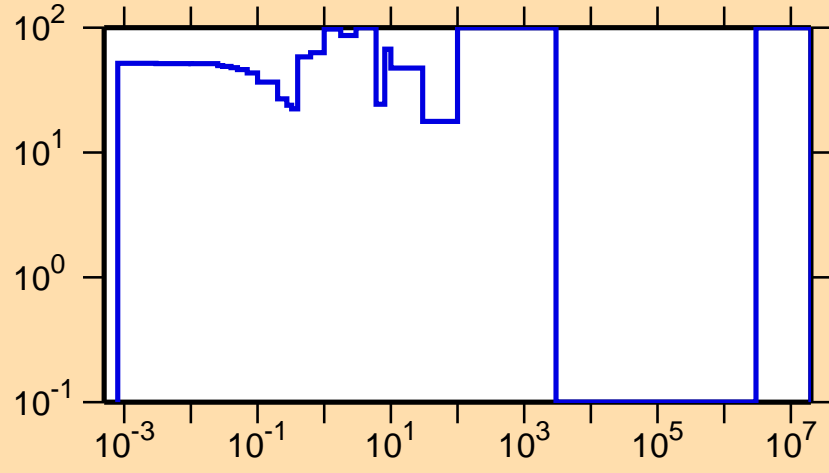
\Delta\sigma/\sigma vs. E for ^{225}\text{Fr}(n,f)
