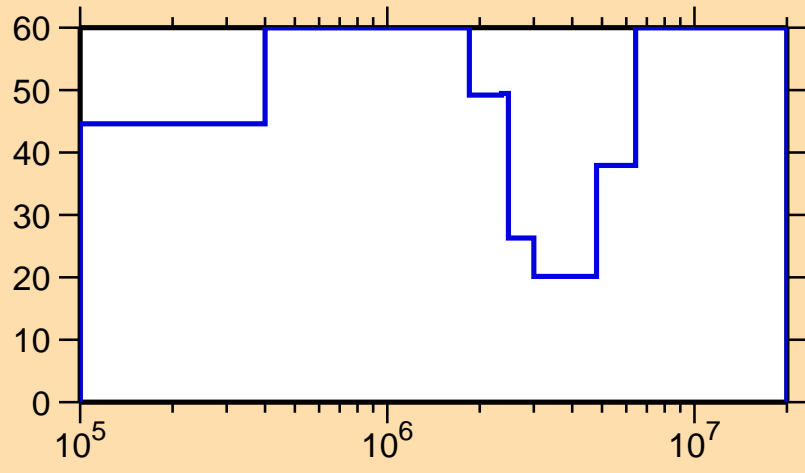
\Delta\sigma/\sigma vs. E for ^{225}\text{Fr}(n, el.)
