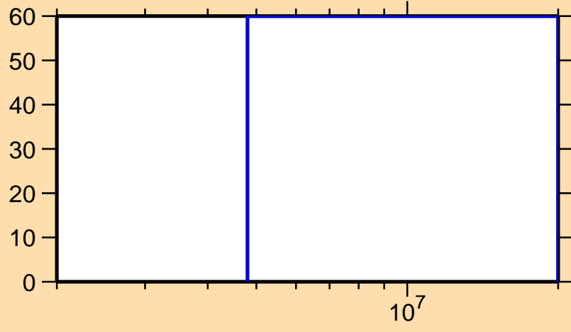
\Delta\sigma/\sigma vs. E for ^{225}\text{Fr}(n,2n)
