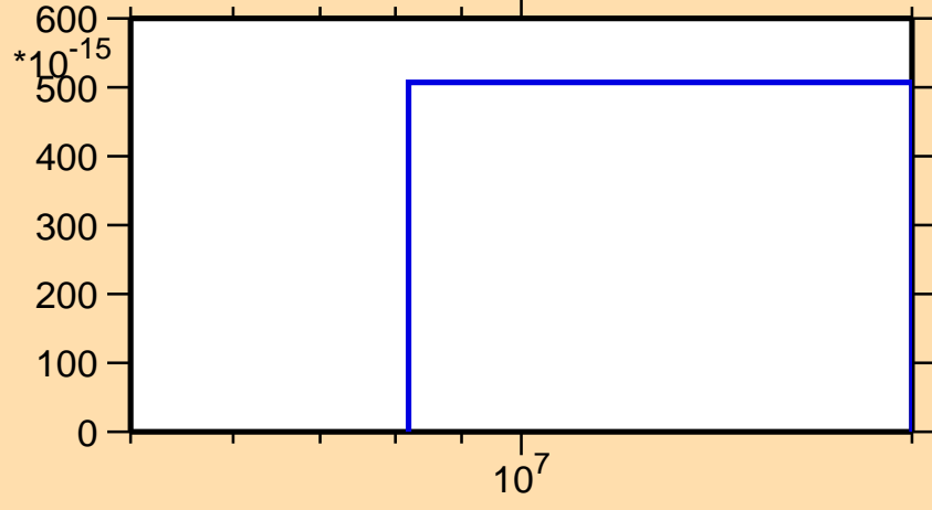
\sigma vs. E for ^{225}\text{Fr}(n,\text{He3})
