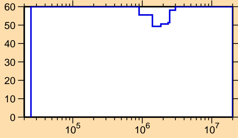
\Delta\sigma/\sigma vs. E for ^{225}\text{Fr}(n,\text{inel.})
