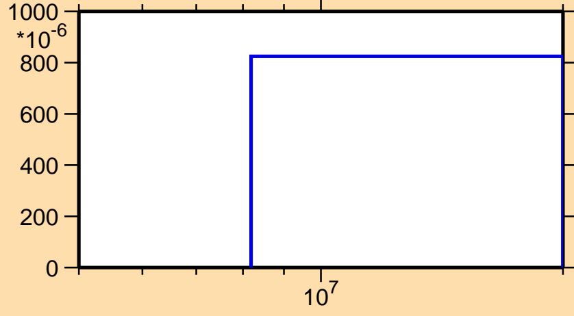
\sigma vs. E for ^{225}\text{Fr}(n,2n\alpha)
