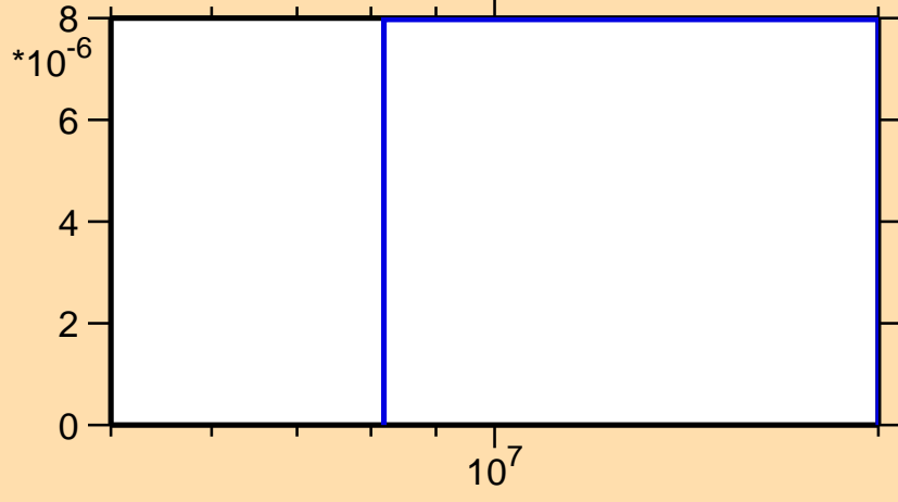
\sigma vs. E for ^{225}\text{Fr}(n,3n\alpha)
