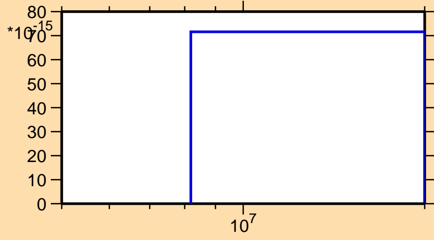
\sigma vs. E for ^{225}\text{Fr}(\text{mt } 11)
