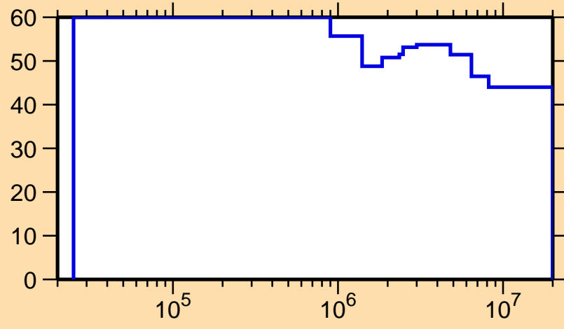
\Delta\sigma/\sigma vs. E for ^{225}\text{Fr}(n,\text{nonel.})
