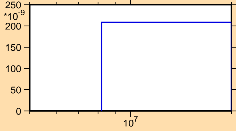
\sigma vs. E for ^{225}\text{Fr}(n,2np)
