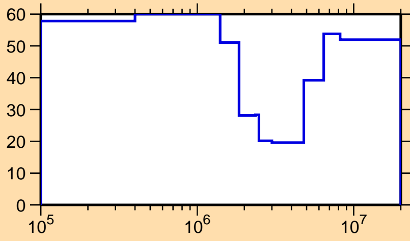
\Delta\sigma/\sigma vs. E for ^{225}\text{Fr}(n,\text{tot.})
