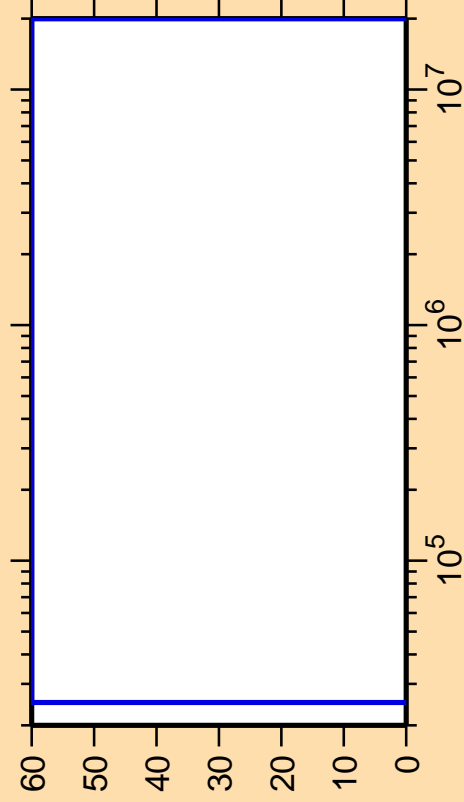
\Delta\sigma/\sigma vs. E for ^{225}\text{Fr}(n,n_1)
