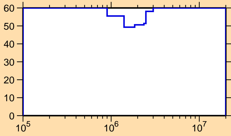
\Delta\sigma/\sigma vs. E for ^{225}\text{Fr}(n, \text{inel.})
