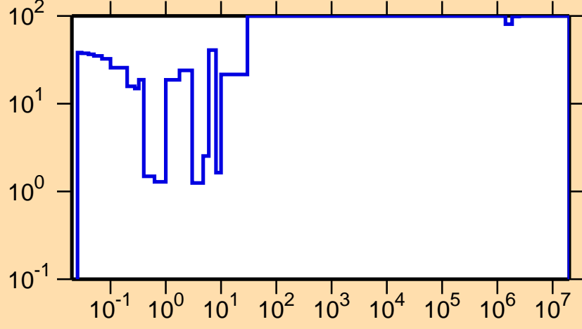
\Delta\sigma/\sigma vs. E for ^{225}\text{Fr}(n,\gamma)
