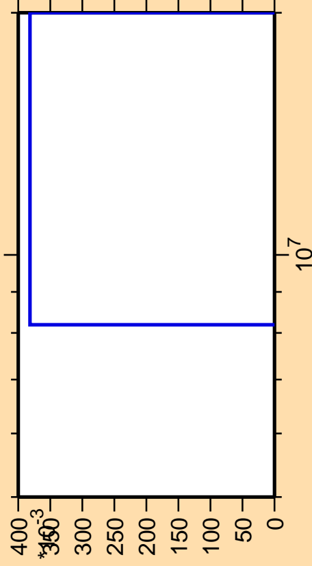
\Delta\sigma/\sigma vs. E for ^{225}\text{Fr}(\text{mt } 11)
