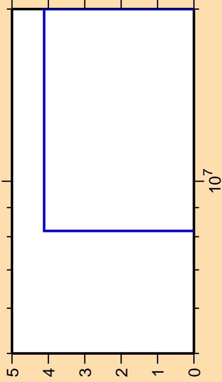
\Delta\sigma/\sigma vs. E for ^{225}\text{Fr}(n,\text{He3})
