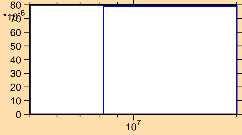
\sigma vs. E for ^{225}\text{Fr}(n,np)
