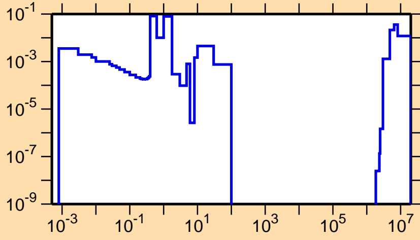
\sigma vs. E for ^{225}\text{Fr}(n,f)
