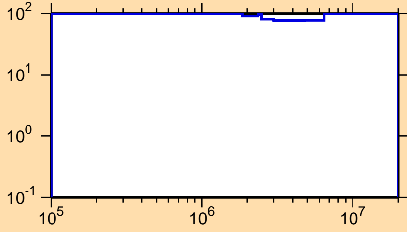
\Delta\sigma/\sigma vs. E for ^{225}\text{Fr}(n, n\text{cont.})
