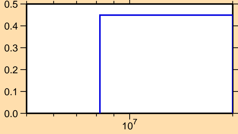
\sigma vs. E for ^{225}\text{Fr}(n,3n)
