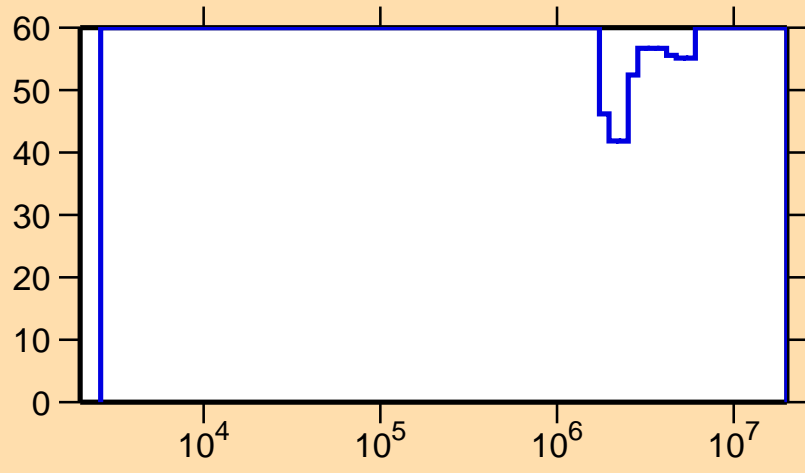
\Delta\sigma/\sigma vs. E for ^{227}\text{Fr}(n,\text{inel.})
