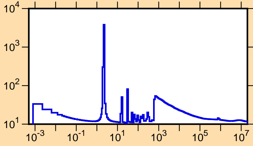
\sigma vs. E for ^{227}\text{Fr}(n,\text{tot.})
