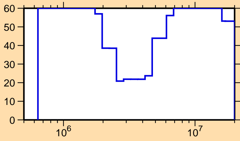
\Delta\sigma/\sigma vs. E for ^{227}\text{Fr}(n, \text{el.})
