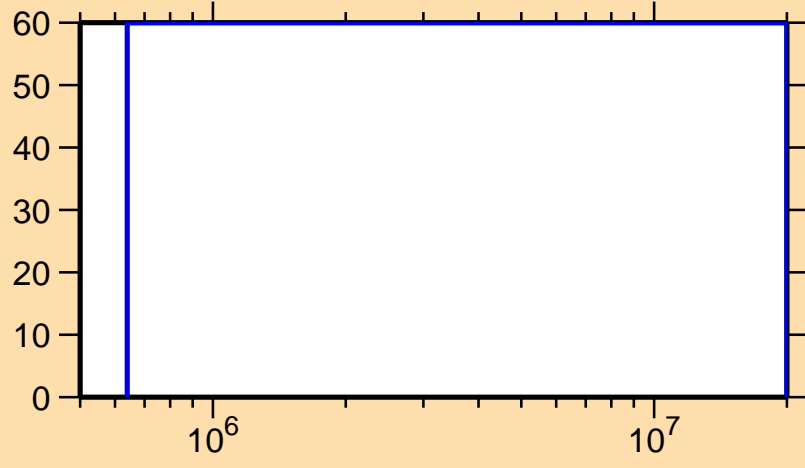
\Delta\sigma/\sigma vs. E for ^{227}\text{Fr}(n,n\text{cont.})
