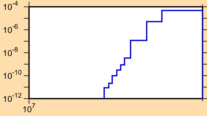
\sigma vs. E for ^{227}\text{Fr}(n,\text{nd})
