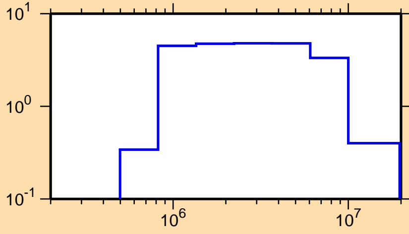
\sigma vs. E for ^{227}\text{Fr}(n,n\text{cont.})
