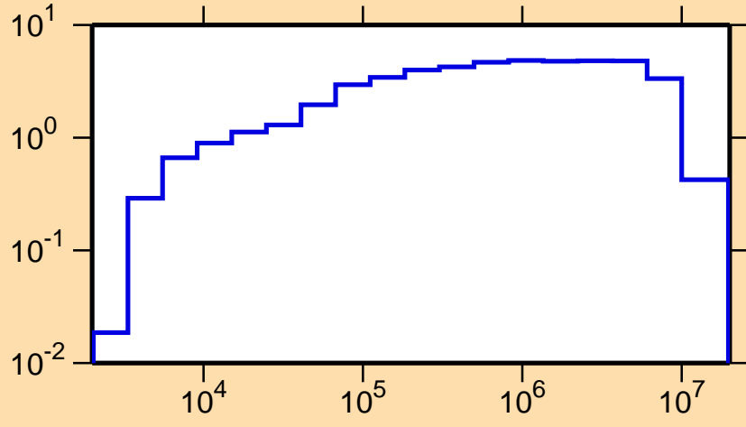
\sigma vs. E for ^{227}\text{Fr}(n,\text{inel.})
