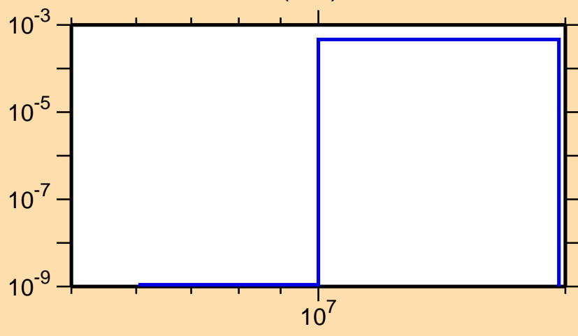
\sigma vs. E for ^{227}\text{Fr}(n,d)
