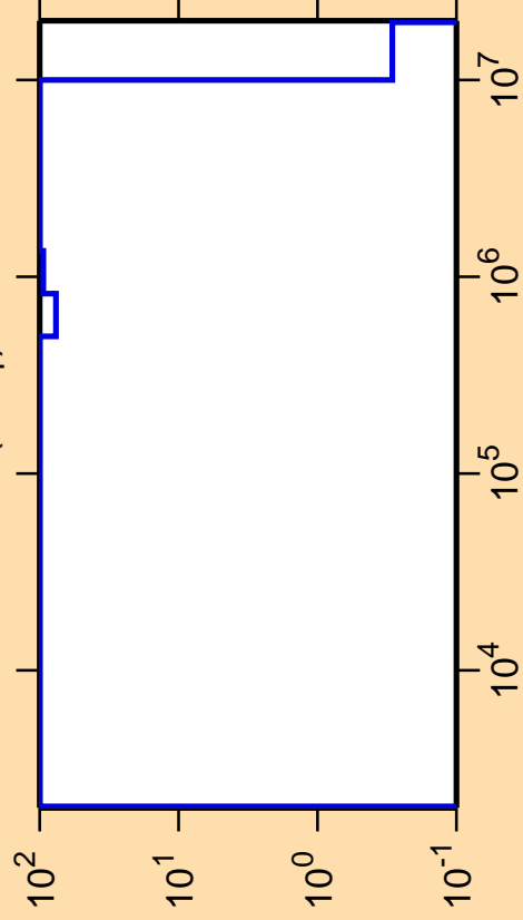
\Delta\sigma/\sigma vs. E for ^{227}\text{Fr}(n,n_1)
