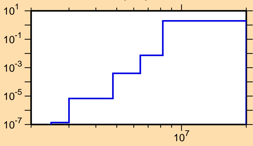
\sigma vs. E for ^{227}\text{Fr}(n,\alpha)
