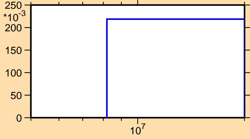
\sigma vs. E for ^{227}\text{Fr}(n,3n)
