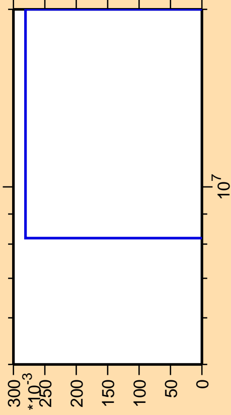
\Delta\sigma/\sigma vs. E for ^{227}\text{Fr}(n,3n\alpha)
