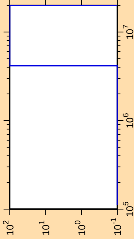
\Delta\sigma/\sigma vs. E for ^{228}\text{Fr}(n,f)
