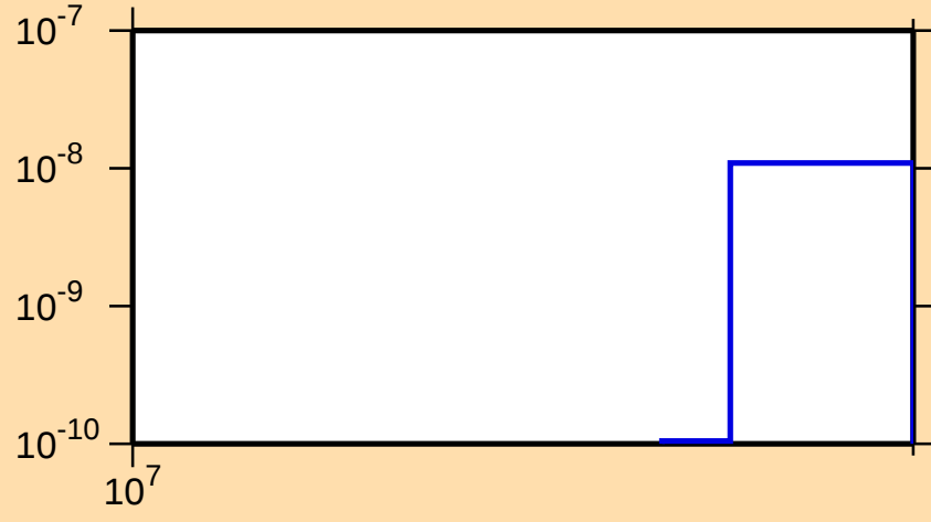
\sigma vs. E for ^{228}\text{Fr}(n,3n\alpha)
