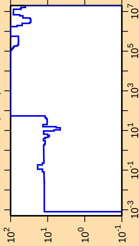
\Delta\sigma/\sigma vs. E for ^{228}\text{Fr}(n,\text{el.})
