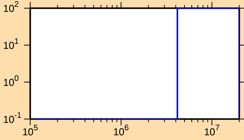
\Delta\sigma/\sigma vs. E for ^{228}\text{Fr}(n,\text{f})
