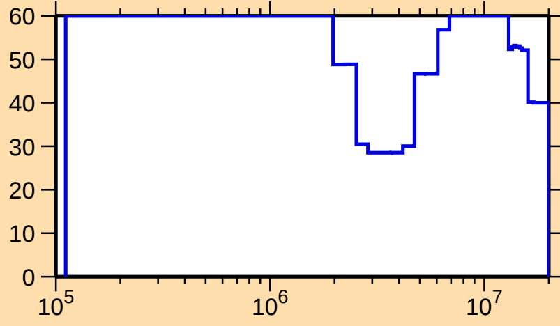
\Delta\sigma/\sigma vs. E for ^{228}\text{Fr}(n,\text{el.})
