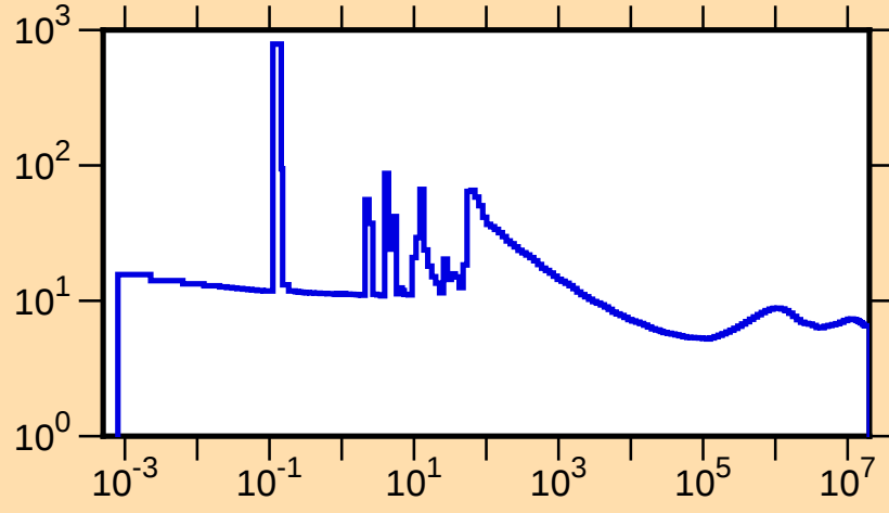
\sigma vs. E for ^{228}\text{Fr}(n,\text{tot.})
