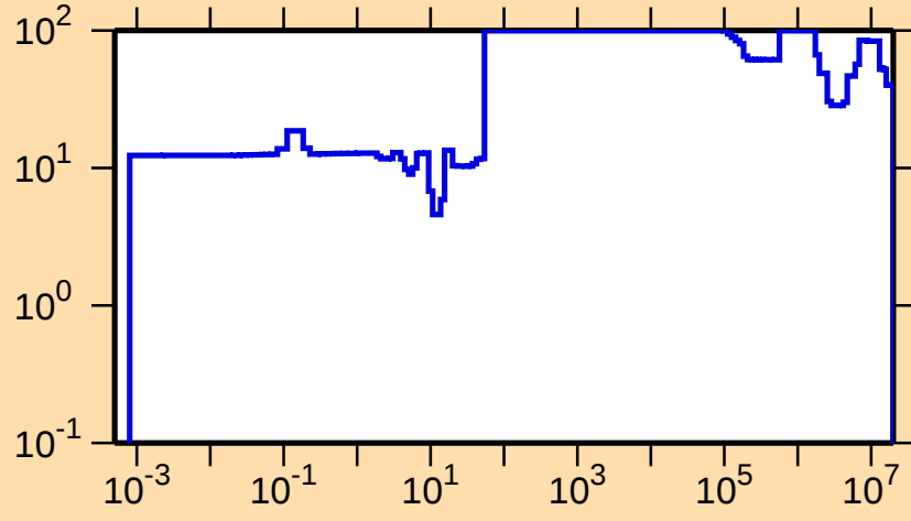
\Delta\sigma/\sigma vs. E for ^{228}\text{Fr}(n,\text{el.})
