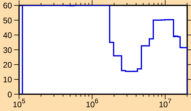
\Delta\sigma/\sigma vs. E for ^{228}\text{Fr}(n,\text{tot.})
