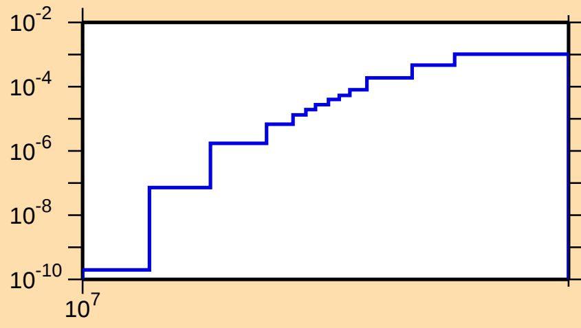
\sigma vs. E for ^{228}\text{Fr}(n,3n)
