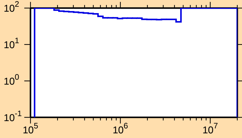
\Delta\sigma/\sigma vs. E for ^{228}\text{Fr}(n,\text{inel.})
