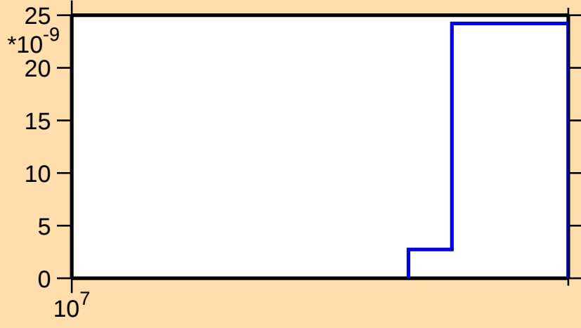
\sigma vs. E for ^{228}\text{Fr}(n,\text{He3})
