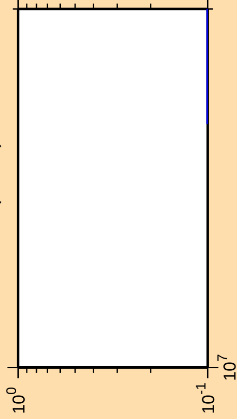
\Delta\sigma/\sigma vs. E for ^{228}\text{Fr}(\text{mt 11})
