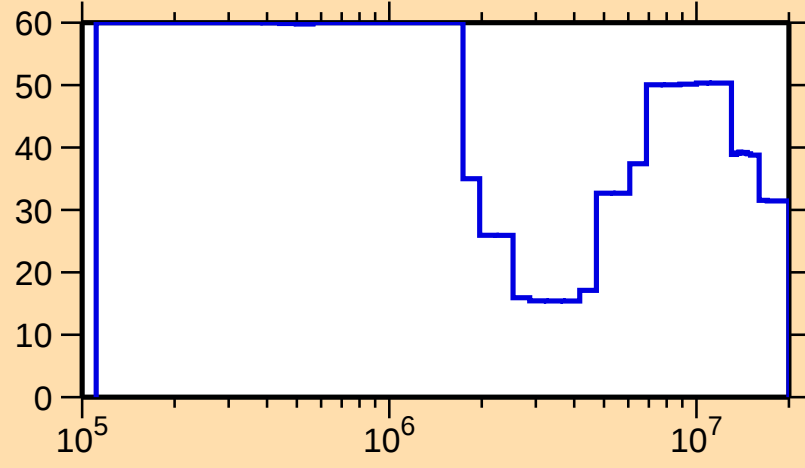
\Delta\sigma/\sigma vs. E for ^{228}\text{Fr}(n,\text{tot.})
