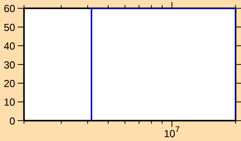
\Delta\sigma/\sigma vs. E for ^{228}\text{Fr}(n,2n)
