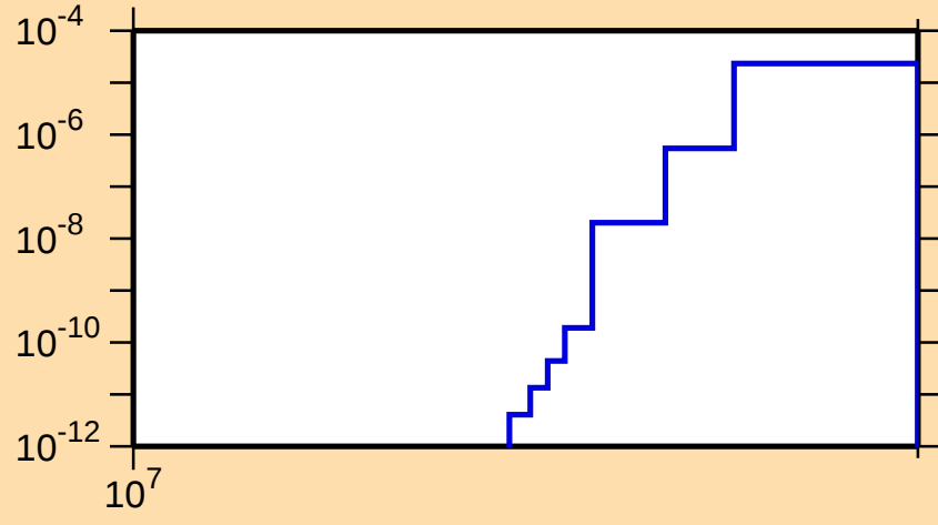
\sigma vs. E for ^{228}\text{Fr}(n,2np)
