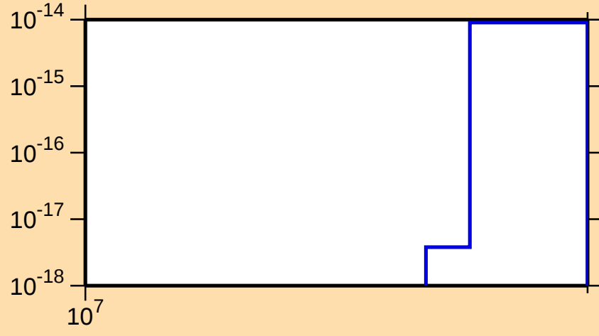
\sigma vs. E for ^{228}\text{Fr}(\text{mt 11})
