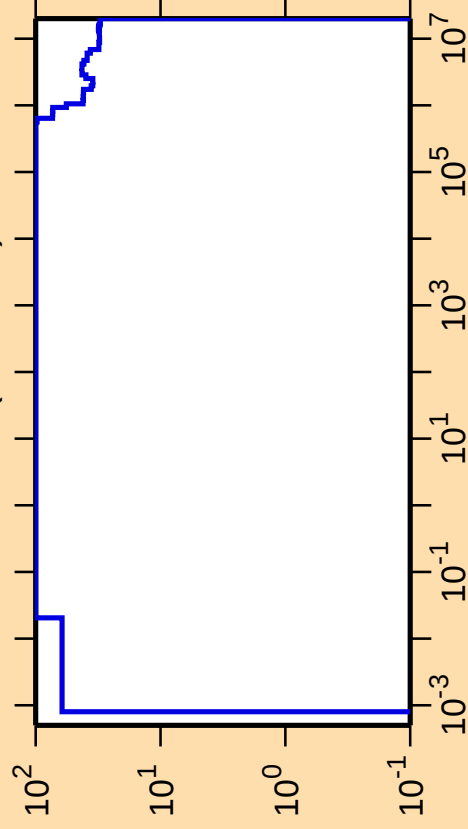
\Delta\sigma/\sigma vs. E for ^{228}\text{Fr}(n,\text{nonel.})
