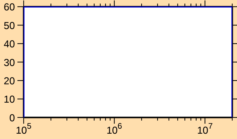
\Delta\sigma/\sigma vs. E for ^{228}\text{Fr}(n,n_1)
