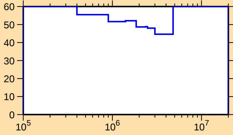
\Delta\sigma/\sigma vs. E for ^{228}\text{Fr}(n,\text{inel.})
