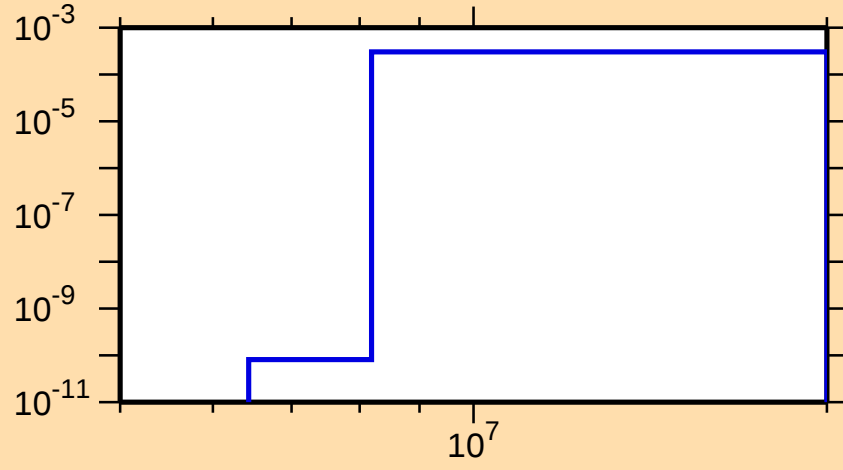
\sigma vs. E for ^{228}\text{Fr}(n,n\alpha)
