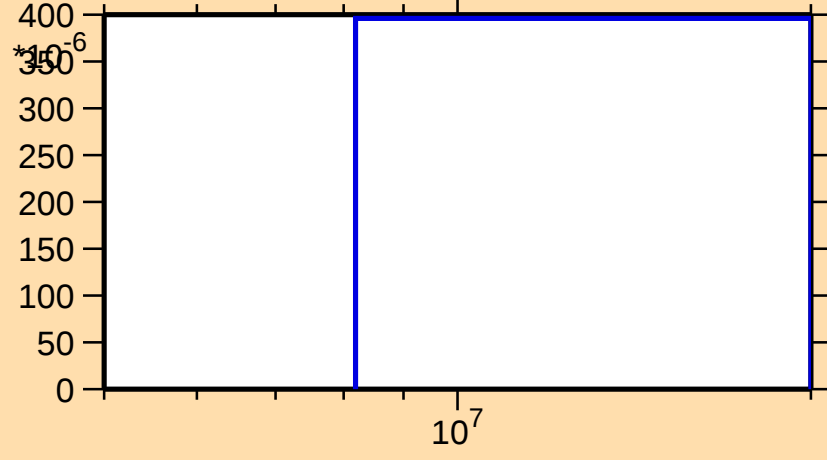
\sigma vs. E for ^{228}\text{Fr}(n,np)
