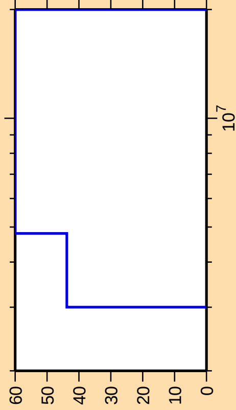
\Delta\sigma/\sigma vs. E for ^{228}\text{Fr}(n,n\text{cont.})
