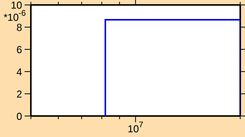
\sigma vs. E for ^{228}\text{Fr}(n,2n\alpha)
