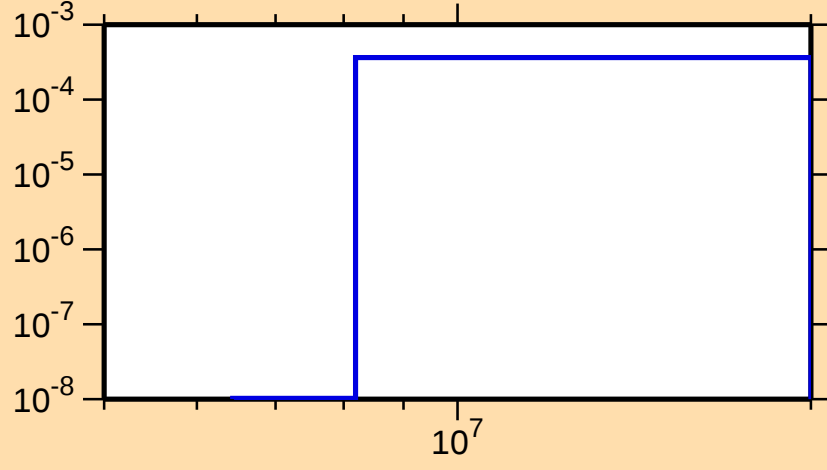
\sigma vs. E for ^{228}\text{Fr}(n,t)
