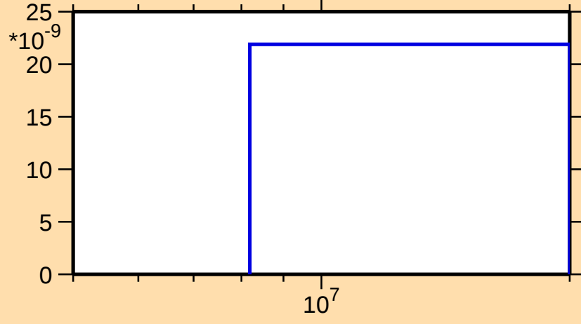
\sigma vs. E for ^{228}\text{Fr}(n,nt)
