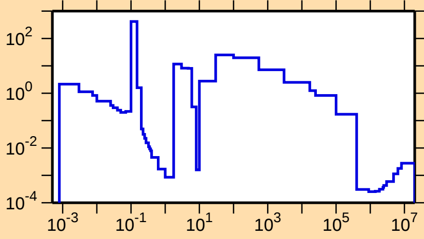
\sigma vs. E for ^{228}\text{Fr}(n,\gamma)
