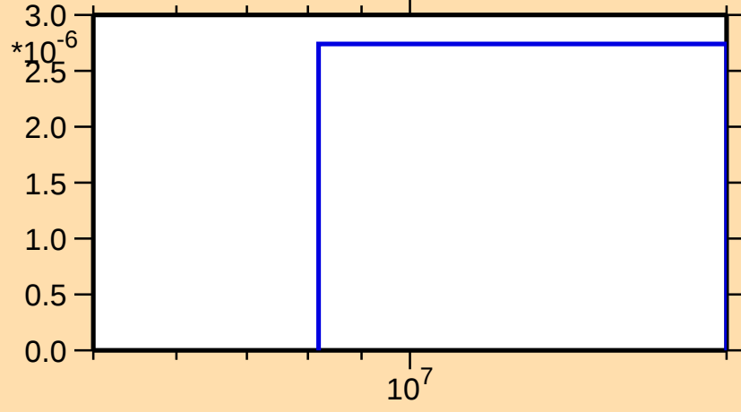
\sigma vs. E for ^{228}\text{Fr}(n,\text{nd})
