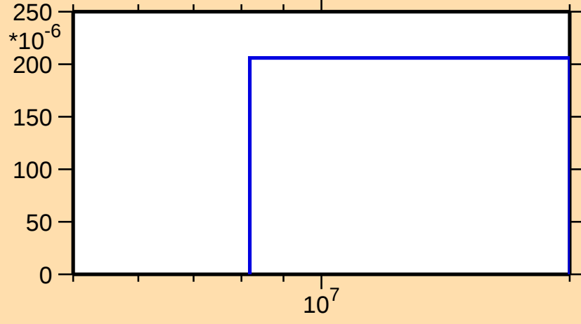
\sigma vs. E for ^{228}\text{Fr}(n,d)
