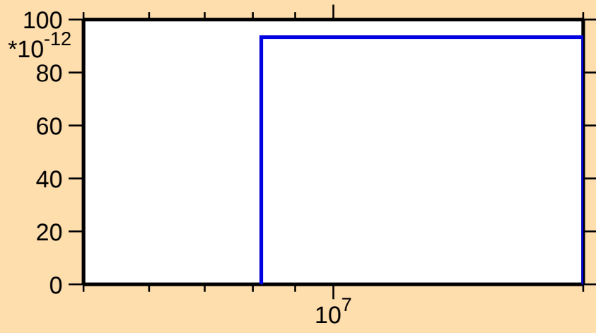
\sigma vs. E for ^{228}\text{Fr}(n,3n\alpha)
