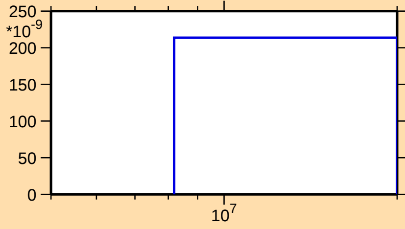
\sigma vs. E for ^{228}\text{Fr}(n,2np)
