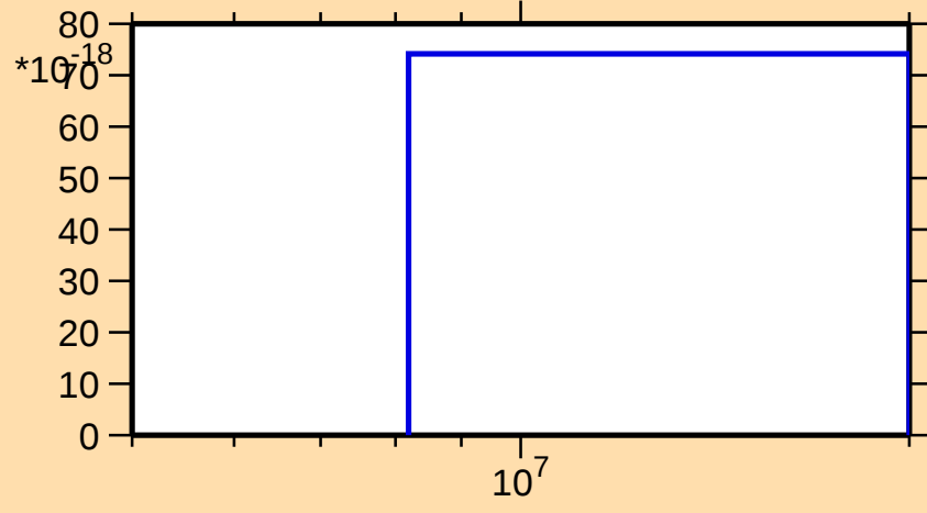
\sigma vs. E for ^{228}\text{Fr}(\text{mt } 11)
