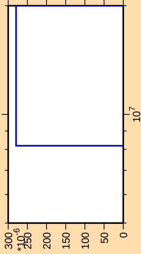
\Delta\sigma/\sigma vs. E for ^{228}\text{Fr}(\text{mt } 11)
