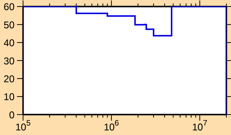
\Delta\sigma/\sigma vs. E for ^{228}\text{Fr}(n,n\text{cont.})
