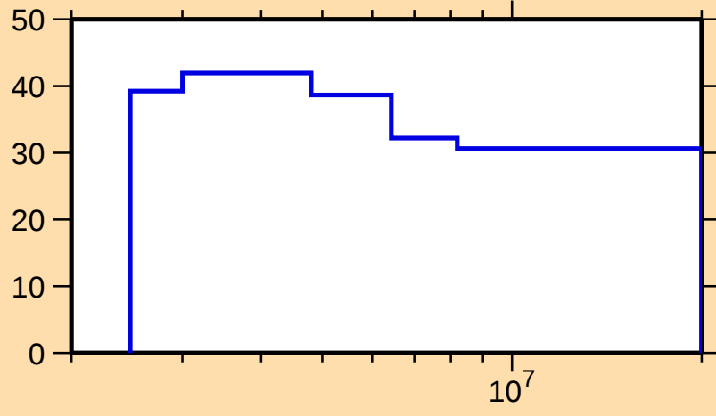
\Delta\sigma/\sigma vs. E for ^{228}\text{Fr}(n,\text{nonel.})
