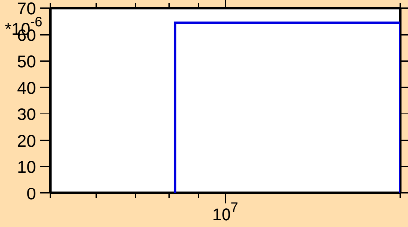
\sigma vs. E for ^{228}\text{Fr}(n,3n)
