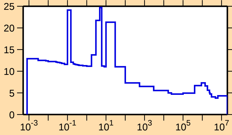
\sigma vs. E for ^{228}\text{Fr}(n,\text{el.})
