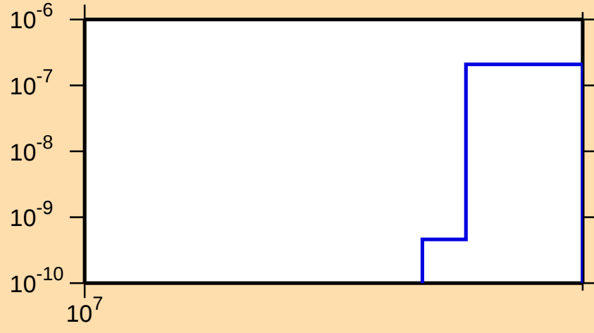
\sigma vs. E for ^{231}\text{Fr}(n,2np)
