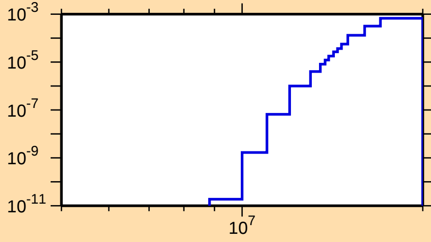
\sigma vs. E for ^{231}\text{Fr}(n,t)
