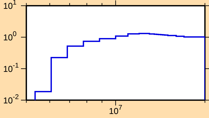
\sigma vs. E for ^{231}\text{Fr}(n,2n)
