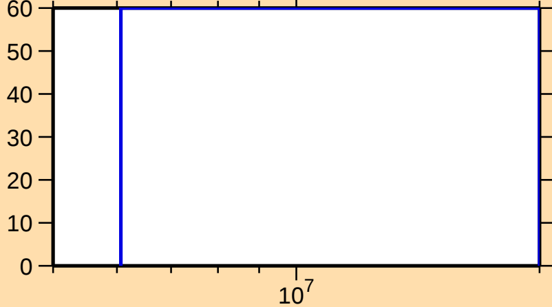
\Delta\sigma/\sigma vs. E for ^{231}\text{Fr}(n,\gamma)
