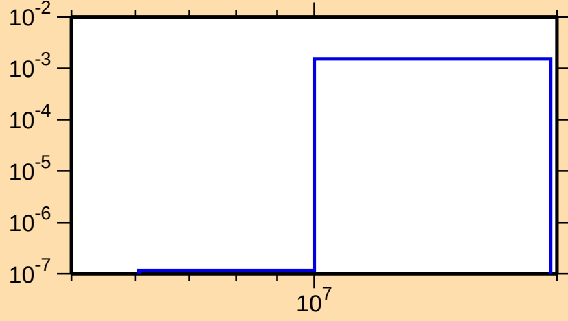
\sigma vs. E for ^{231}\text{Fr}(n,p)
