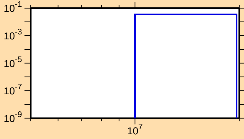
\sigma vs. E for ^{231}\text{Fr}(n,3n)
