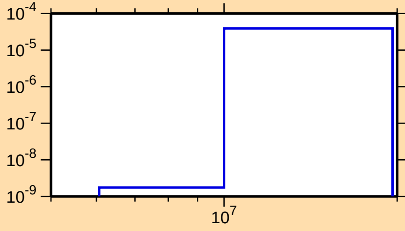
\sigma vs. E for ^{231}\text{Fr}(n,\alpha)
