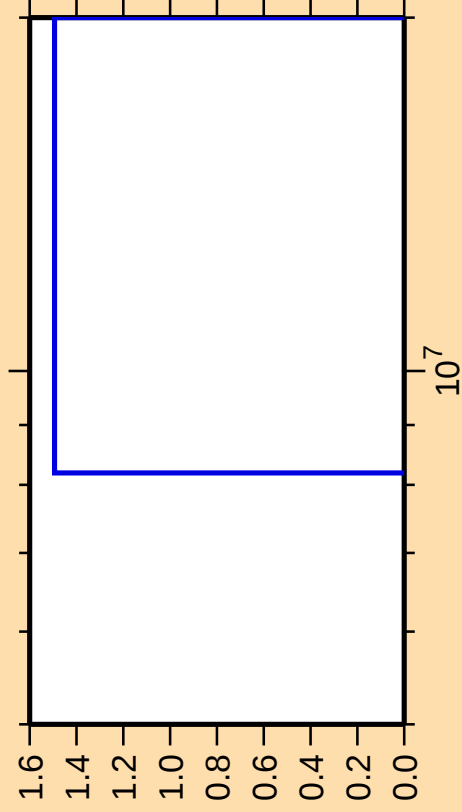
\Delta\sigma/\sigma vs. E for ^{231}\text{Fr}(n,3n\alpha)
