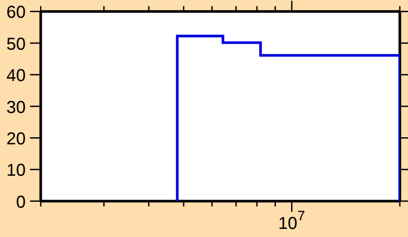
\Delta\sigma/\sigma vs. E for ^{231}\text{Fr}(n,\text{nonel.})
