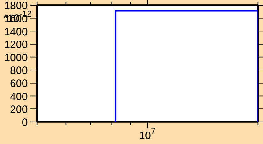
\sigma vs. E for ^{231}\text{Fr}(n,2np)
