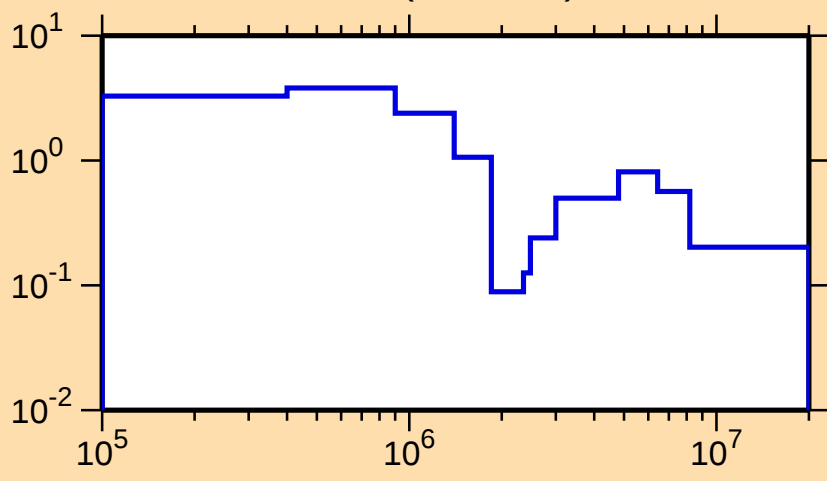
\sigma vs. E for ^{231}\text{Fr}(n,n\text{cont.})
