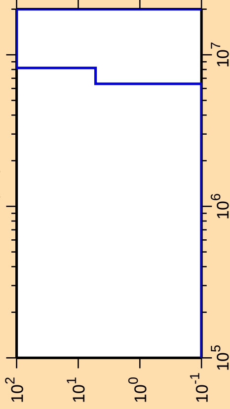
\Delta\sigma/\sigma vs. E for ^{231}\text{Fr}(n,f)
