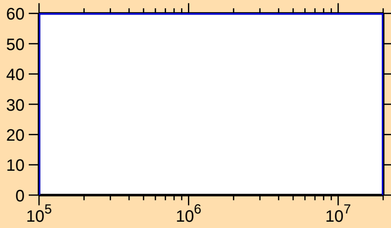
\Delta\sigma/\sigma vs. E for ^{231}\text{Fr}(n,n_1)
