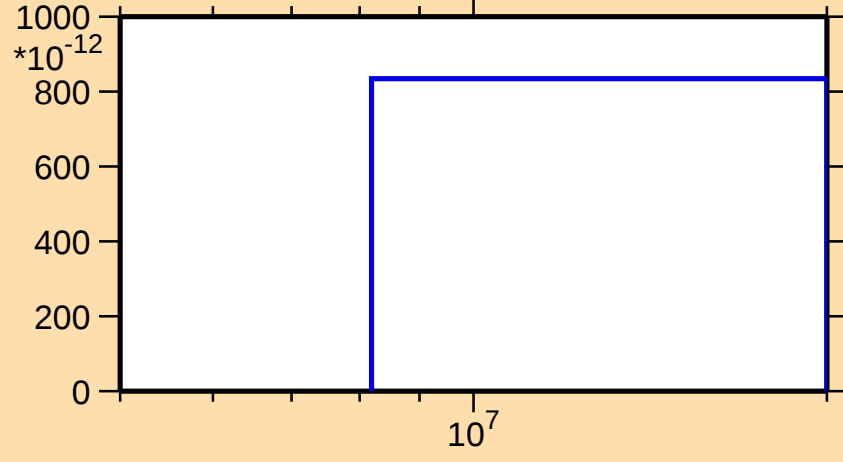
\sigma vs. E for ^{231}\text{Fr}(n,2n\alpha)
