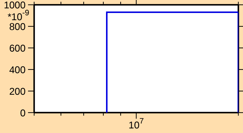
\sigma vs. E for ^{231}\text{Fr}(n,nt)
