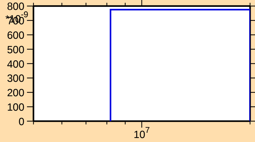
\sigma vs. E for ^{231}\text{Fr}(n,n\alpha)
