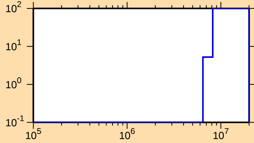
\Delta\sigma/\sigma vs. E for ^{231}\text{Fr}(n,\text{f})
