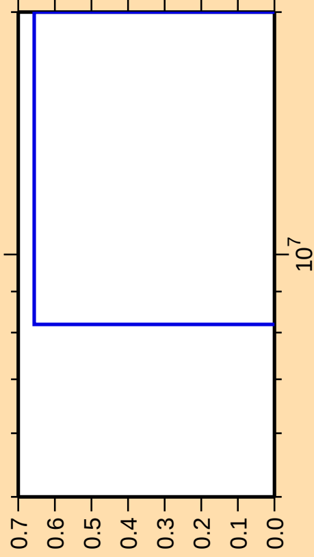
\Delta\sigma/\sigma vs. E for ^{231}\text{Fr}(\text{mt } 11)
