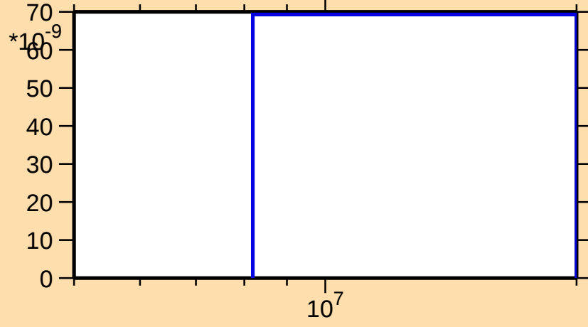
\sigma vs. E for ^{231}\text{Fr}(n,\text{nd})
