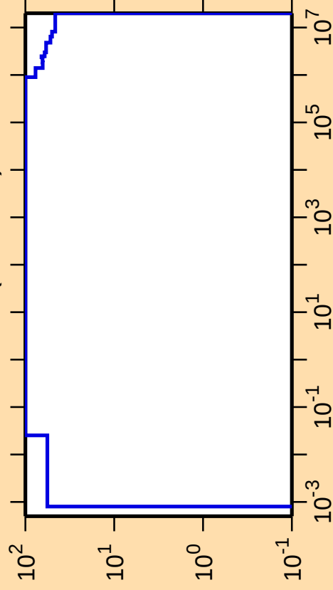
\Delta\sigma/\sigma vs. E for ^{231}\text{Fr}(n,\text{nonel.})
