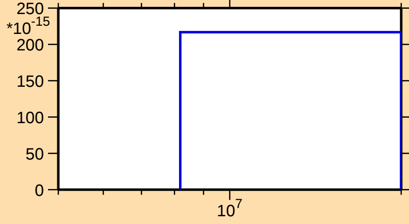
\sigma vs. E for ^{231}\text{Fr}(n,3n\alpha)
