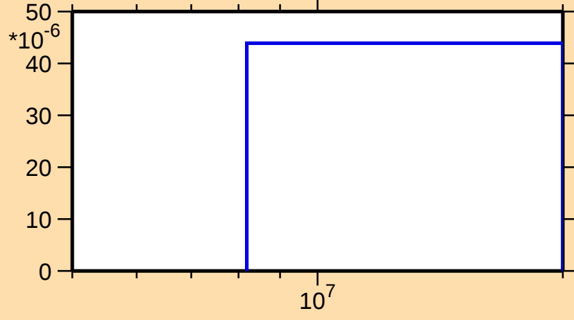
\sigma vs. E for ^{231}\text{Fr}(n,t)
