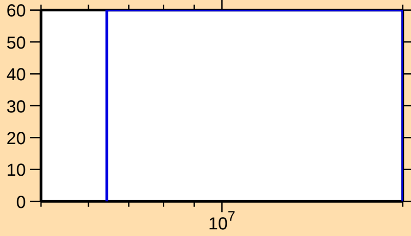
\Delta\sigma/\sigma vs. E for ^{231}\text{Fr}(n,n_1)
