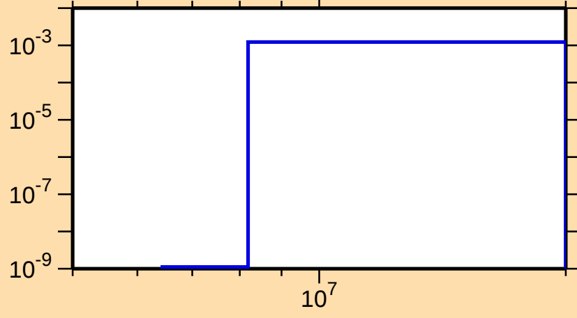
\sigma vs. E for ^{231}\text{Fr}(n,p)
