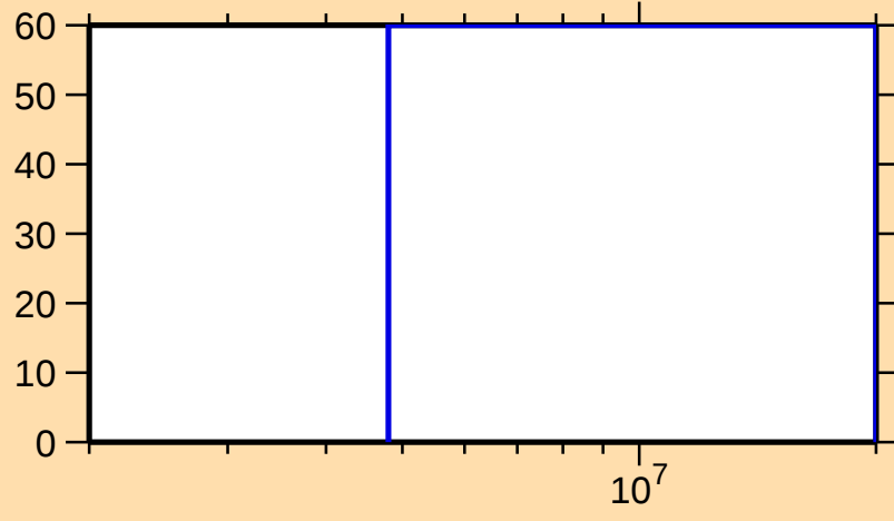
\Delta\sigma/\sigma vs. E for ^{231}\text{Fr}(n,\text{el.})
