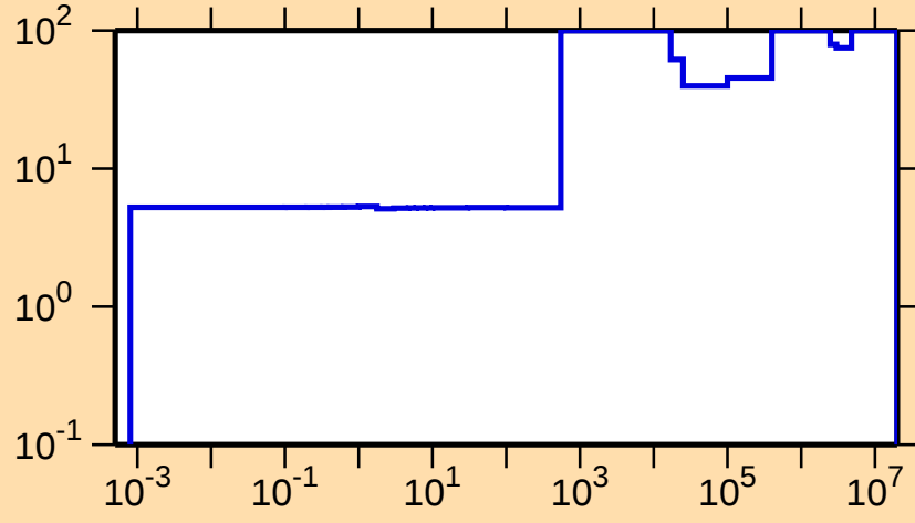
\Delta\sigma/\sigma vs. E for ^{231}\text{Fr}(n,\text{el.})
