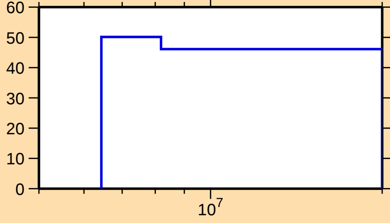
\Delta\sigma/\sigma vs. E for ^{231}\text{Fr}(n,\text{nonel.})
