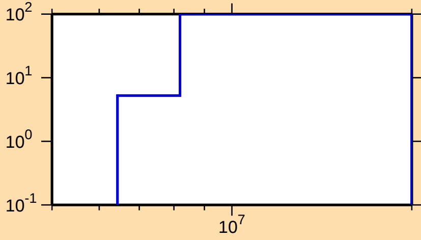
\Delta\sigma/\sigma vs. E for ^{231}\text{Fr}(n,f)
