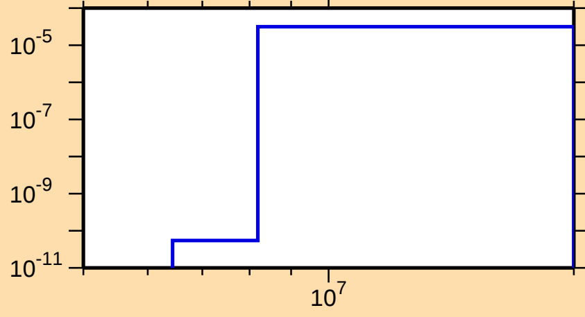
\sigma vs. E for ^{231}\text{Fr}(n,\alpha)
