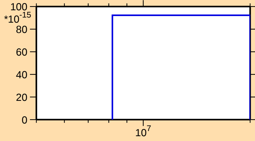
\sigma vs. E for ^{231}\text{Fr}(\text{mt } 11)
