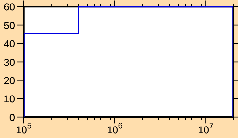
\Delta\sigma/\sigma vs. E for ^{231}\text{Fr}(\text{n,el.})
