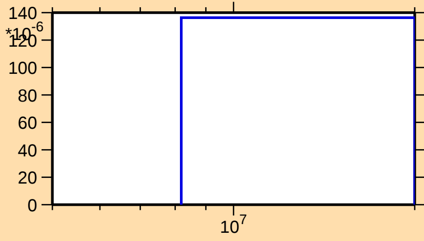
\sigma vs. E for ^{231}\text{Fr}(n,d)
