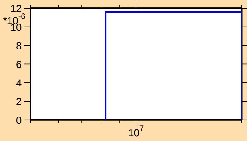
\sigma vs. E for ^{231}\text{Fr}(n,np)
