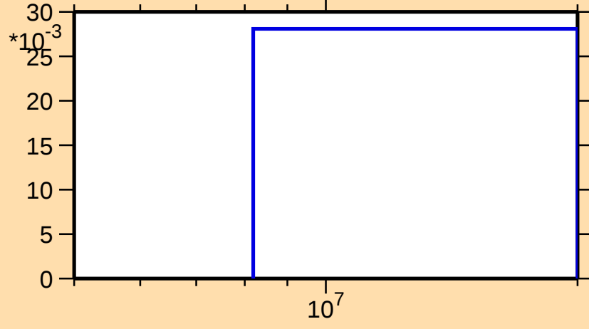
\sigma vs. E for ^{231}\text{Fr}(n,3n)
