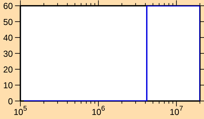
\Delta\sigma/\sigma vs. E for ^{232}\text{Fr}(n,f)
