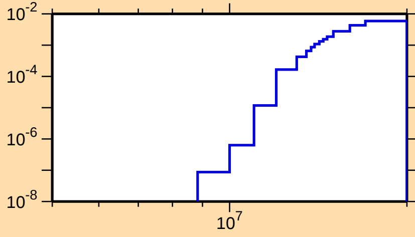
\sigma vs. E for ^{232}\text{Fr}(n,n\alpha)
