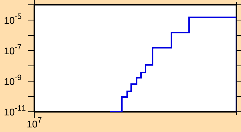
\sigma vs. E for ^{232}\text{Fr}(n,\text{nd})
