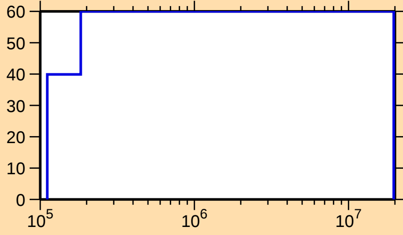
\Delta\sigma/\sigma vs. E for ^{232}\text{Fr}(\text{n,el.})
