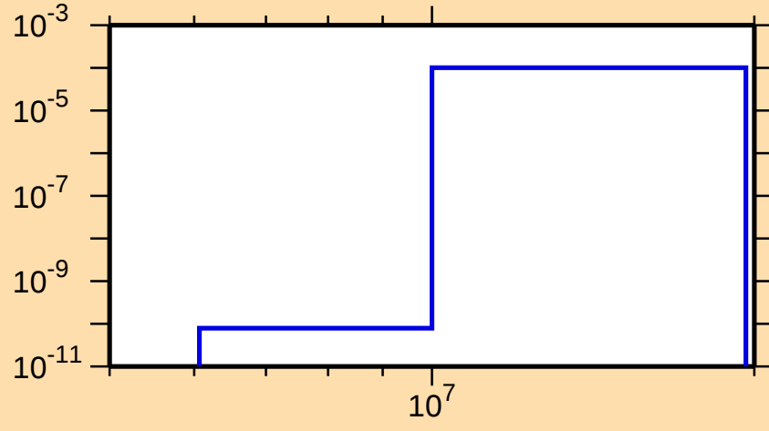
\sigma vs. E for ^{232}\text{Fr}(n,t)
