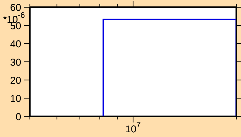
\sigma vs. E for ^{232}\text{Fr}(n,d)
