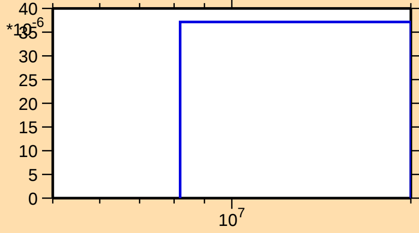
\sigma vs. E for ^{232}\text{Fr}(n,nt)
