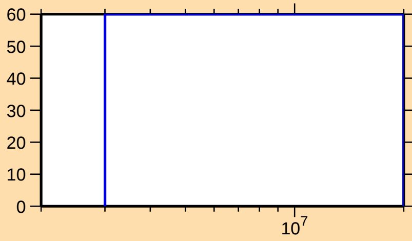
\Delta\sigma/\sigma vs. E for ^{232}\text{Fr}(n,\gamma)
