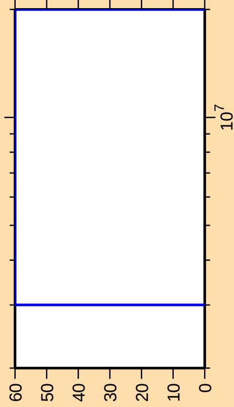
\Delta\sigma/\sigma vs. E for ^{232}\text{Fr}(n,\alpha)
