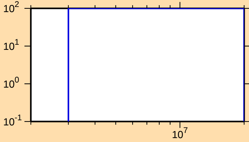
\Delta\sigma/\sigma vs. E for ^{232}\text{Fr}(n,n_1)
