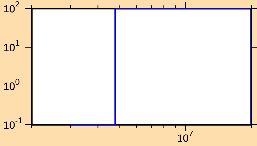
\Delta\sigma/\sigma vs. E for ^{232}\text{Fr}(n,p)
