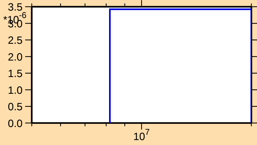
\sigma vs. E for ^{232}\text{Fr}(n,2n\alpha)
