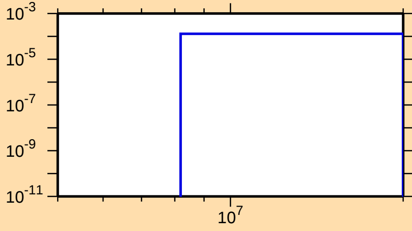
\sigma vs. E for ^{232}\text{Fr}(n,np)
