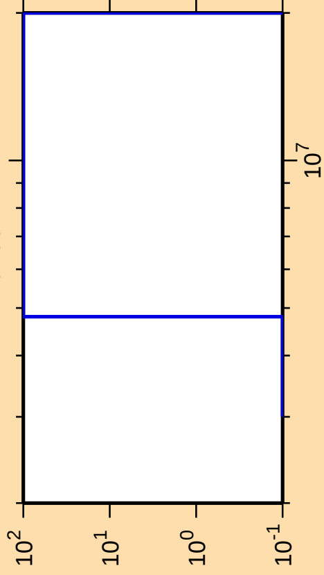
\Delta\sigma/\sigma vs. E for ^{232}\text{Fr}(n,p)
