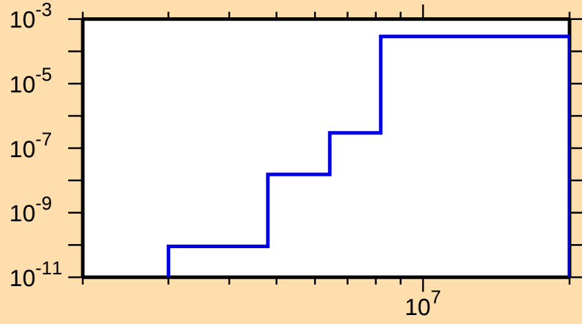
\sigma vs. E for ^{232}\text{Fr}(n,\alpha)
