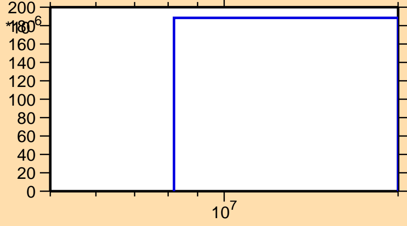
\sigma vs. E for ^{233}\text{Fr}(n,d)
