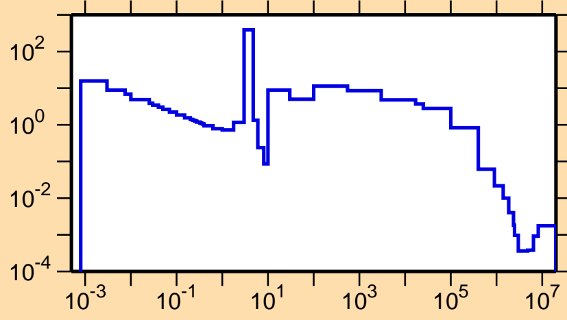
\sigma vs. E for ^{233}\text{Fr}(n,\gamma)
