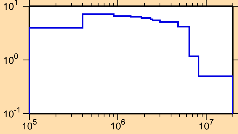
\sigma vs. E for ^{233}\text{Fr}(n,\text{inel.})
