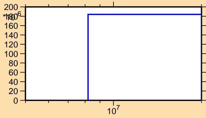
\sigma vs. E for ^{233}\text{Fr}(n,np)
