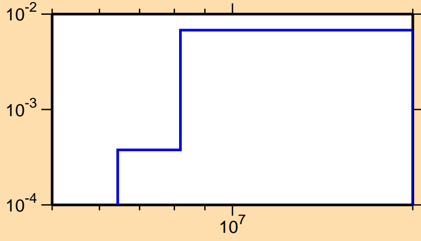
\sigma vs. E for ^{233}\text{Fr}(n,\alpha)
