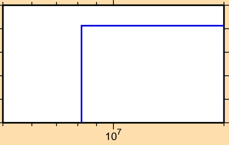
\sigma vs. E for ^{233}\text{Fr}(n,2n\alpha)
