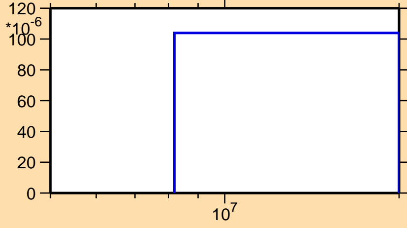
\sigma vs. E for ^{233}\text{Fr}(n,n\alpha)
