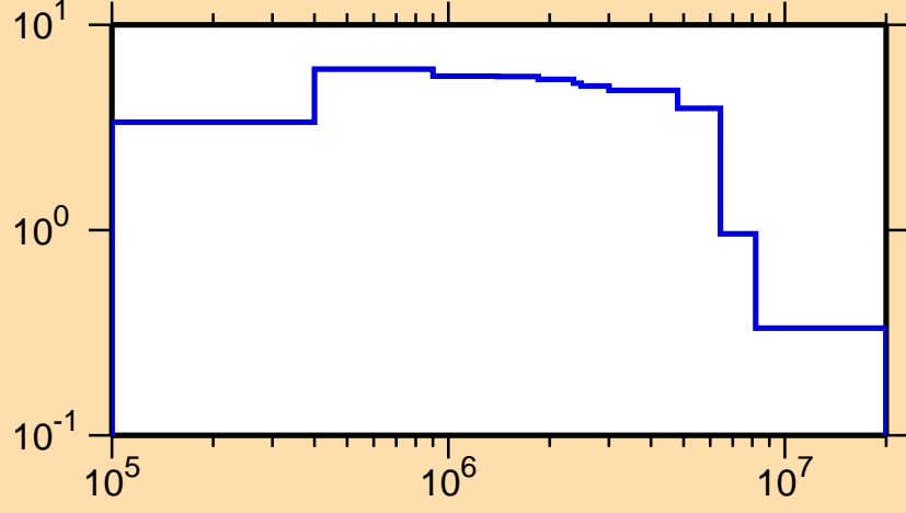
\sigma vs. E for ^{233}\text{Fr}(n,n\text{cont.})
