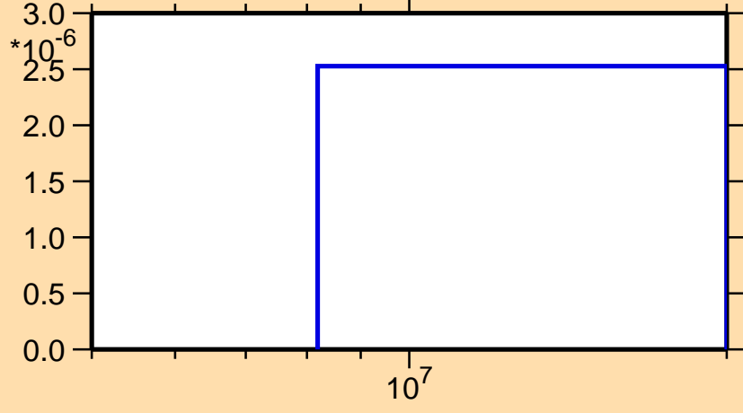
\sigma vs. E for ^{233}\text{Fr}(n,nt)
