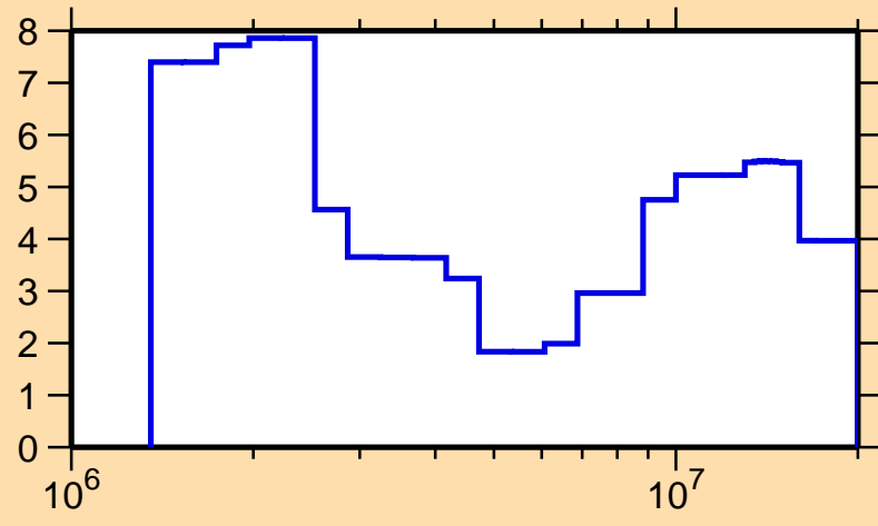
\Delta\sigma/\sigma vs. E for ^{63}\text{Ga}(n,\text{tot.})
