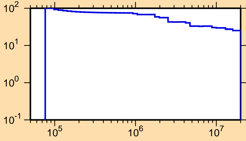
\Delta\sigma/\sigma vs. E for ^{63}\text{Ga}(n,n_1)
