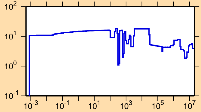
\Delta\sigma/\sigma vs. E for ^{63}\text{Ga}(n,\text{tot.})
