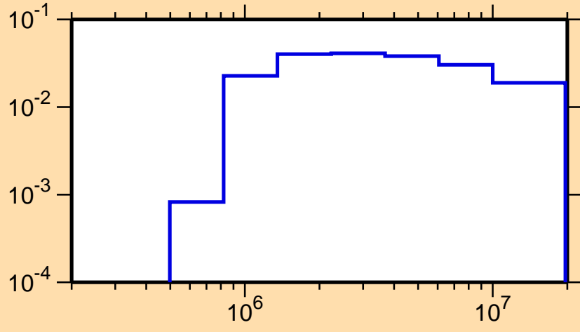
\sigma vs. E for ^{63}\text{Ga}(n,n_3)
