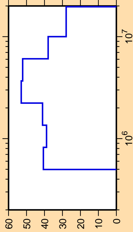
\Delta\sigma/\sigma vs. E for ^{63}\text{Ga}(n,n_3)
