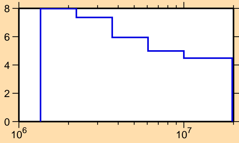
\Delta\sigma/\sigma vs. E for ^{63}\text{Ga}(n,n\text{onel.})
