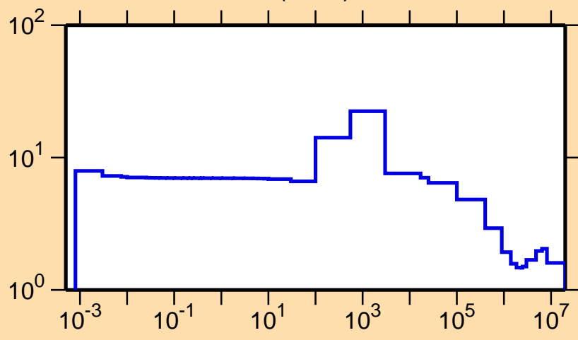
\sigma vs. E for ^{63}\text{Ga}(n,\text{el.})
