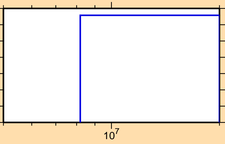
\sigma vs. E for ^{63}\text{Ga}(n,\text{nd})
