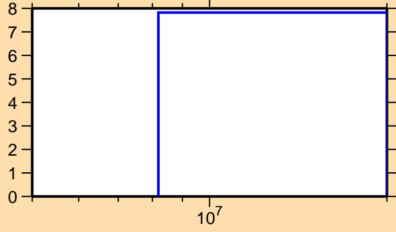
\Delta\sigma/\sigma vs. E for ^{63}\text{Ga}(n,\text{el.})
