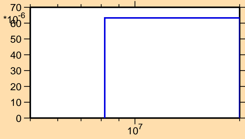
\sigma vs. E for ^{63}\text{Ga} (mt 45)
