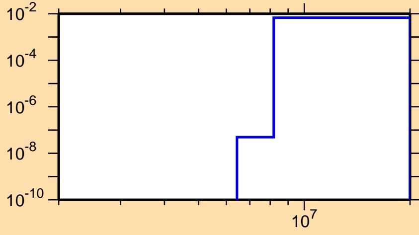
\sigma vs. E for ^{63}\text{Ga}(n,n\alpha)
