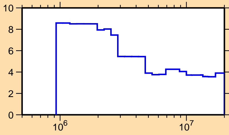
\Delta\sigma/\sigma vs. E for ^{64}\text{Ga}(n,\text{nonel.})
