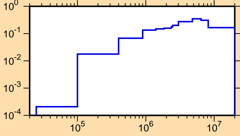
\sigma vs. E for ^{64}\text{Ga}(n,\text{inel.})
