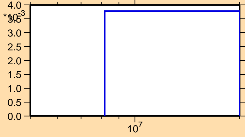
\sigma vs. E for ^{64}\text{Ga}(n,2n)
