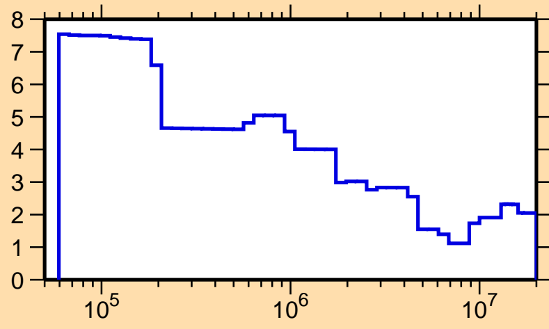
\Delta\sigma/\sigma vs. E for ^{65}\text{Ga}(n,\text{nonel.})
