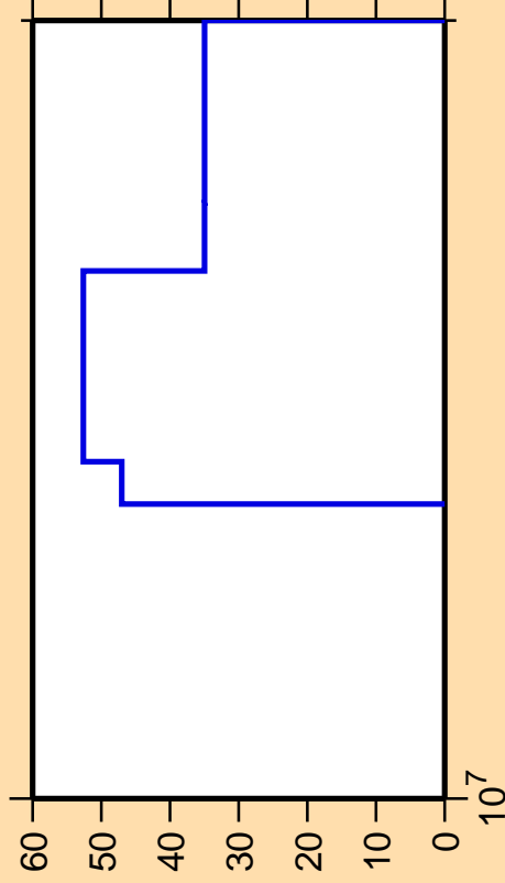
\Delta\sigma/\sigma vs. E for ^{65}\text{Ga} (mt 45)
