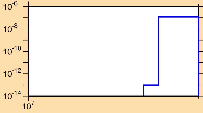
\sigma vs. E for ^{65}\text{Ga}(n,\text{pt})
