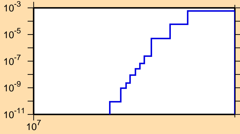
\sigma vs. E for ^{65}\text{Ga} (mt 45)
