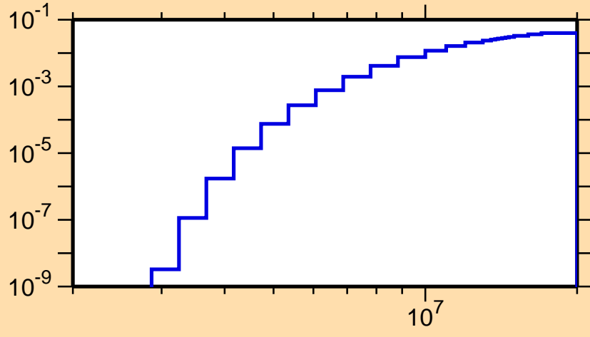
\sigma vs. E for ^{65}\text{Ga}(n,d)
