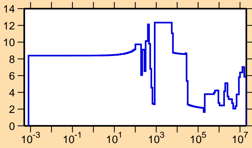
\Delta\sigma/\sigma vs. E for ^{65}\text{Ga}(n,\text{el.})
