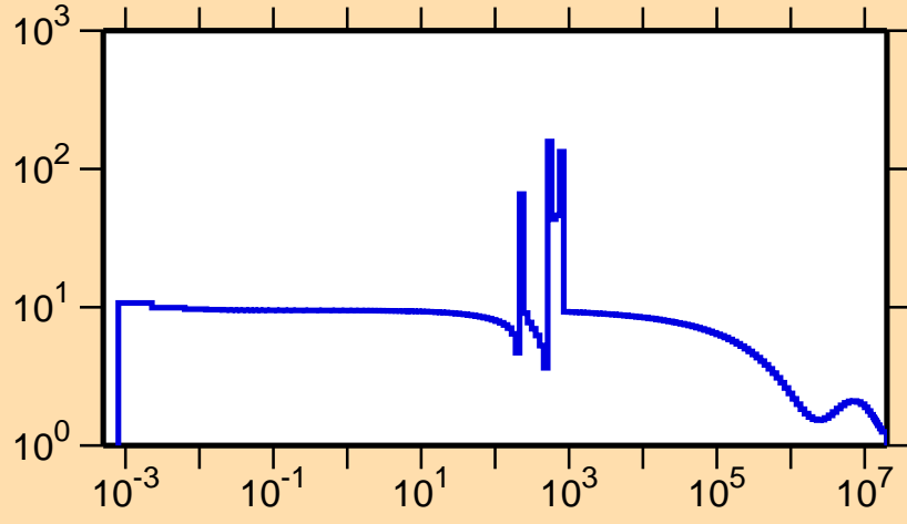
\sigma vs. E for ^{65}\text{Ga}(n,\text{el.})
