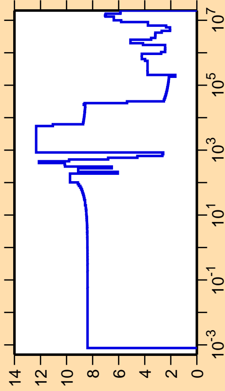
\Delta\sigma/\sigma vs. E for ^{65}\text{Ga}(n,\text{el.})
