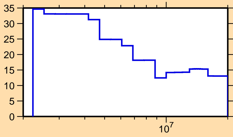
\Delta\sigma/\sigma vs. E for ^{65}\text{Ga}(n,ncont.)
