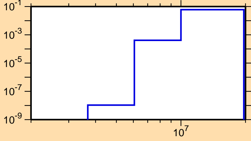
\sigma vs. E for ^{65}\text{Ga}(n,p\alpha)
