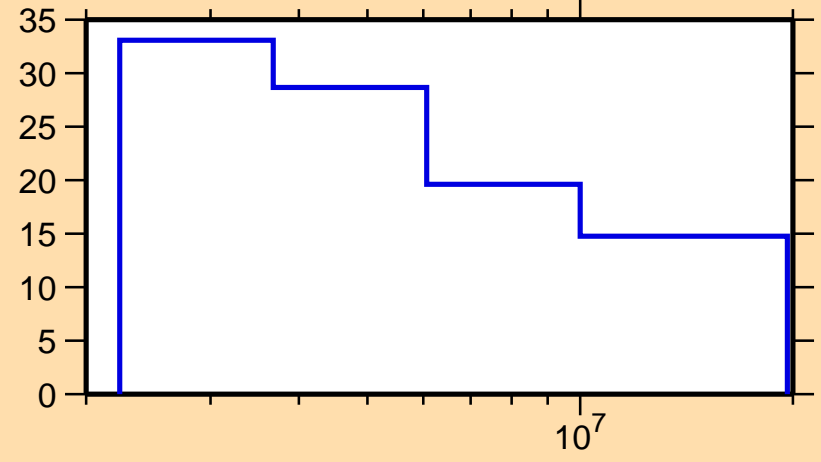
\Delta\sigma/\sigma vs. E for ^{65}\text{Ga}(n,n\text{cont.})
