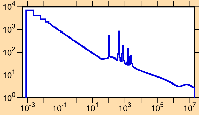
\sigma vs. E for ^{66}\text{Ga}(n,\text{tot.})
