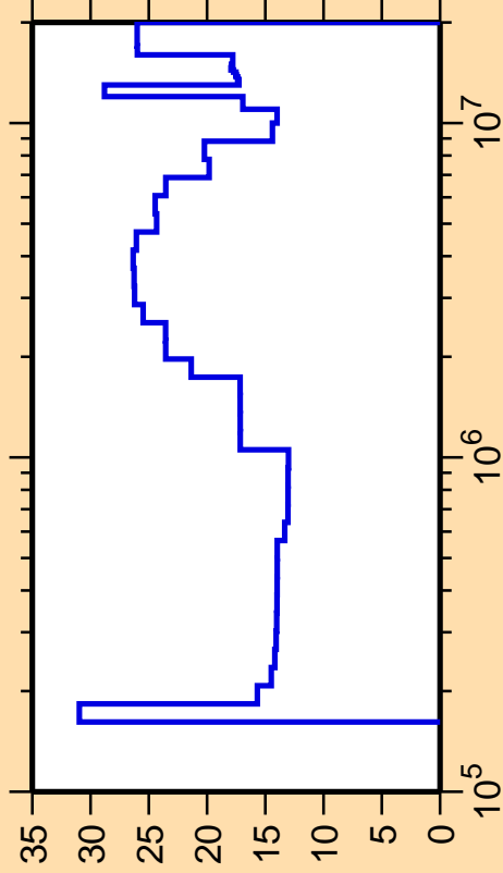
\Delta\sigma/\sigma vs. E for ^{66}\text{Ga}(n,n_4)
