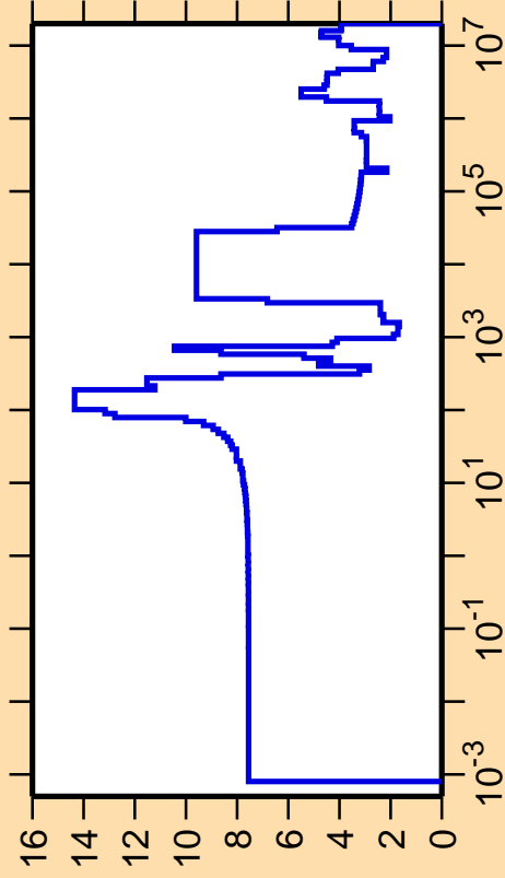
\Delta\sigma/\sigma vs. E for ^{66}\text{Ga}(n,\text{el.})
