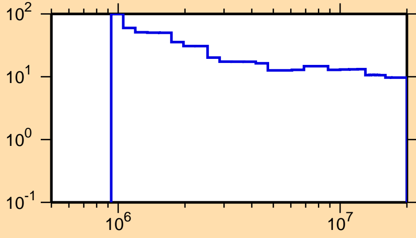
\Delta\sigma/\sigma vs. E for ^{66}\text{Ga}(n,n\text{cont.})
