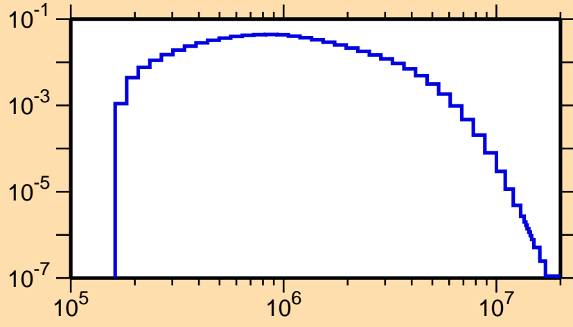
\sigma vs. E for ^{66}\text{Ga}(n,n_4)
