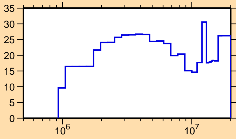
\Delta\sigma/\sigma vs. E for ^{66}\text{Ga}(n,n_1)
