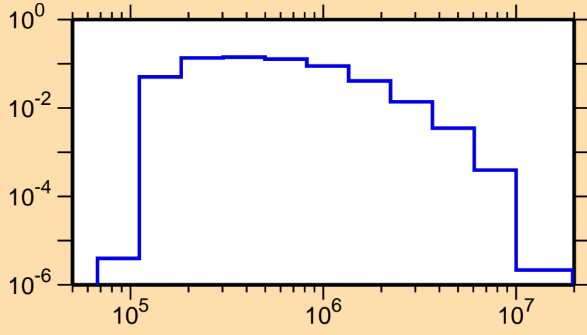
\sigma vs. E for ^{66}\text{Ga}(n,n_3)
