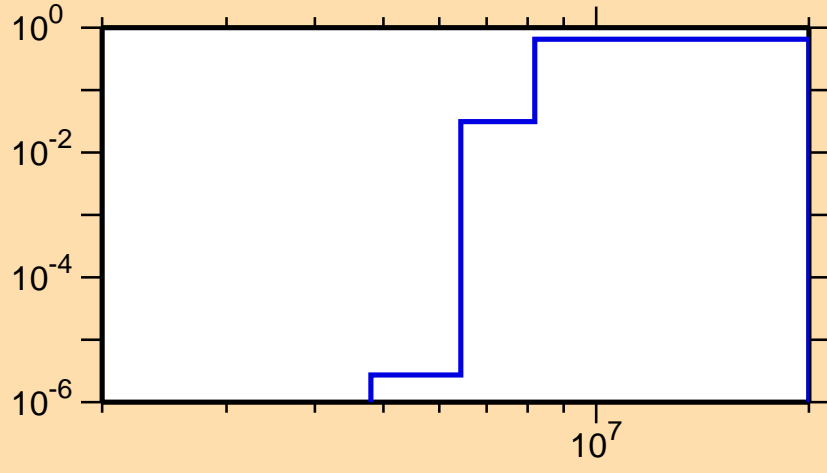
\sigma vs. E for ^{66}\text{Ga}(n,np)
