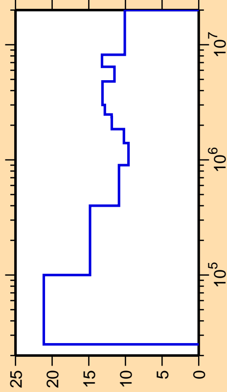
\Delta\sigma/\sigma vs. E for ^{66}\text{Ga}(n,\text{inel.})
