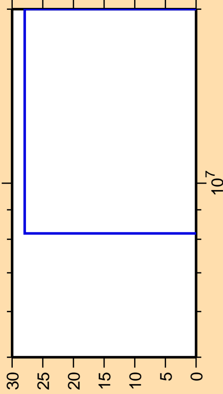
\Delta\sigma/\sigma vs. E for ^{66}\text{Ga}(n,2n)
