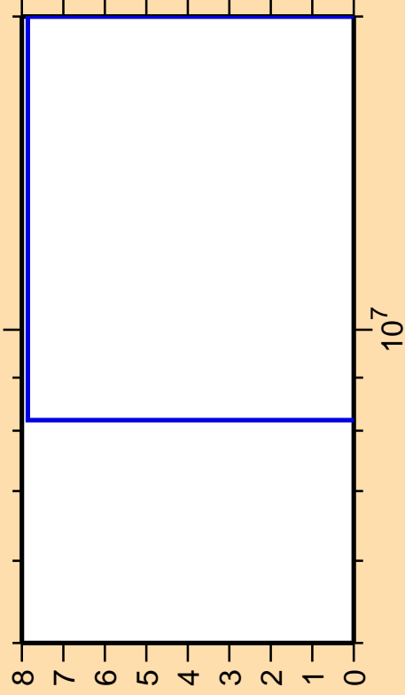
\Delta\sigma/\sigma vs. E for ^{66}\text{Ga}(n,p)
