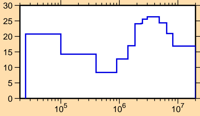
\Delta\sigma/\sigma vs. E for ^{66}\text{Ga}(n,n_1)
