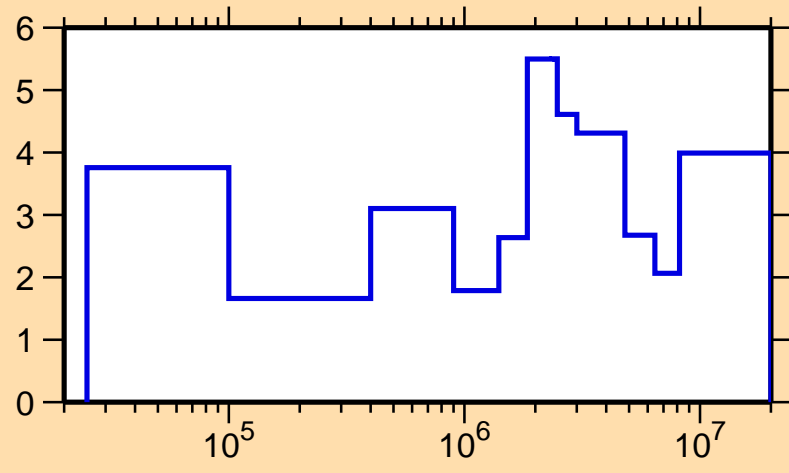
\Delta\sigma/\sigma vs. E for ^{66}\text{Ga}(n,\text{el.})
