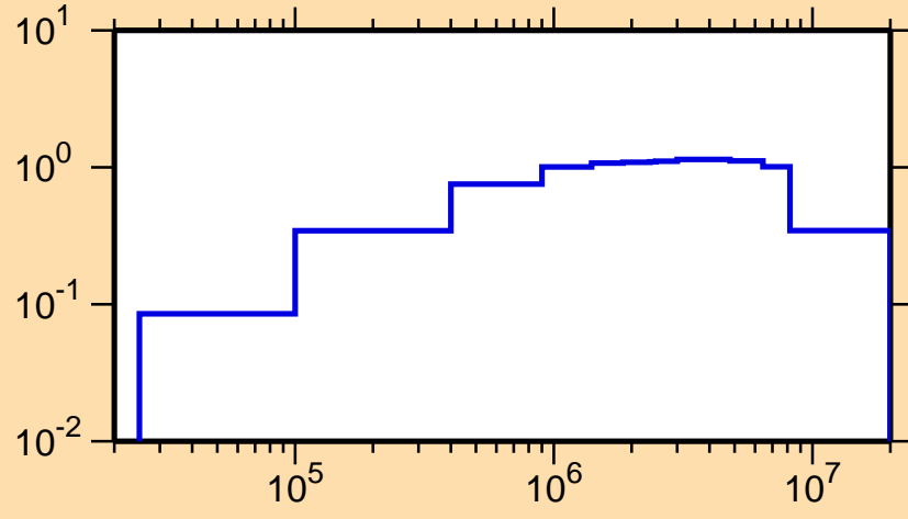
\sigma vs. E for ^{66}\text{Ga}(n,\text{inel.})
