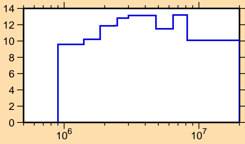
\Delta\sigma/\sigma vs. E for ^{66}\text{Ga}(n,\text{inel.})
