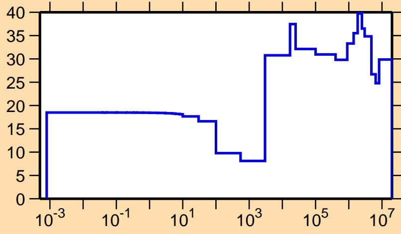
\Delta\sigma/\sigma vs. E for ^{66}\text{Ga}(n,\gamma)
