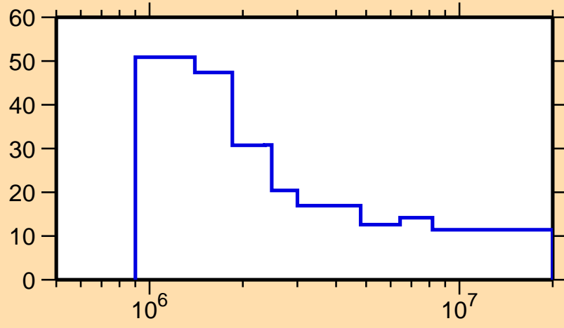
\Delta\sigma/\sigma vs. E for ^{66}\text{Ga}(n,n\text{cont.})
