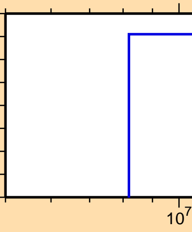
\sigma vs. E for ^{66}\text{Ga}(n,\text{He3})
