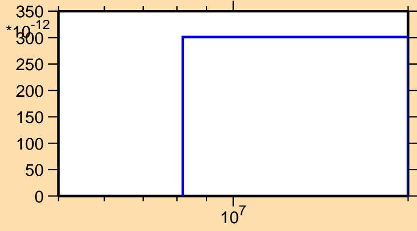
\sigma vs. E for ^{66}\text{Ga} (mt 34)
