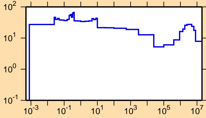
\Delta\sigma/\sigma vs. E for ^{66}\text{Ga}(n,p)
