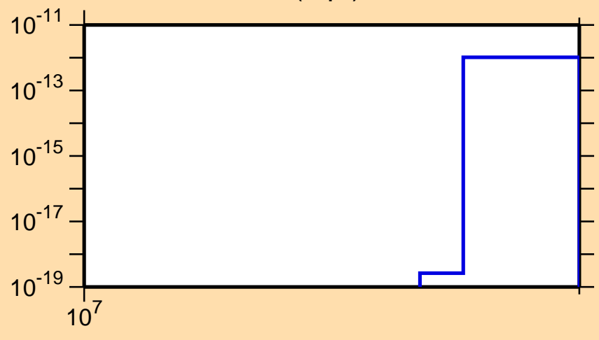
\sigma vs. E for ^{67}\text{Ga}(n,\text{pt})
