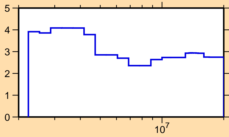
\Delta\sigma/\sigma vs. E for ^{67}\text{Ga}(n,n\text{inel.})
