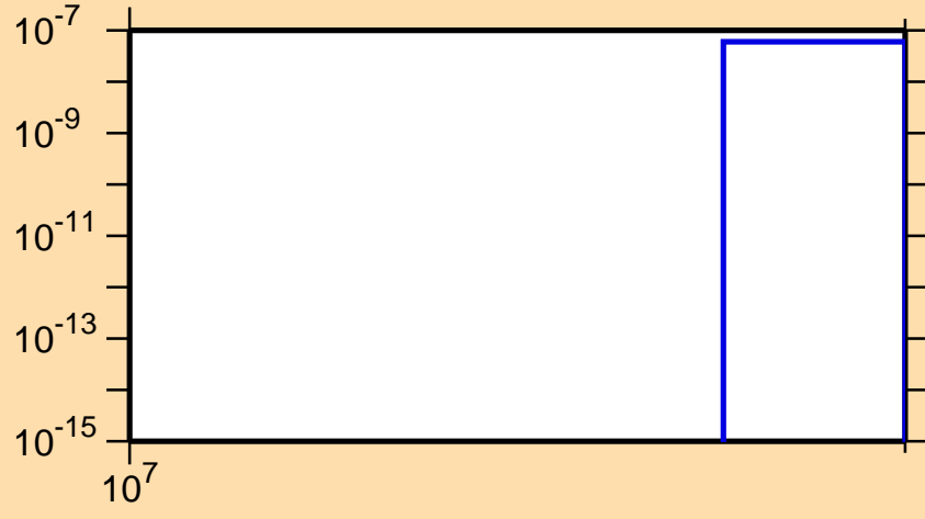
\sigma vs. E for ^{67}\text{Ga}(n,nt)
