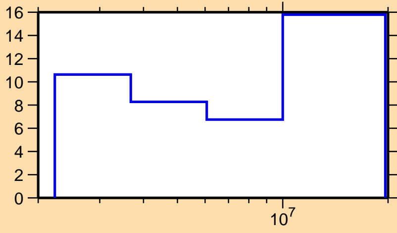
\Delta\sigma/\sigma vs. E for ^{67}\text{Ga}(n,ncont.)
