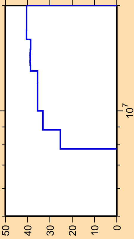
\Delta\sigma/\sigma vs. E for ^{68}\text{Ga}(n,\gamma)
