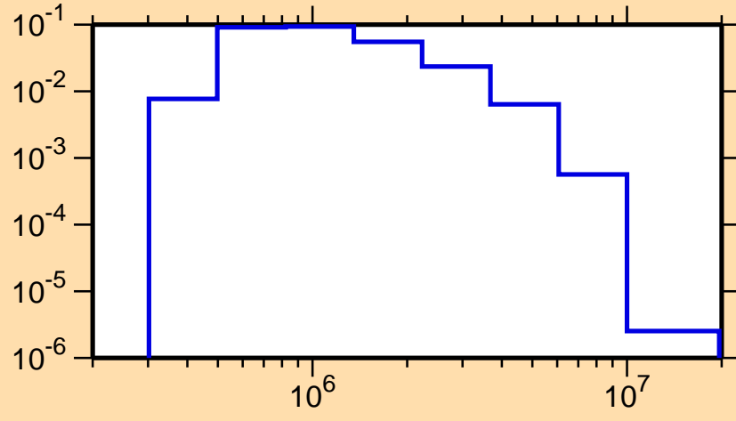
\sigma vs. E for ^{68}\text{Ga}(n,n_4)
