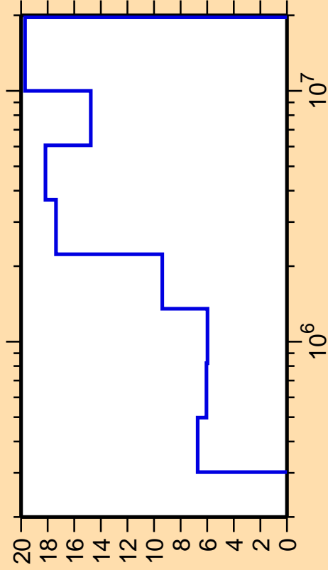
\Delta\sigma/\sigma vs. E for ^{68}\text{Ga}(n,n_4)
