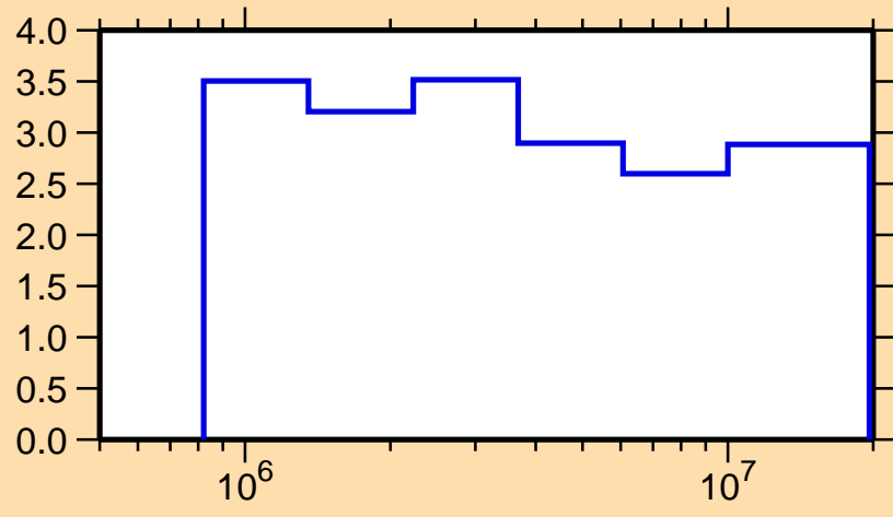
\Delta\sigma/\sigma vs. E for ^{68}\text{Ga}(n,n\text{onel.})
