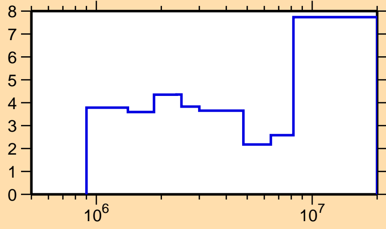
\Delta\sigma/\sigma vs. E for ^{68}\text{Ga}(n,\text{inel.})
