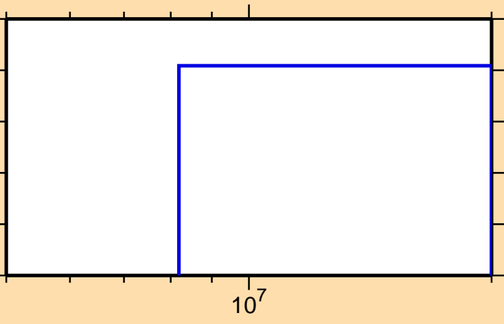
\sigma vs. E for ^{68}\text{Ga}(n,2np)
