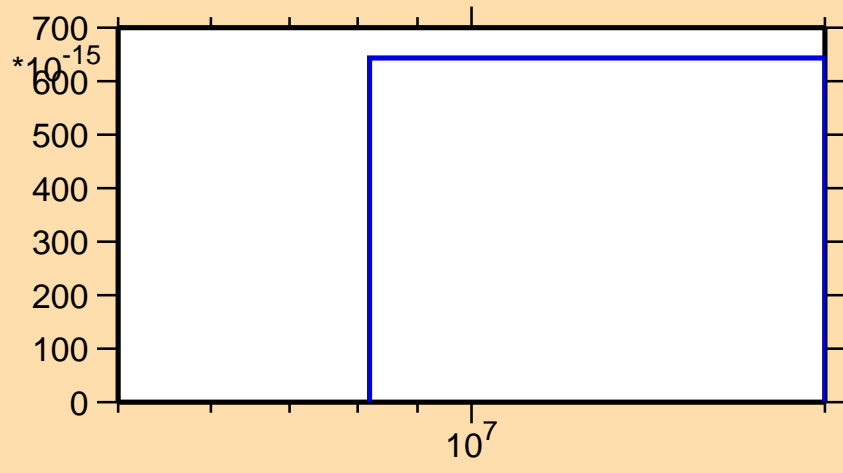
\sigma vs. E for ^{68}\text{Ga} (mt 34)
