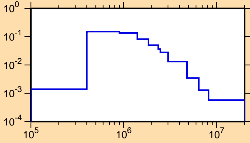
\sigma vs. E for ^{68}\text{Ga}(n,n_3)
