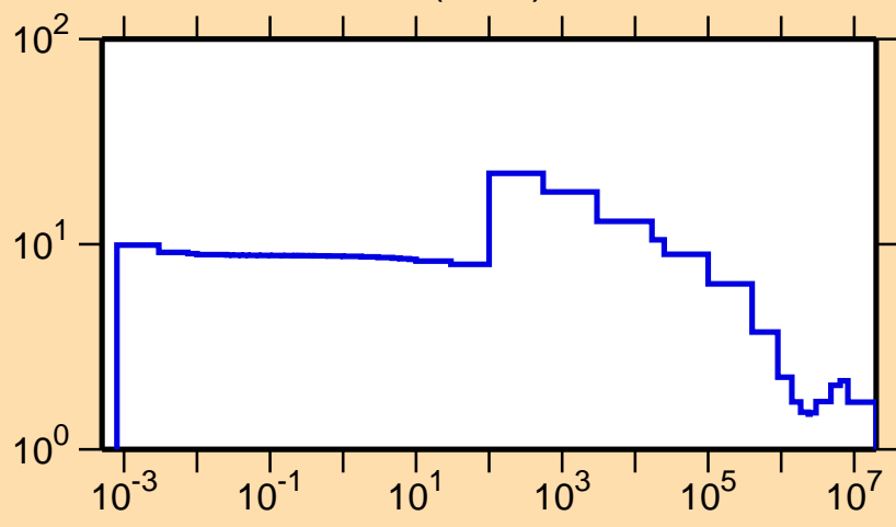
\sigma vs. E for ^{68}\text{Ga}(n,\text{el.})
