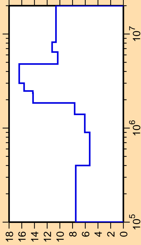
\Delta\sigma/\sigma vs. E for ^{68}\text{Ga}(n,n_3)
