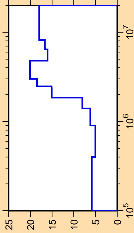
\Delta\sigma/\sigma vs. E for ^{68}\text{Ga}(n,n_2)
