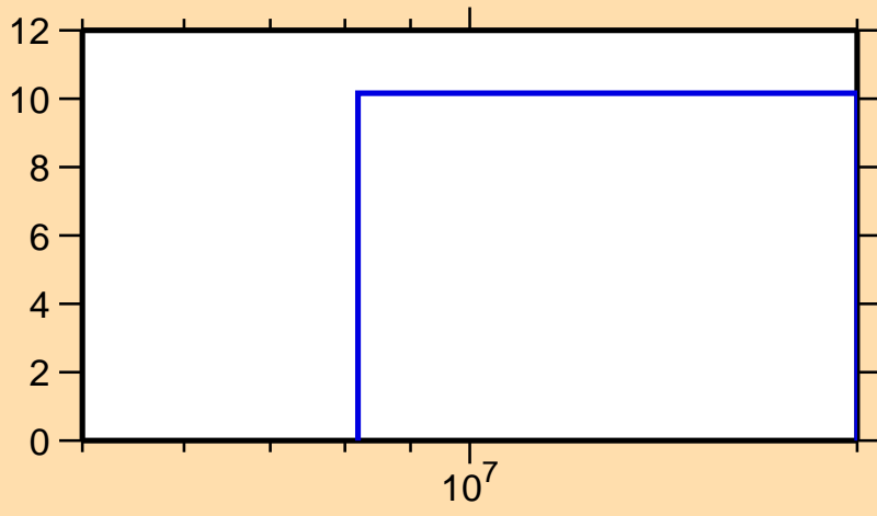
\Delta\sigma/\sigma vs. E for ^{68}\text{Ga}(n,2n)
