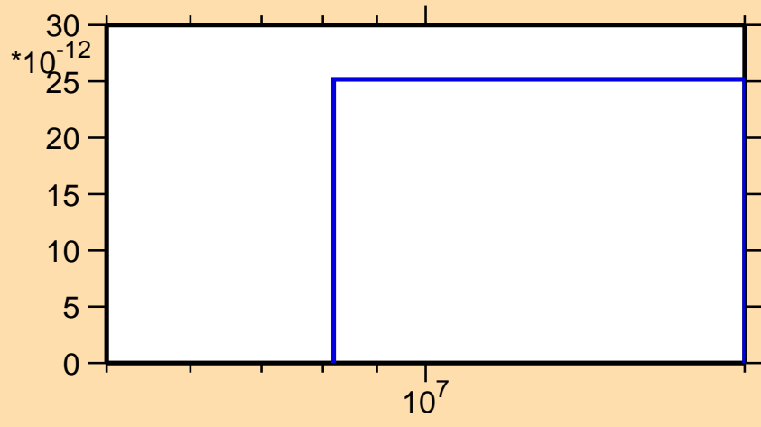
\sigma vs. E for ^{68}\text{Ga} (mt 45)
