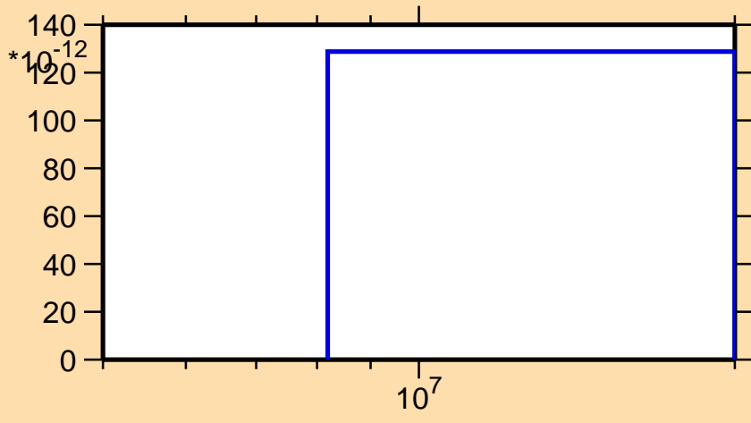
\sigma vs. E for ^{68}\text{Ga}(\text{mt117})
