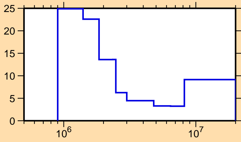
\Delta\sigma/\sigma vs. E for ^{68}\text{Ga}(n,n\text{cont.})
