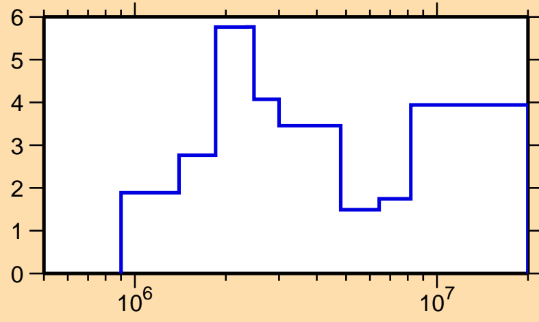
\Delta\sigma/\sigma vs. E for ^{68}\text{Ga}(n,\text{el.})
