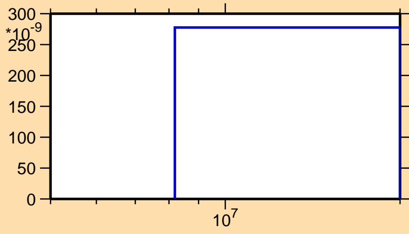
\sigma vs. E for ^{68}\text{Ga}(n,2n\alpha)
