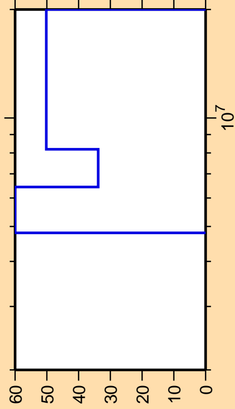
\Delta\sigma/\sigma vs. E for ^{68}\text{Ga}(n,d)
