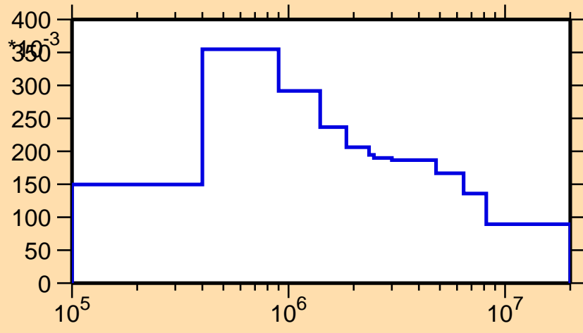
\sigma vs. E for ^{68}\text{Ga}(n,n_1)
