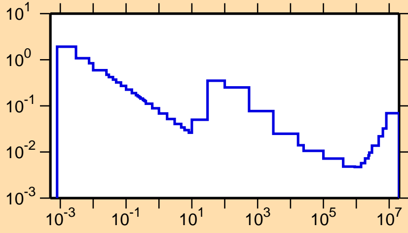
\sigma vs. E for ^{68}\text{Ga}(n,\alpha)
