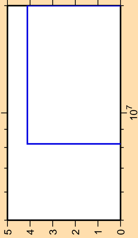
\Delta\sigma/\sigma vs. E for ^{68}\text{Ga}(n,3n)
