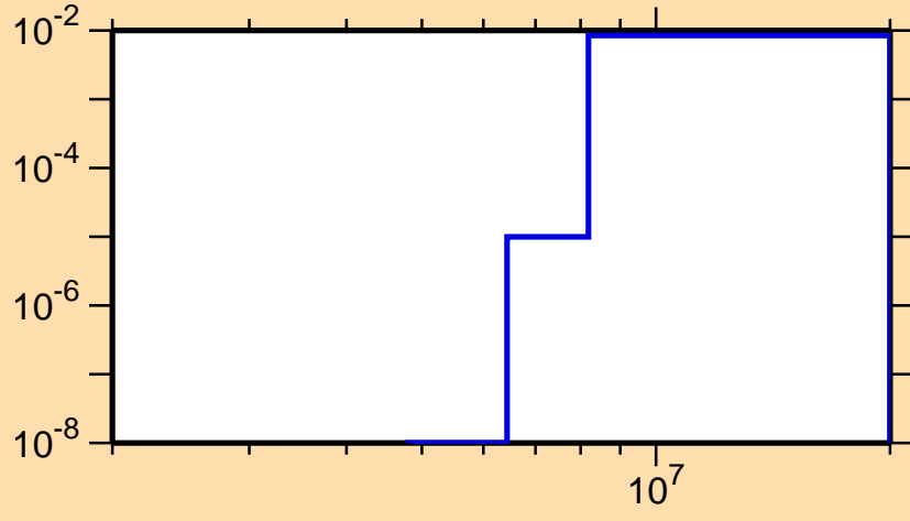
\sigma vs. E for ^{68}\text{Ga}(n,d)
