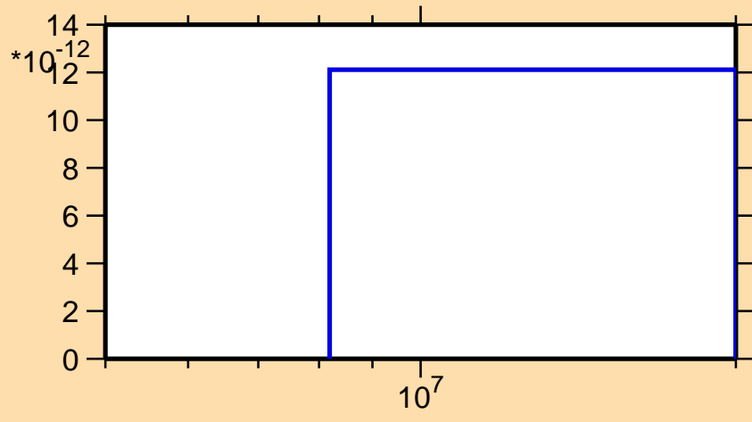
\sigma vs. E for ^{68}\text{Ga}(n,3n)
