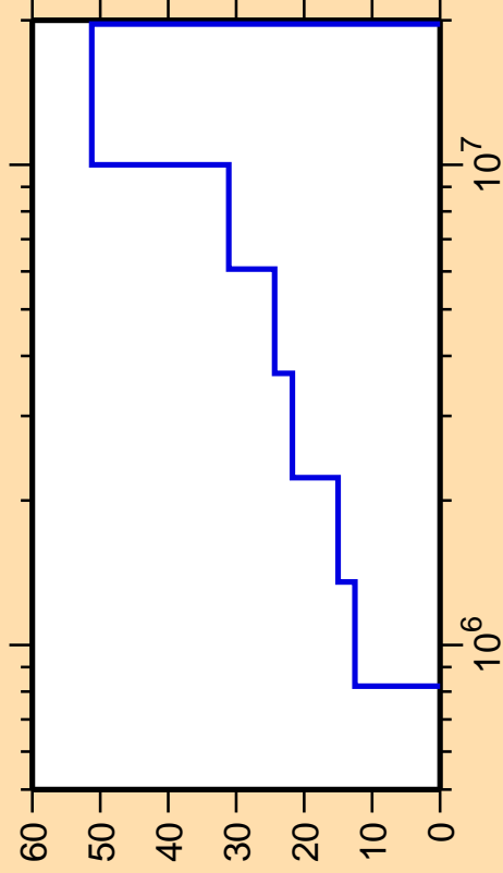
\Delta\sigma/\sigma vs. E for ^{70}\text{Ga}(n,n_4)
