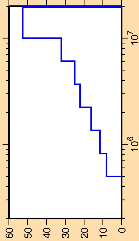
\Delta\sigma/\sigma vs. E for ^{70}\text{Ga}(n,n_3)
