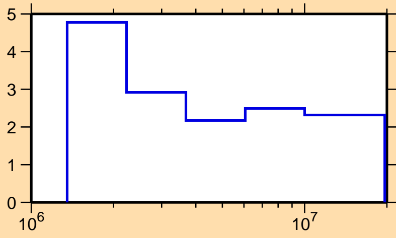
\Delta\sigma/\sigma vs. E for ^{70}\text{Ga}(n,n\text{nonel.})
