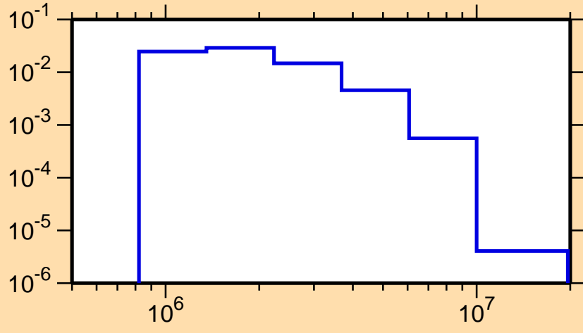
\sigma vs. E for ^{70}\text{Ga}(n,n_4)
