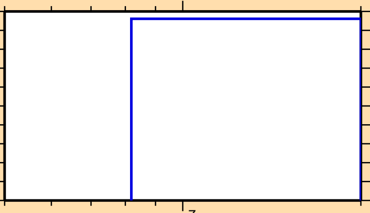
\sigma vs. E for ^{70}\text{Ga}(n,\text{He}3)
