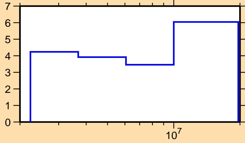
\Delta\sigma/\sigma vs. E for ^{71}\text{Ga}(n,ncont.)
