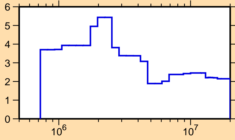
\Delta\sigma/\sigma vs. E for ^{72}\text{Ga}(n,n\text{onel.})
