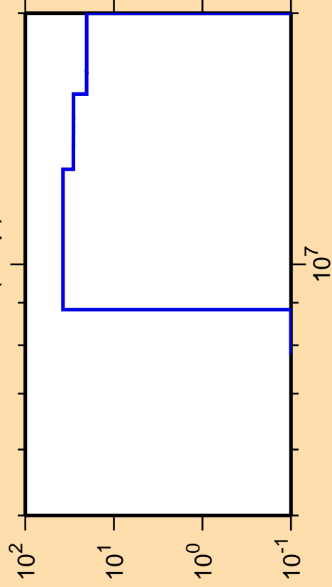
\Delta\sigma/\sigma vs. E for ^{72}\text{Ga}(n,np)
