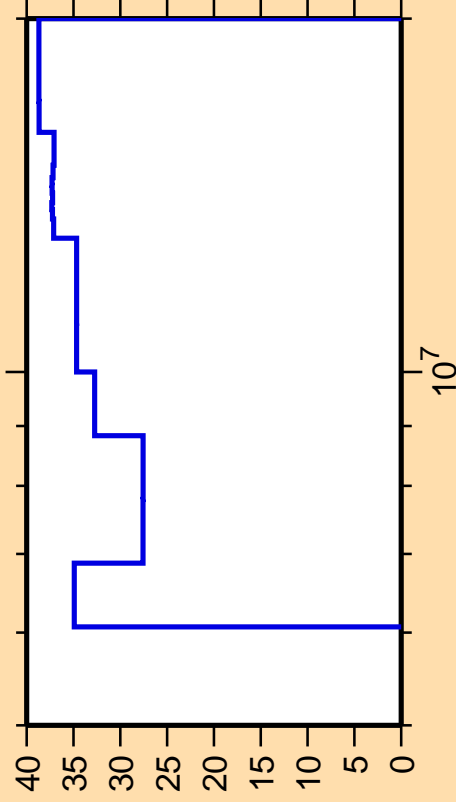
\Delta\sigma/\sigma vs. E for ^{72}\text{Ga}(n,\gamma)
