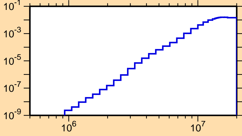
\sigma vs. E for ^{72}\text{Ga}(n,\alpha)
