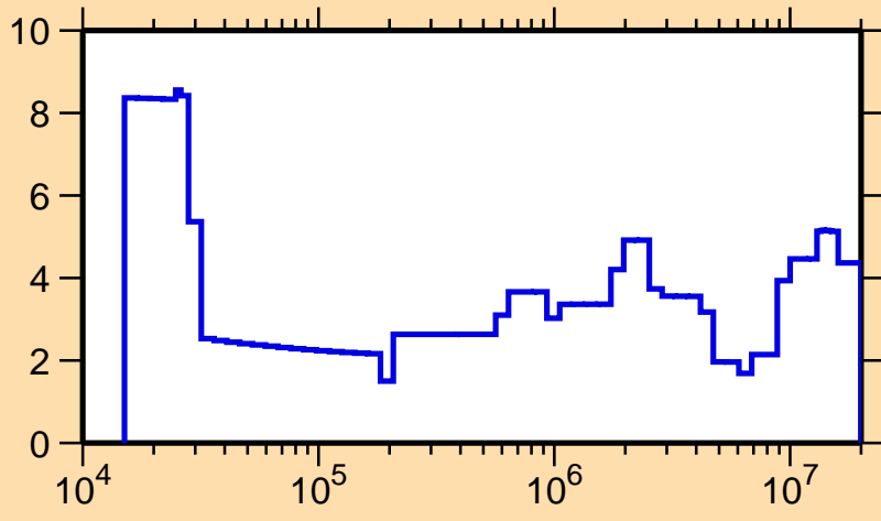
\Delta\sigma/\sigma vs. E for ^{72}\text{Ga}(n,\text{el.})
