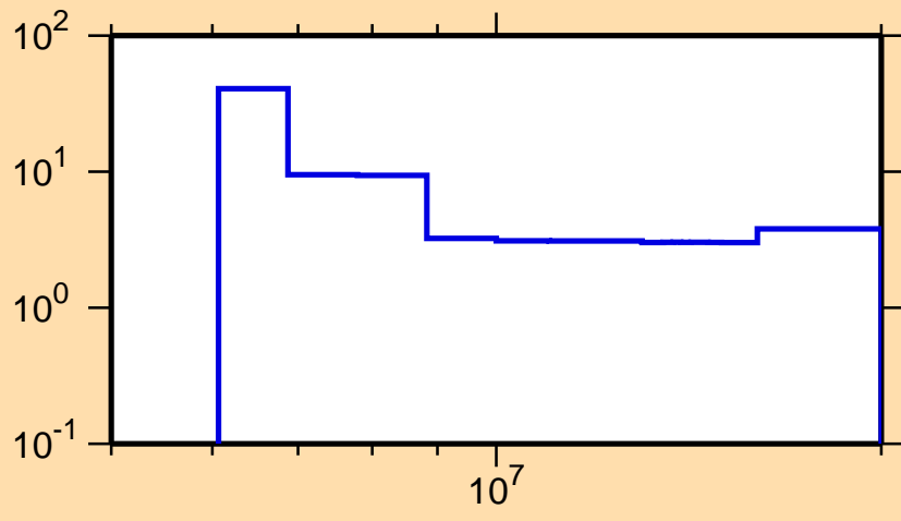
\Delta\sigma/\sigma vs. E for ^{72}\text{Ga}(n,2n)
