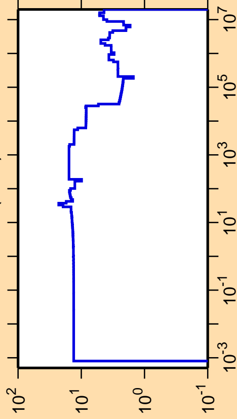
\Delta\sigma/\sigma vs. E for ^{72}\text{Ga}(n,\text{el.})
