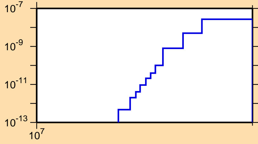
\sigma vs. E for ^{72}\text{Ga}(n,p\alpha)
