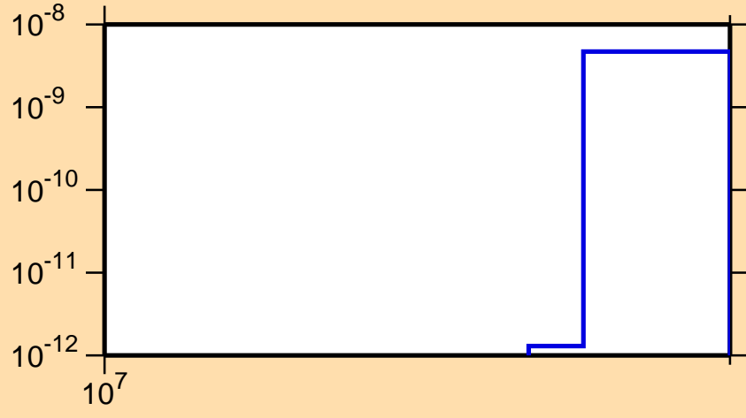
\sigma vs. E for ^{72}\text{Ga}(n,\text{He}3)
