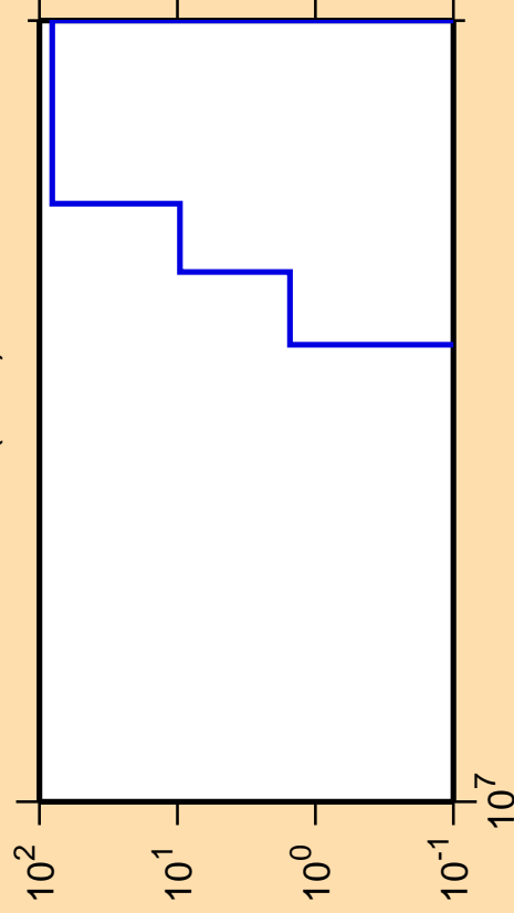
\Delta\sigma/\sigma vs. E for ^{72}\text{Ga}(n,nt)
