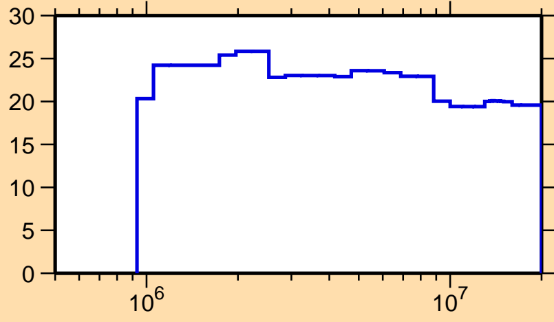
\Delta\sigma/\sigma vs. E for ^{72}\text{Ga}(n,p)
