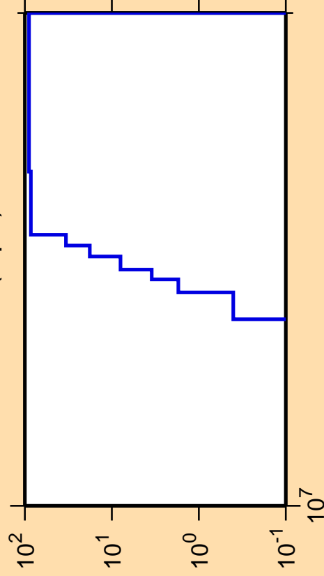
\Delta\sigma/\sigma vs. E for ^{72}\text{Ga}(n,p\alpha)
