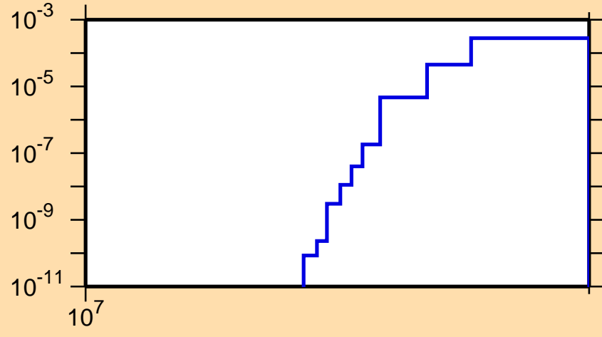
\sigma vs. E for ^{72}\text{Ga}(n,\text{nd})
