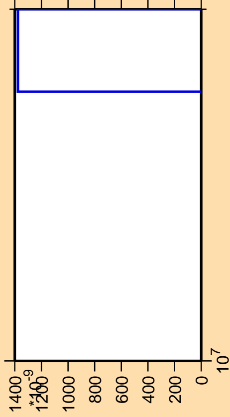
\Delta\sigma/\sigma vs. E for ^{72}\text{Ga}(n,\text{pd})
