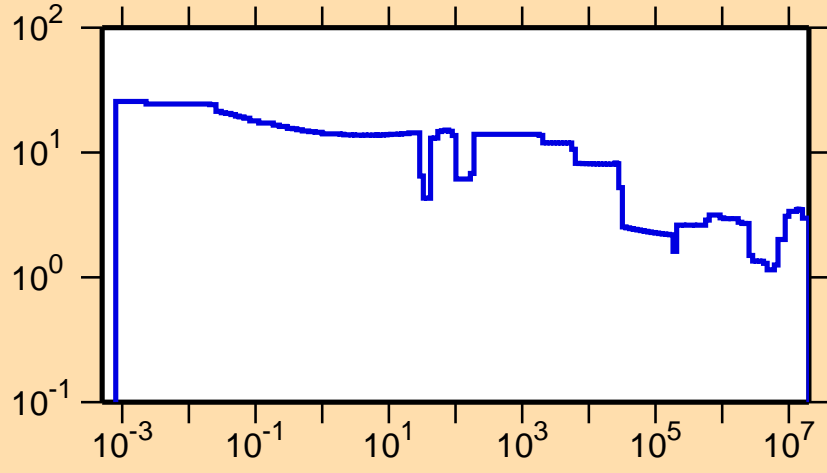
\Delta\sigma/\sigma vs. E for ^{72}\text{Ga}(n,\text{tot.})
