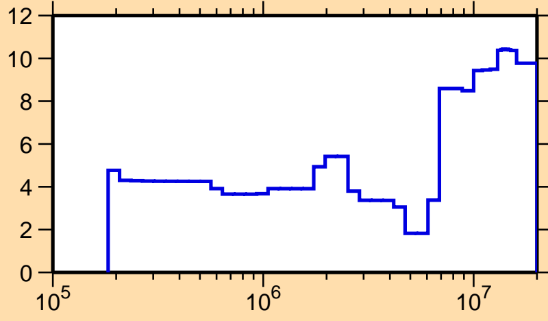
\Delta\sigma/\sigma vs. E for ^{72}\text{Ga}(n,\text{inel.})
