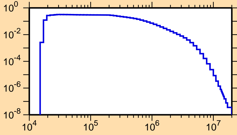
\sigma vs. E for ^{72}\text{Ga}(n,n_1)
