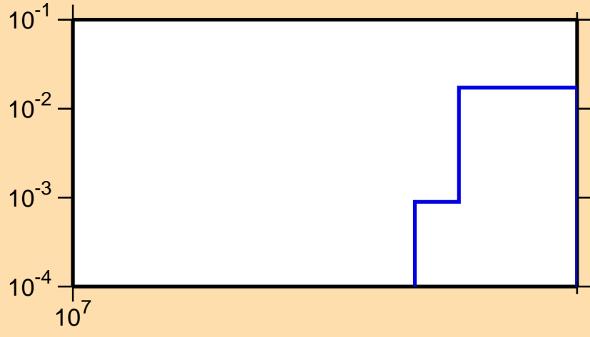
\sigma vs. E for ^{72}\text{Ga}(n,3n)
