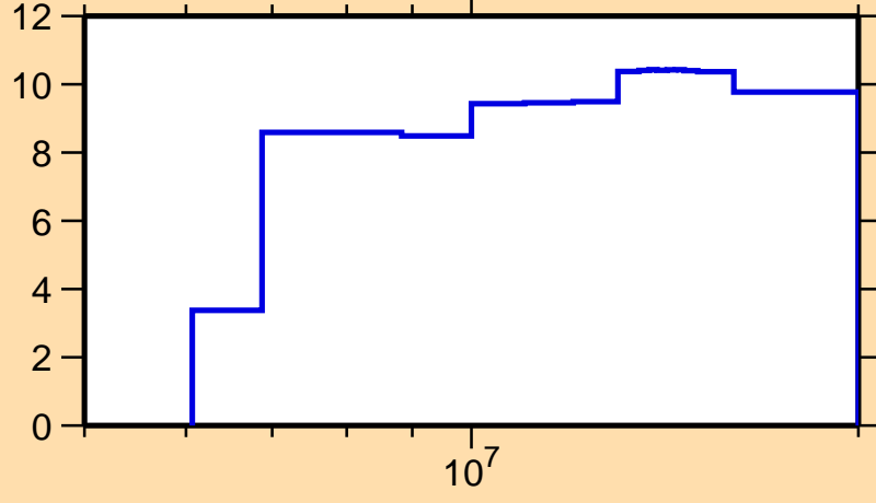
\Delta\sigma/\sigma vs. E for ^{72}\text{Ga}(n,\text{inel.})
