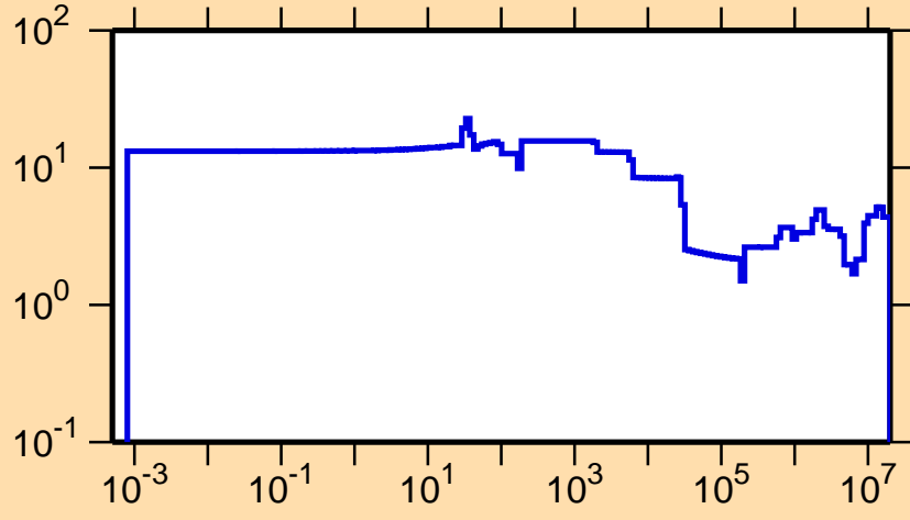
\Delta\sigma/\sigma vs. E for ^{72}\text{Ga}(n,\text{el.})
