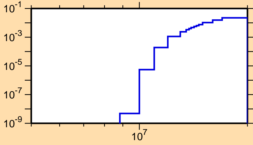
\sigma vs. E for ^{72}\text{Ga}(n,np)
