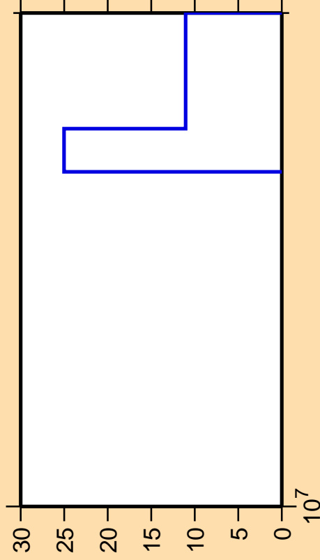
\Delta\sigma/\sigma vs. E for ^{72}\text{Ga}(n,3n)
