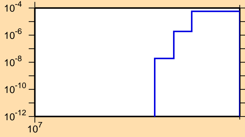
\sigma vs. E for ^{72}\text{Ga}(n,2np)
