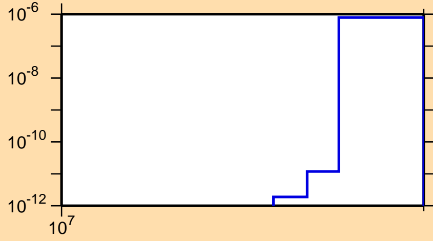
\sigma vs. E for ^{72}\text{Ga}(n,nt)
