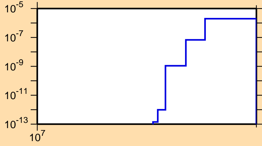
\sigma vs. E for ^{72}\text{Ga}(n,2n\alpha)
