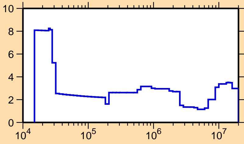
\Delta\sigma/\sigma vs. E for ^{72}\text{Ga}(n,\text{tot.})
