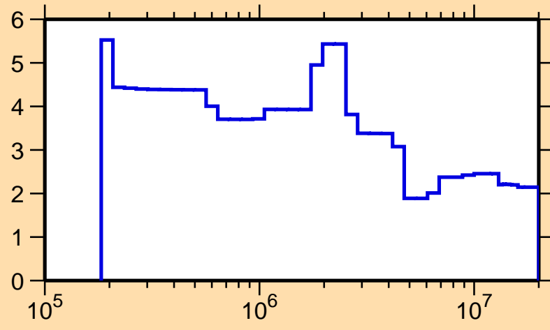
\Delta\sigma/\sigma vs. E for ^{72}\text{Ga}(n,\text{nonel.})
