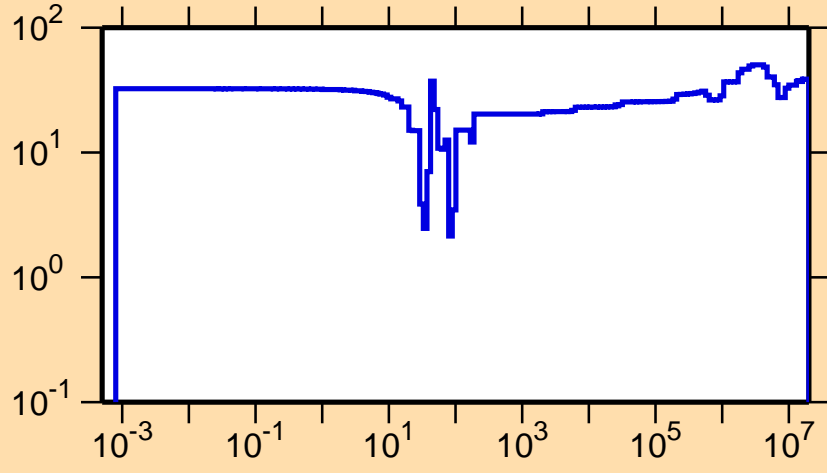
\Delta\sigma/\sigma vs. E for ^{72}\text{Ga}(n,\gamma)
