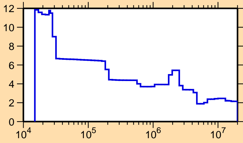
\Delta\sigma/\sigma vs. E for ^{72}\text{Ga}(n,\text{nonel.})
