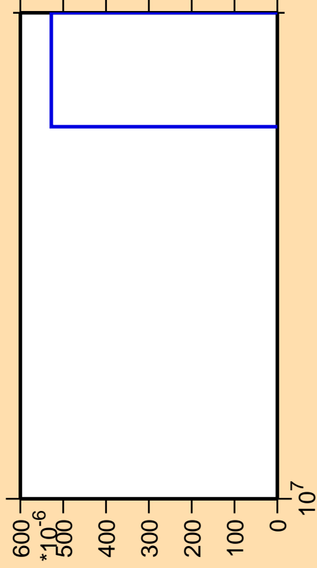
\Delta\sigma/\sigma vs. E for ^{72}\text{Ga} (mt 34)
