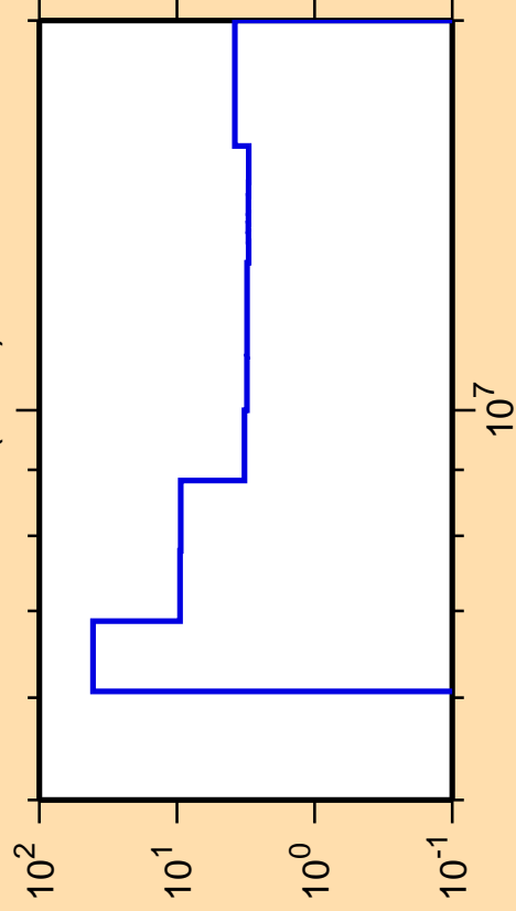
\Delta\sigma/\sigma vs. E for ^{72}\text{Ga}(n,2n)
