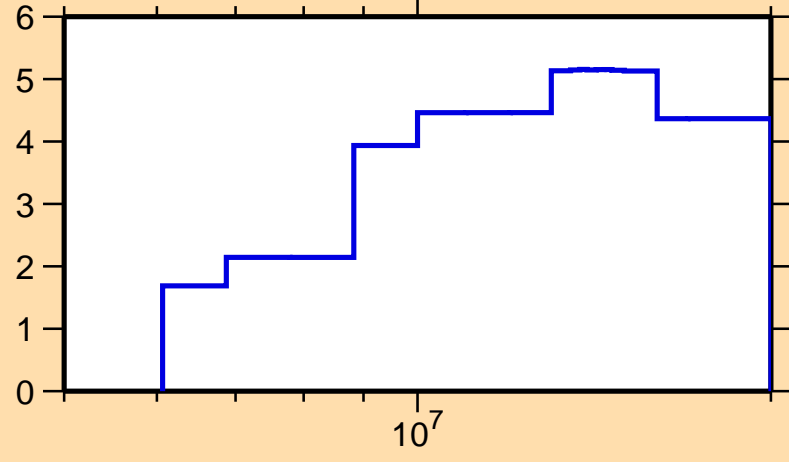
\Delta\sigma/\sigma vs. E for ^{72}\text{Ga}(n,\text{el.})
