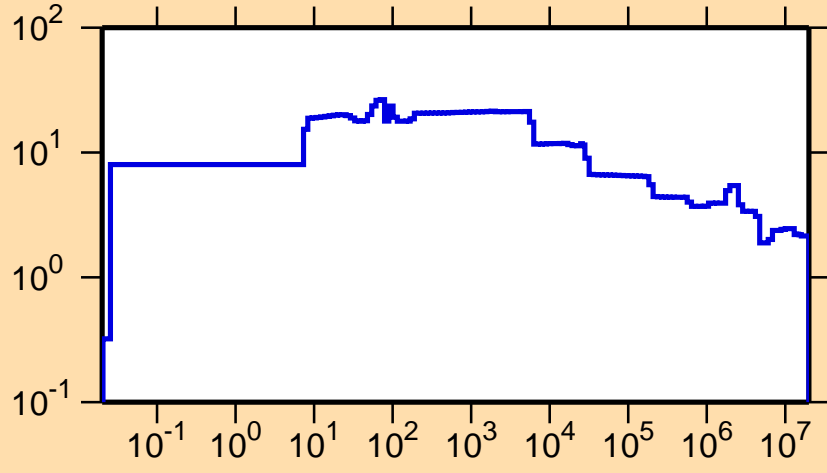
\Delta\sigma/\sigma vs. E for ^{72}\text{Ga}(n,\text{nonel.})
