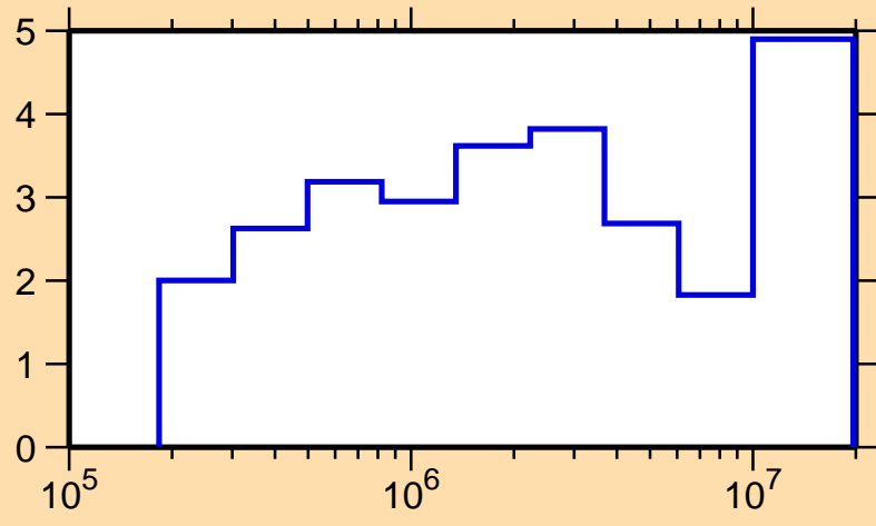
\Delta\sigma/\sigma vs. E for ^{72}\text{Ga}(n,el.)
