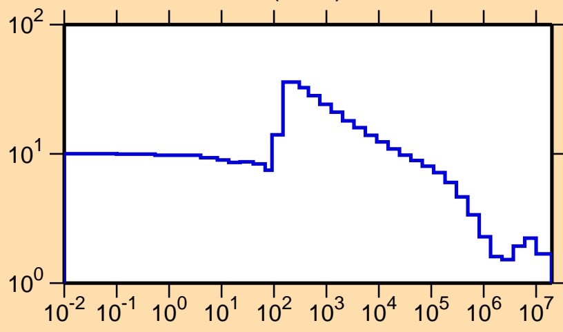
\sigma vs. E for ^{72}\text{Ga}(n,\text{el.})
