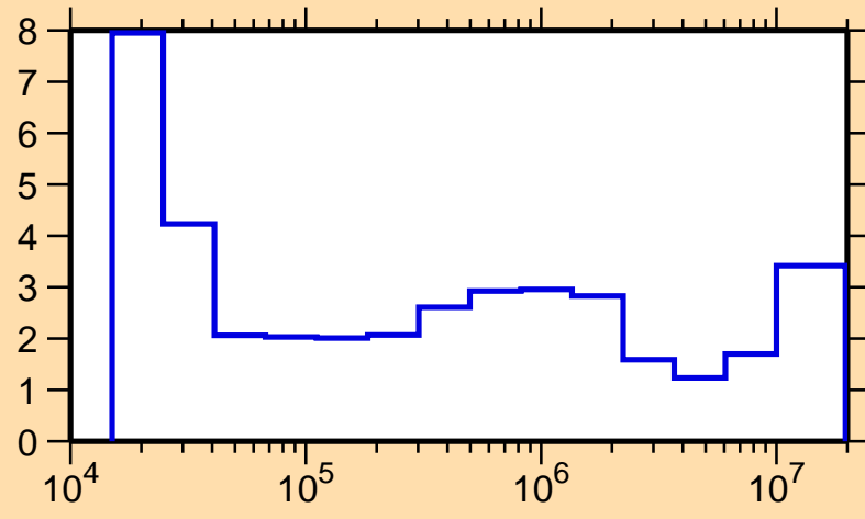
\Delta\sigma/\sigma vs. E for ^{72}\text{Ga}(n,\text{tot.})
