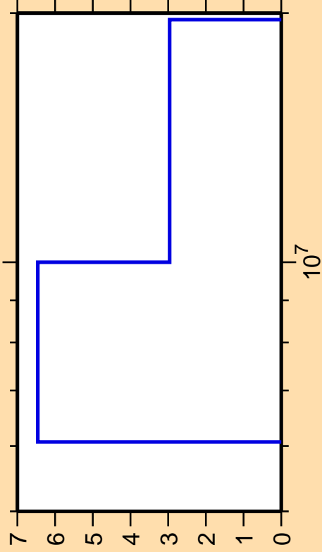
\Delta\sigma/\sigma vs. E for ^{72}\text{Ga}(n,2n)
