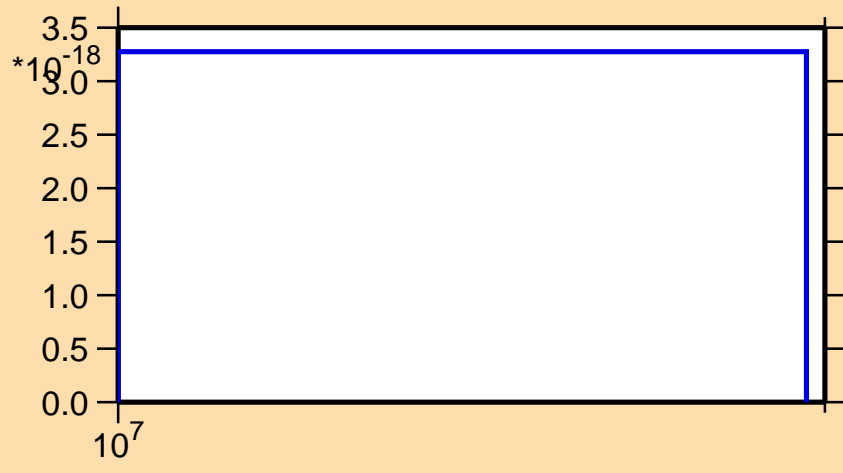
\sigma vs. E for ^{72}\text{Ga} (mt 34)
