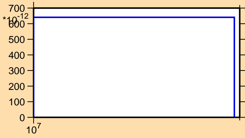
\sigma vs. E for ^{72}\text{Ga}(n,p\alpha)
