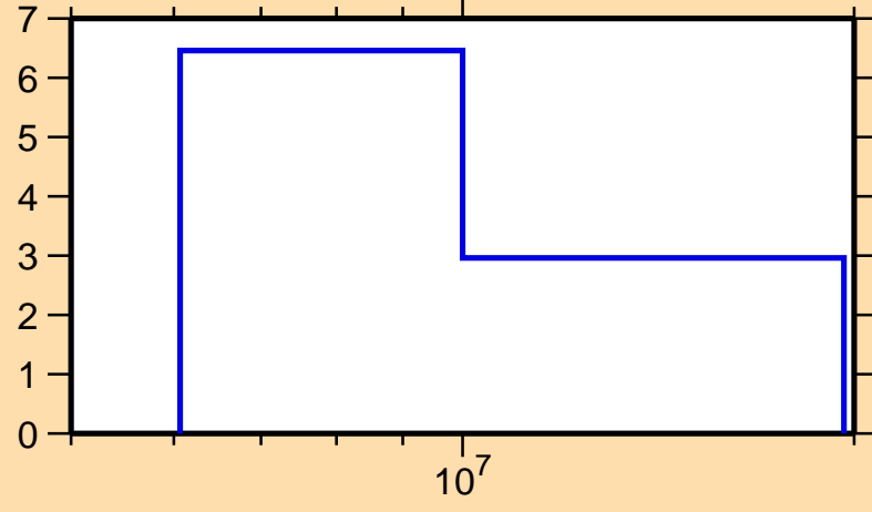
\Delta\sigma/\sigma vs. E for ^{72}\text{Ga}(n,2n)
