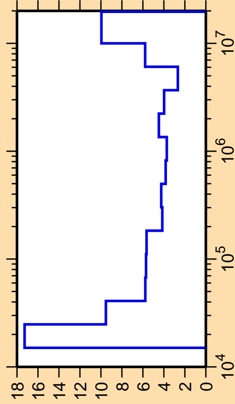
\Delta\sigma/\sigma vs. E for ^{72}\text{Ga}(n,\text{inel.})
