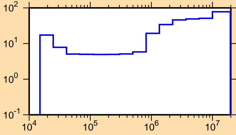
\Delta\sigma/\sigma vs. E for ^{72}\text{Ga}(n,n_1)
