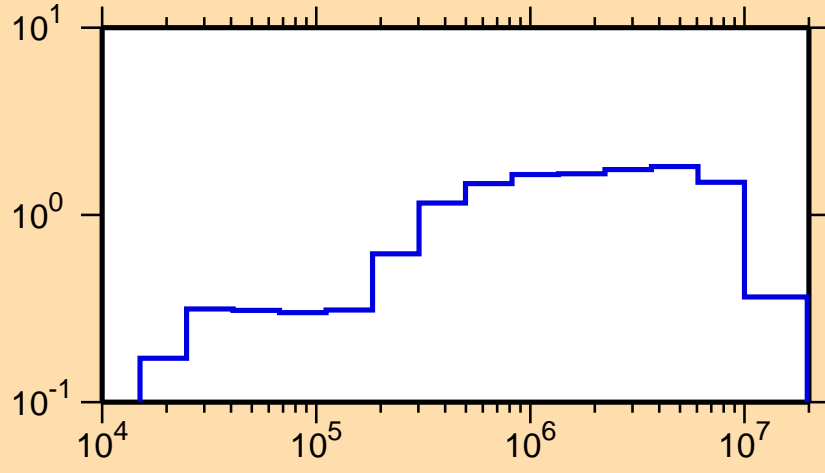
\sigma vs. E for ^{72}\text{Ga}(n,\text{inel.})
