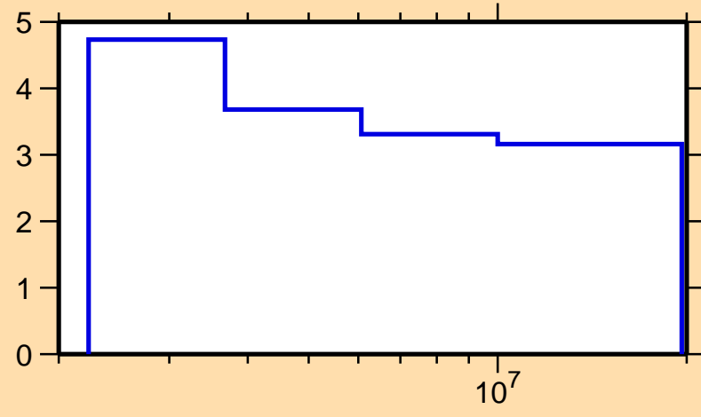
\Delta\sigma/\sigma vs. E for ^{73}\text{Ga}(n,n\text{inel.})
