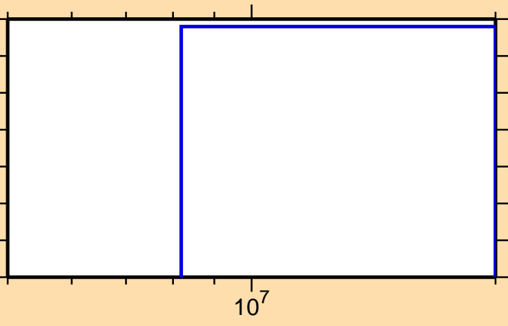
\sigma vs. E for ^{73}\text{Ga}(n,\text{nd})
