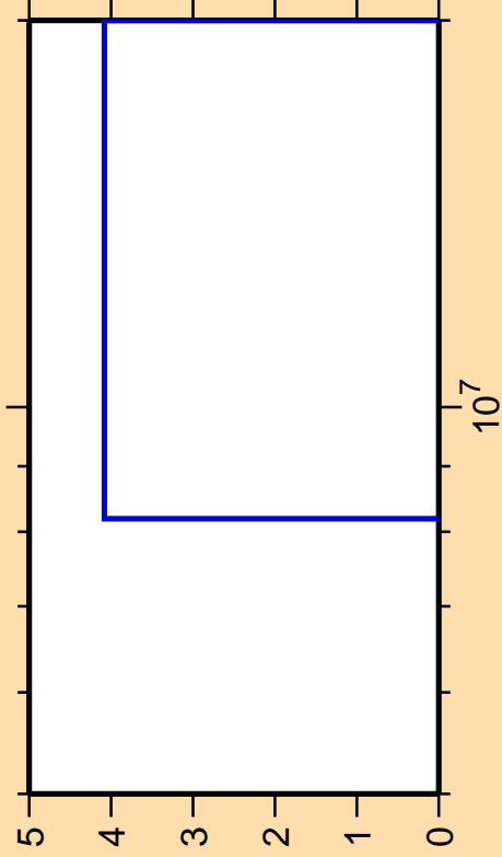
\Delta\sigma/\sigma vs. E for ^{73}\text{Ga}(n,2np)
