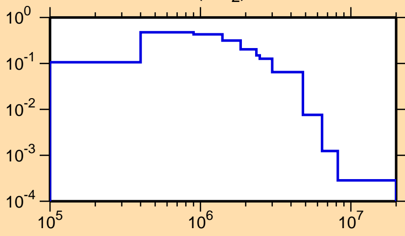
\sigma vs. E for ^{73}\text{Ga}(n,n_2)
