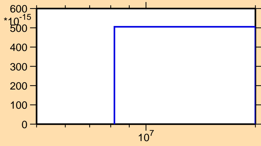
\sigma vs. E for ^{73}\text{Ga}(n,2n\alpha)
