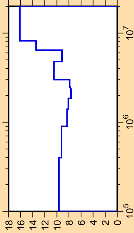
\Delta\sigma/\sigma vs. E for ^{73}\text{Ga}(n,n_2)
