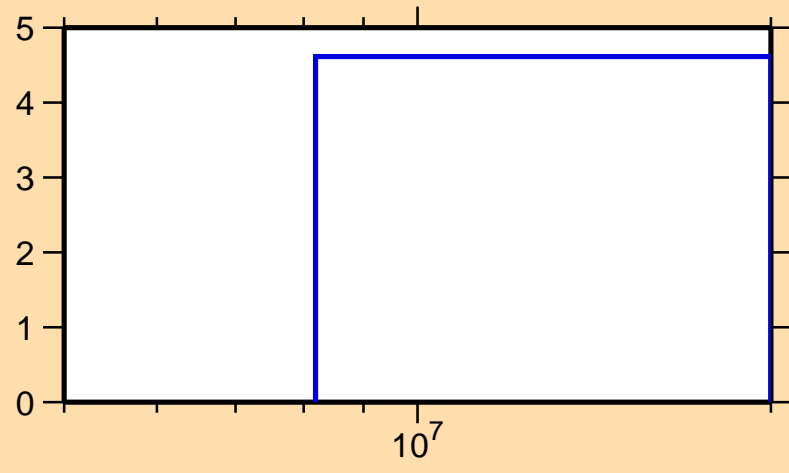
\Delta\sigma/\sigma vs. E for ^{73}\text{Ga}(n,2n)
