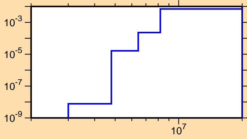
\sigma vs. E for ^{73}\text{Ga}(n,p)
