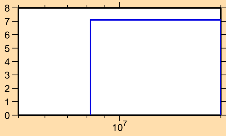
\Delta\sigma/\sigma vs. E for ^{73}\text{Ga}(n,\text{inel.})
