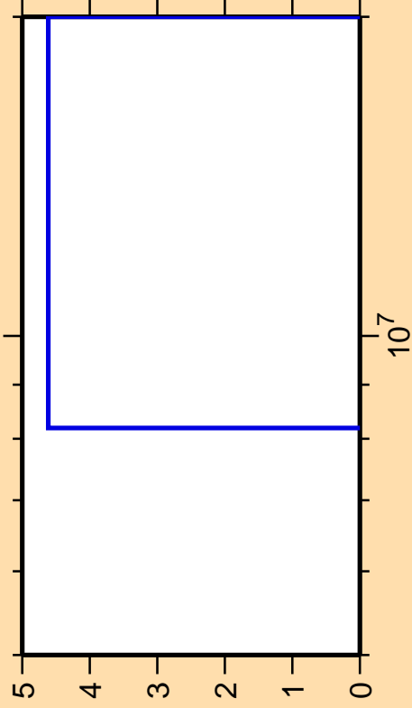
\Delta\sigma/\sigma vs. E for ^{73}\text{Ga}(n,2n)
