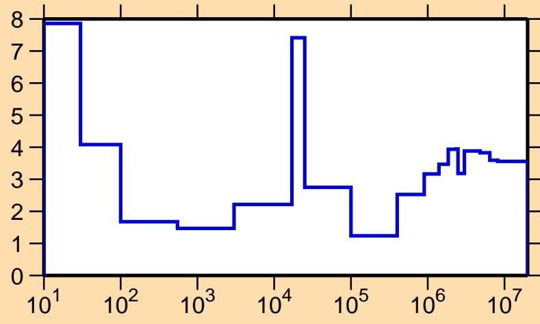
\Delta\sigma/\sigma vs. E for ^{73}\text{Ga}(n,\text{el.})
