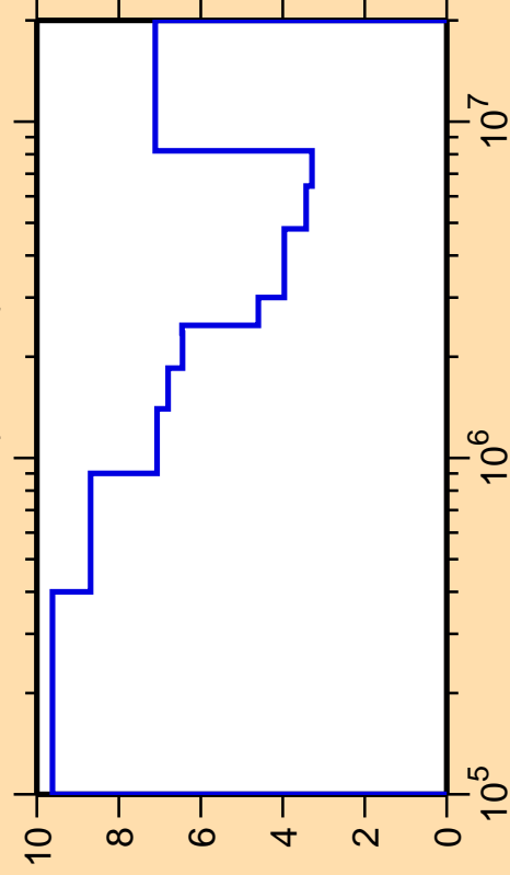
\Delta\sigma/\sigma vs. E for ^{73}\text{Ga}(n,\text{inel.})
