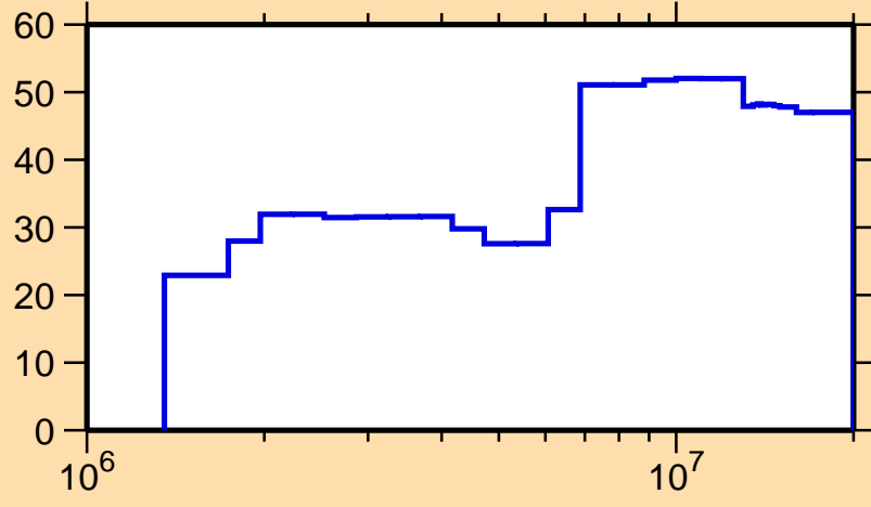
\Delta\sigma/\sigma vs. E for ^{74}\text{Ga}(n,\gamma)
