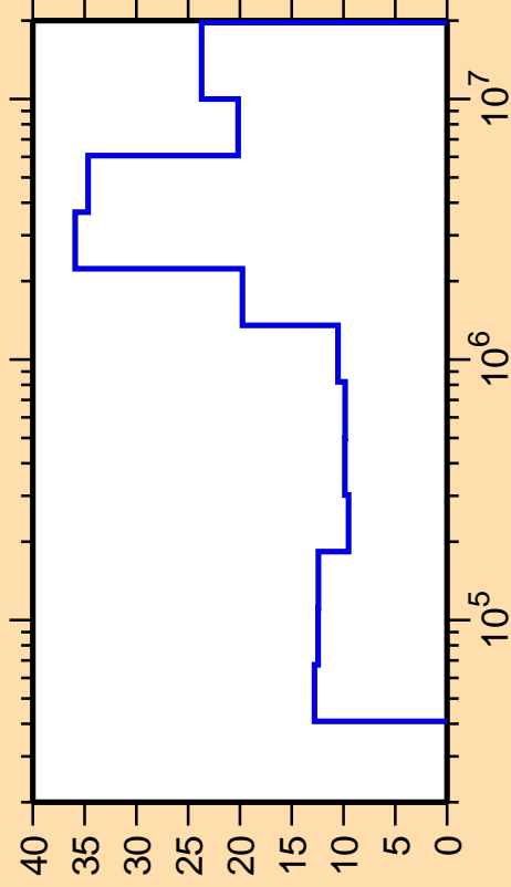
\Delta\sigma/\sigma vs. E for ^{74}\text{Ga}(n,n_3)
