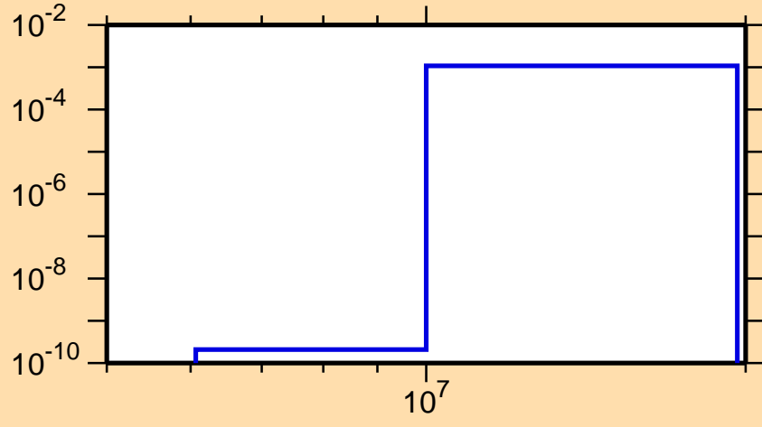
\sigma vs. E for ^{74}\text{Ga}(n,d)
