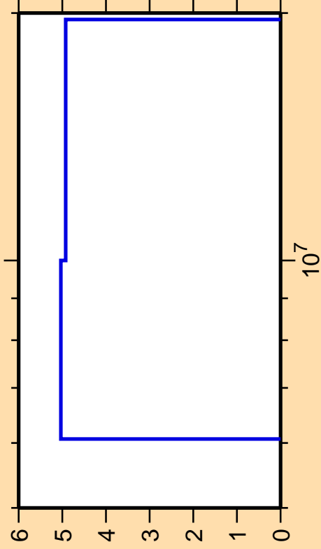
\Delta\sigma/\sigma vs. E for ^{74}\text{Ga}(n,2n)
