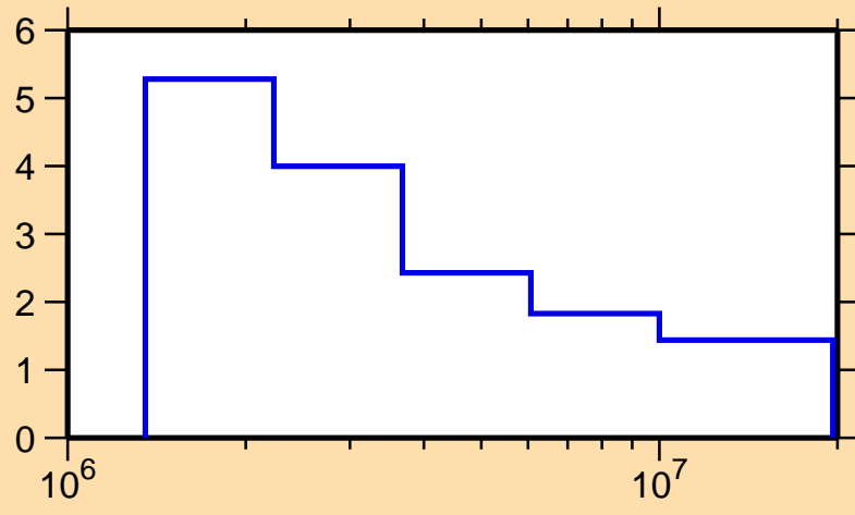
\Delta\sigma/\sigma vs. E for ^{74}\text{Ga}(n,n\text{onel.})
