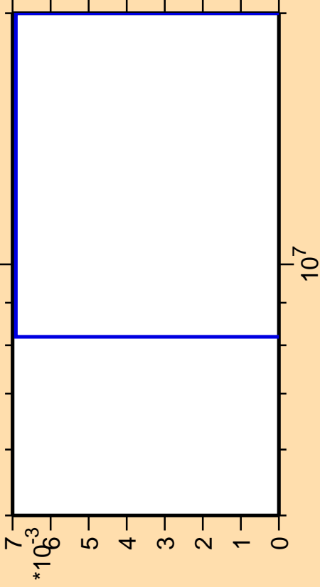
\Delta\sigma/\sigma vs. E for ^{74}\text{Ga}(n,\text{He}3)
