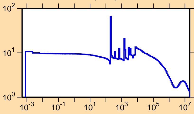
\sigma vs. E for ^{75}\text{Ga}(n,\text{el.})
