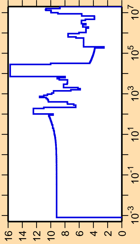
\Delta\sigma/\sigma vs. E for ^{75}\text{Ga}(n,\text{el.})
