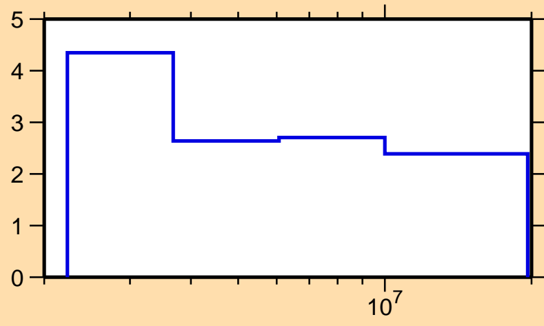
\Delta\sigma/\sigma vs. E for ^{75}\text{Ga}(n,n\text{inel.})
