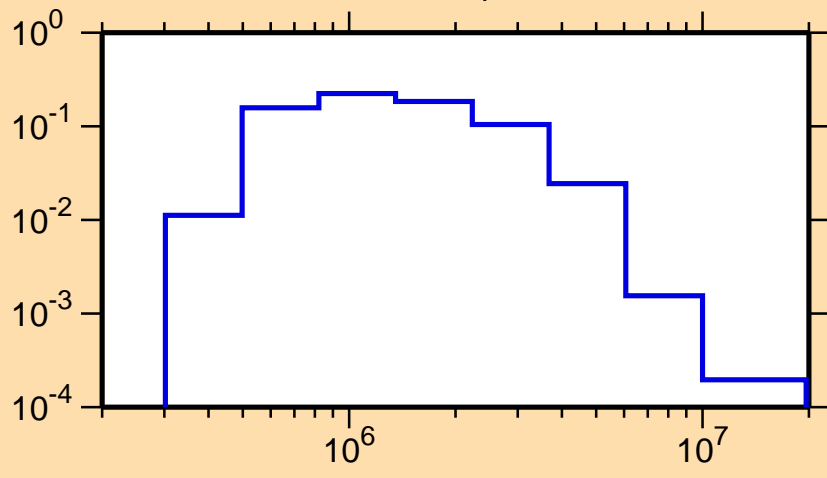
\sigma vs. E for ^{75}\text{Ga}(n,n_4)
