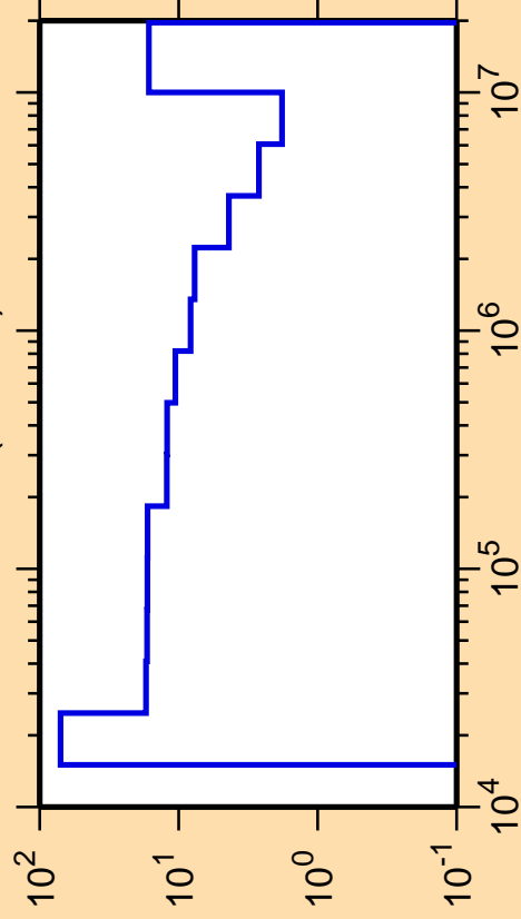
\Delta\sigma/\sigma vs. E for ^{75}\text{Ga}(n,\text{inel.})
