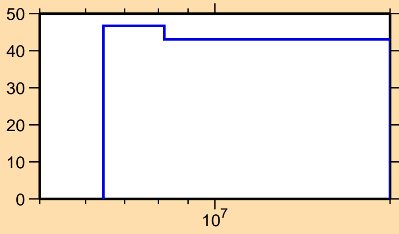
\Delta\sigma/\sigma vs. E for ^{75}\text{Ga}(n,\gamma)
