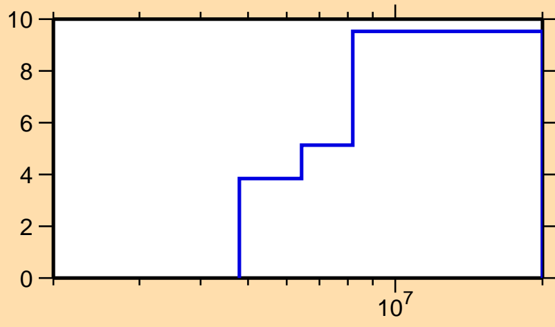
\Delta\sigma/\sigma vs. E for ^{75}\text{Ga}(n,el.)
