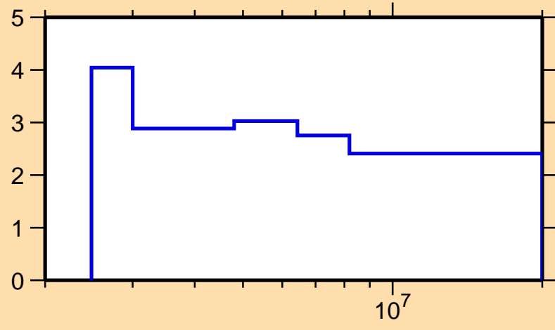
\Delta\sigma/\sigma vs. E for ^{75}\text{Ga}(n,n\text{onel.})
