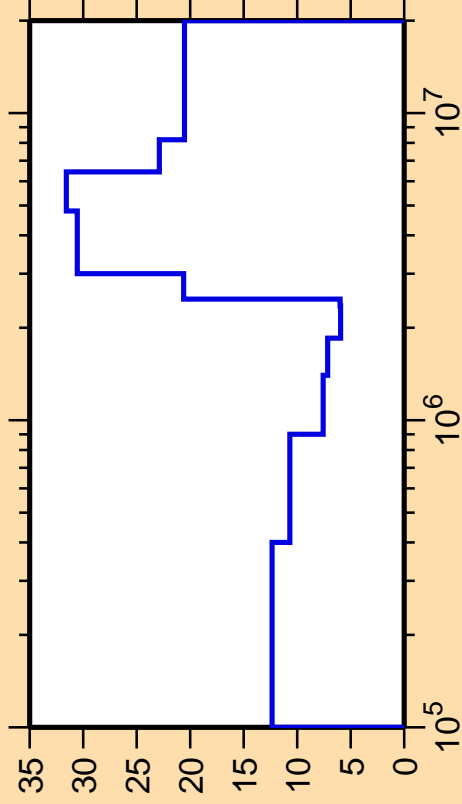
\Delta\sigma/\sigma vs. E for ^{75}\text{Ga}(n,n_2)
