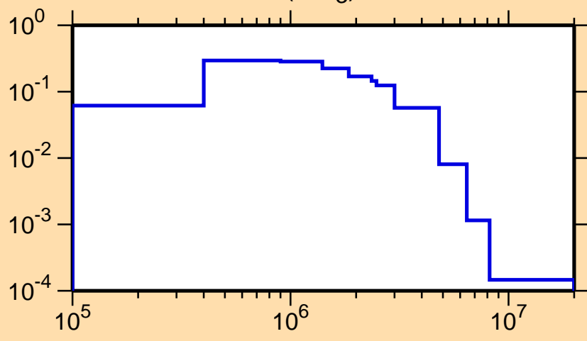
\sigma vs. E for ^{75}\text{Ga}(n,n_3)
