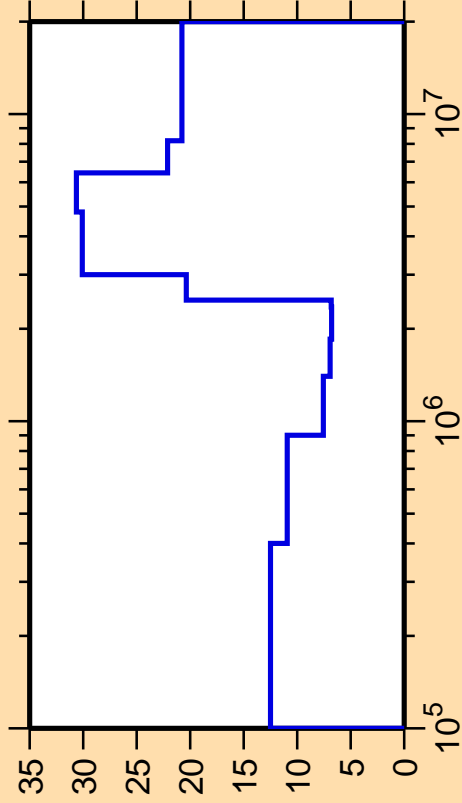
\Delta\sigma/\sigma vs. E for ^{75}\text{Ga}(n,n_3)
