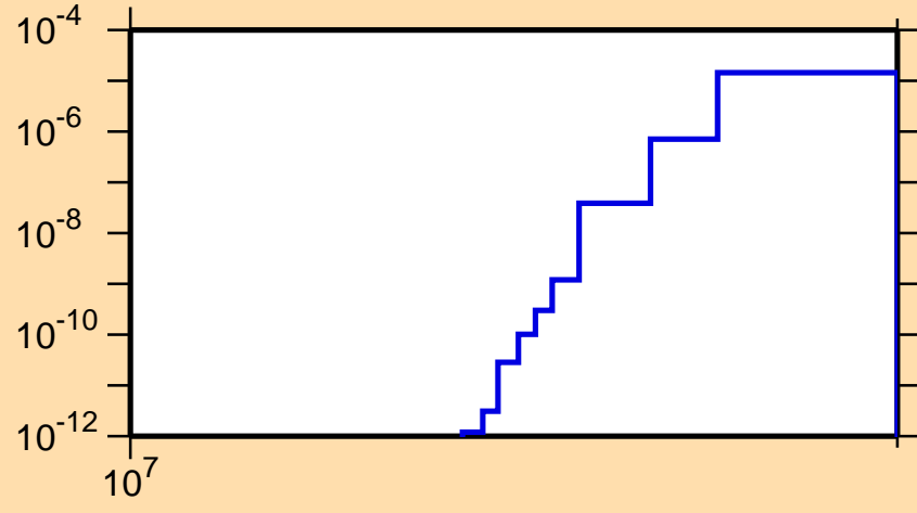
\sigma vs. E for ^{78}\text{Ga}(n,n\alpha)
