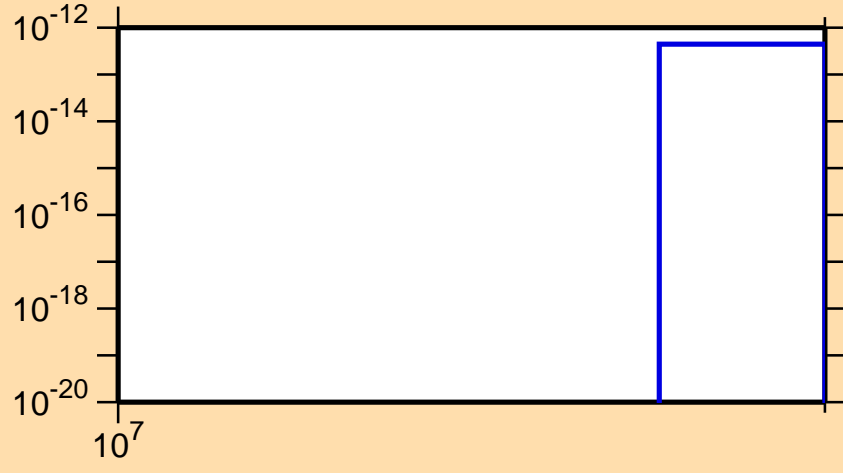
\sigma vs. E for ^{78}\text{Ga}(n,2n\alpha)
