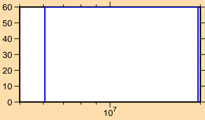
\Delta\sigma/\sigma vs. E for ^{78}\text{Ga}(n,\gamma)
