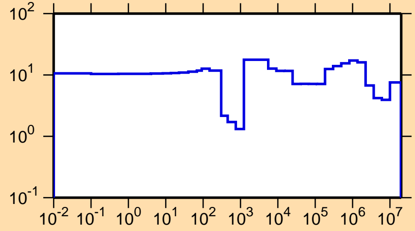
\Delta\sigma/\sigma vs. E for ^{78}\text{Ga}(n,\text{tot.})
