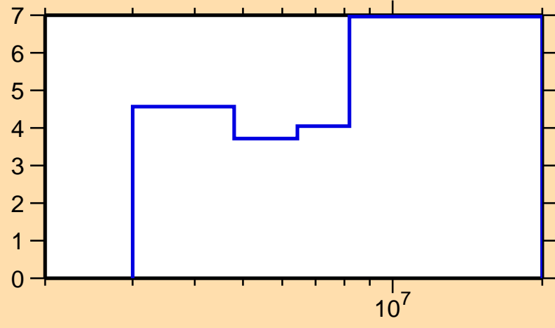
\Delta\sigma/\sigma vs. E for ^{78}\text{Ga}(n,\text{tot.})
