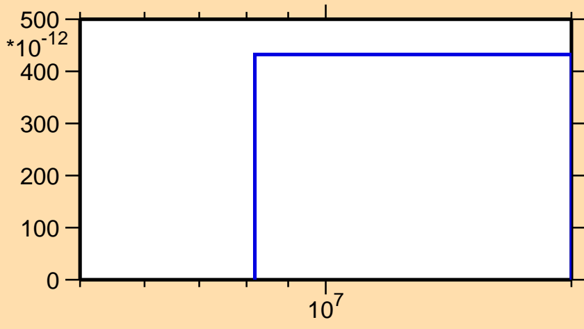
\sigma vs. E for ^{78}\text{Ga}(n,nt)
