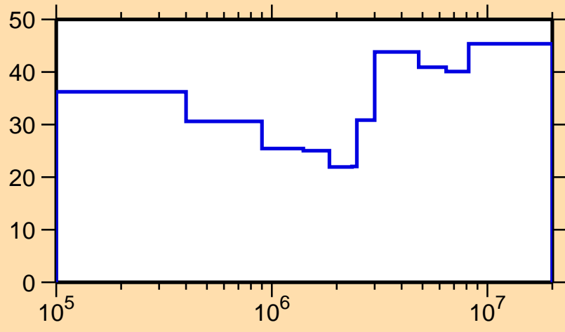
\Delta\sigma/\sigma vs. E for ^{78}\text{Ga}(n,n_1)
