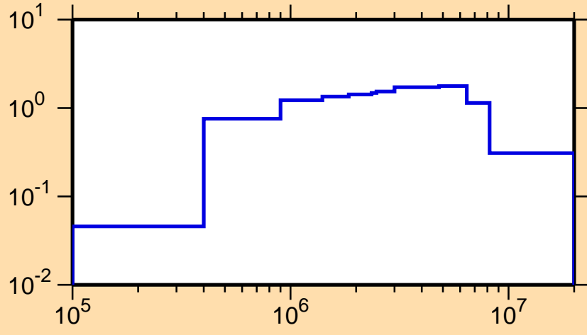
\sigma vs. E for ^{78}\text{Ga}(n,\text{inel.})
