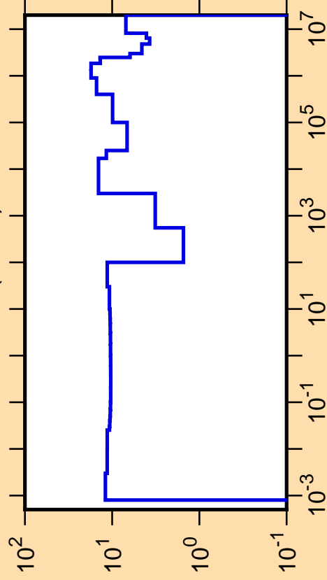
\Delta\sigma/\sigma vs. E for ^{78}\text{Ga}(n,\text{tot.})
