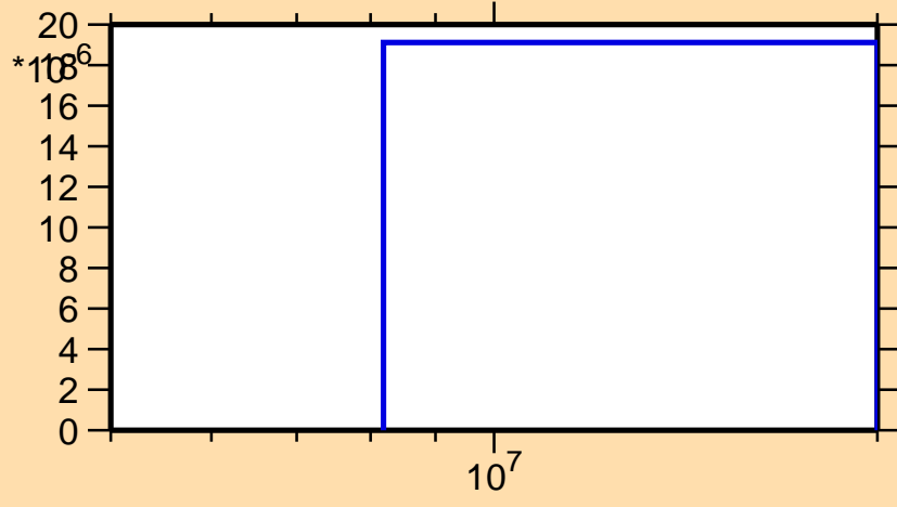
\sigma vs. E for ^{78}\text{Ga}(n,np)
