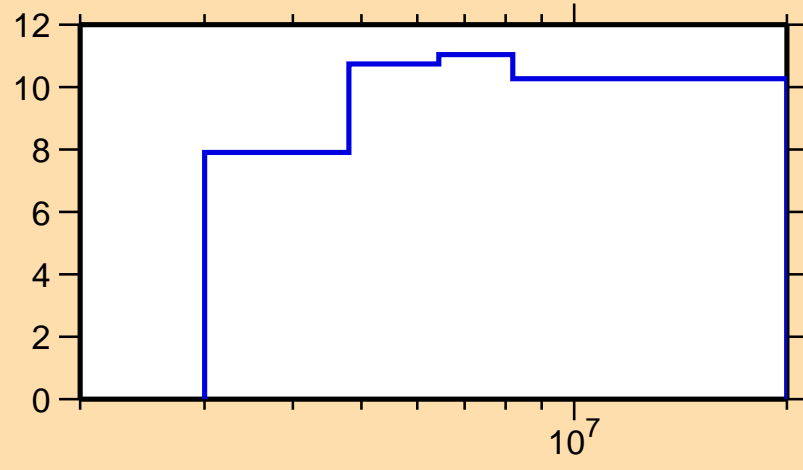
\Delta\sigma/\sigma vs. E for ^{78}\text{Ga}(n,n\text{onel.})
