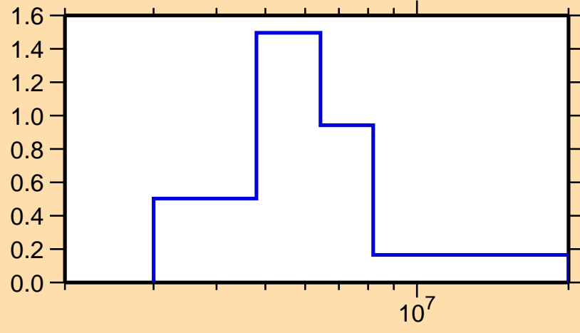
\sigma vs. E for ^{78}\text{Ga}(n,n\text{cont.})
