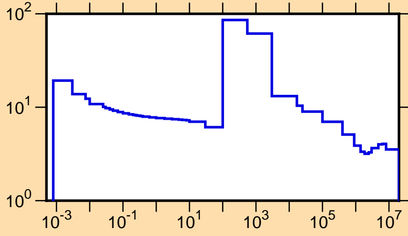
\sigma vs. E for ^{78}\text{Ga}(n,\text{tot.})
