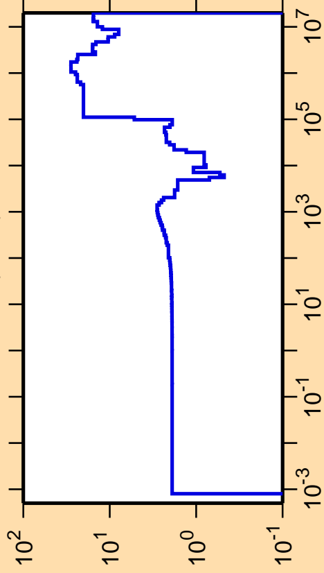
\Delta\sigma/\sigma vs. E for ^{79}\text{Ga}(n,\text{el.})
