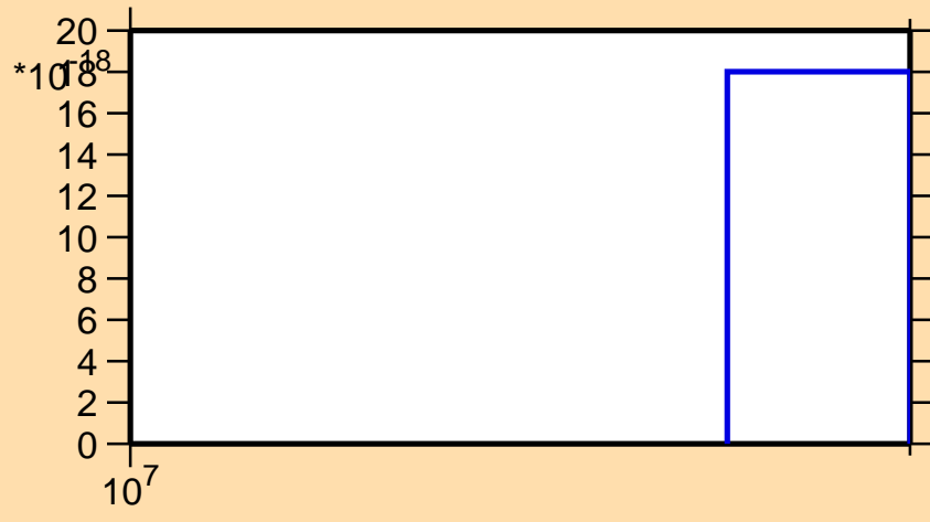
\sigma vs. E for ^{79}\text{Ga}(n,2np)
