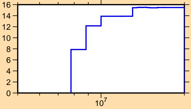
\Delta\sigma/\sigma vs. E for ^{79}\text{Ga}(n,el.)
