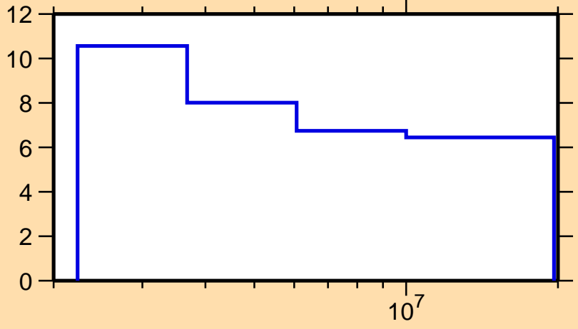
\Delta\sigma/\sigma vs. E for ^{79}\text{Ga}(n,n\text{onel.})
