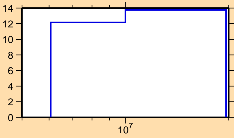
\Delta\sigma/\sigma vs. E for ^{79}\text{Ga}(n,2n)
