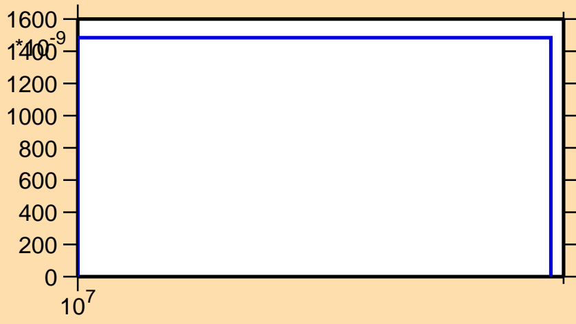
\sigma vs. E for ^{79}\text{Ga}(n,t)
