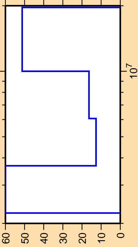
\Delta\sigma/\sigma vs. E for ^{79}\text{Ga}(n,n\text{cont.})
