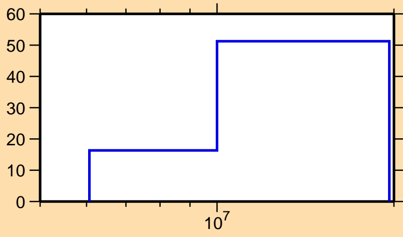
\Delta\sigma/\sigma vs. E for ^{79}\text{Ga}(n,ncont.)
