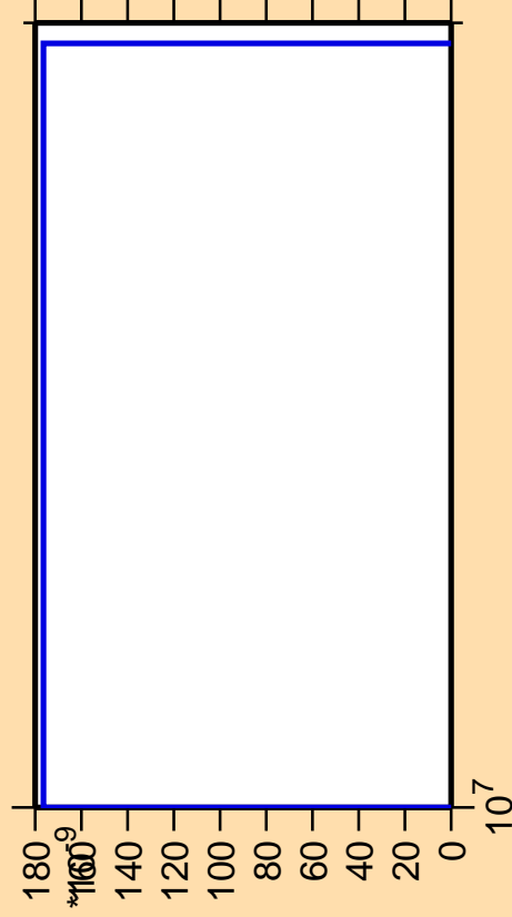
\Delta\sigma/\sigma vs. E for ^{79}\text{Ga}(n,2np)
