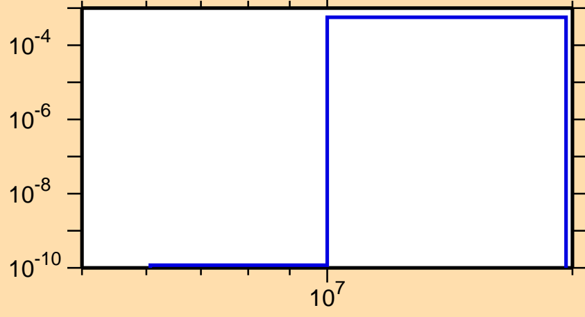
\sigma vs. E for ^{79}\text{Ga}(n,p)
