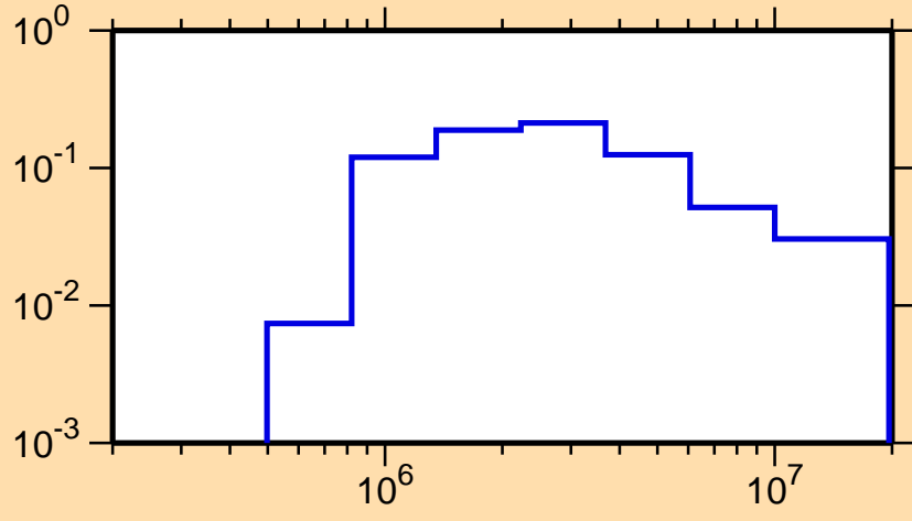
\sigma vs. E for ^{79}\text{Ga}(n,n_3)
