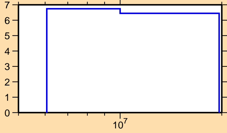
\Delta\sigma/\sigma vs. E for ^{79}\text{Ga}(n,\text{nonel.})
