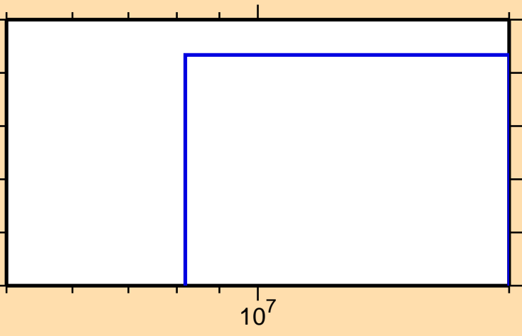
\sigma vs. E for ^{79}\text{Ga}(n,\alpha)
