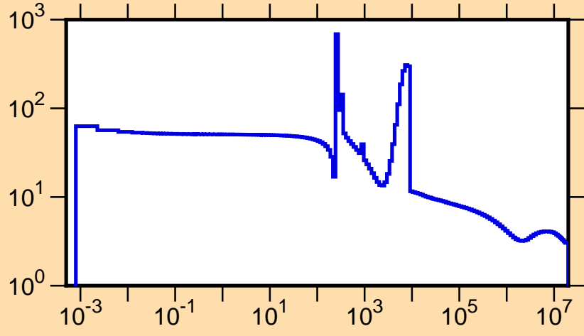
\sigma vs. E for ^{80}\text{Ga}(n,\text{tot.})
