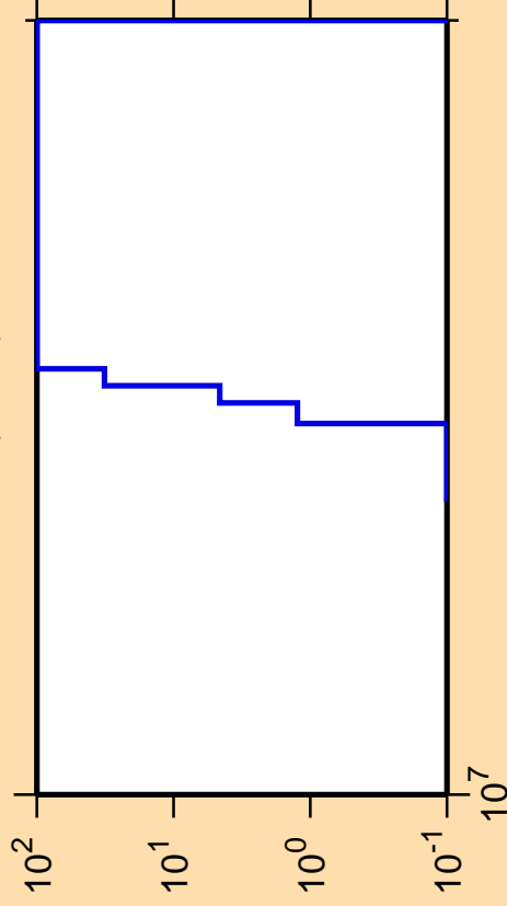
\Delta\sigma/\sigma vs. E for ^{80}\text{Ga}(n,\alpha)
