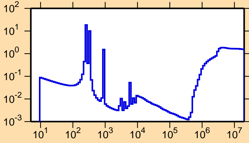
\sigma vs. E for ^{80}\text{Ga}(n,\text{nonel.})
