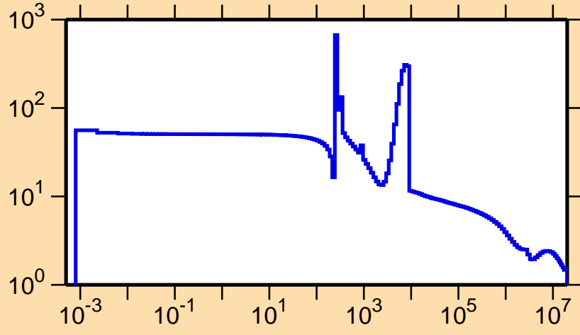
\sigma vs. E for ^{80}\text{Ga}(n,\text{el.})
