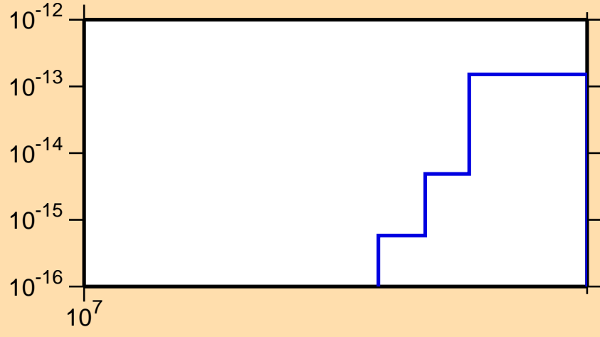
\sigma vs. E for ^{80}\text{Ga}(n,2n\alpha)
