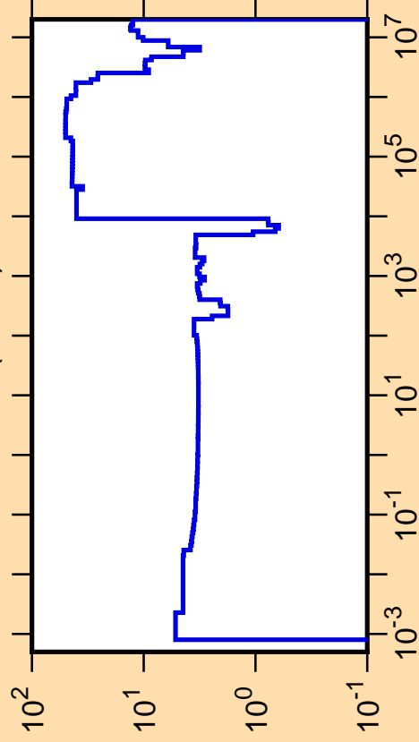
\Delta\sigma/\sigma vs. E for ^{80}\text{Ga}(n,\text{tot.})
