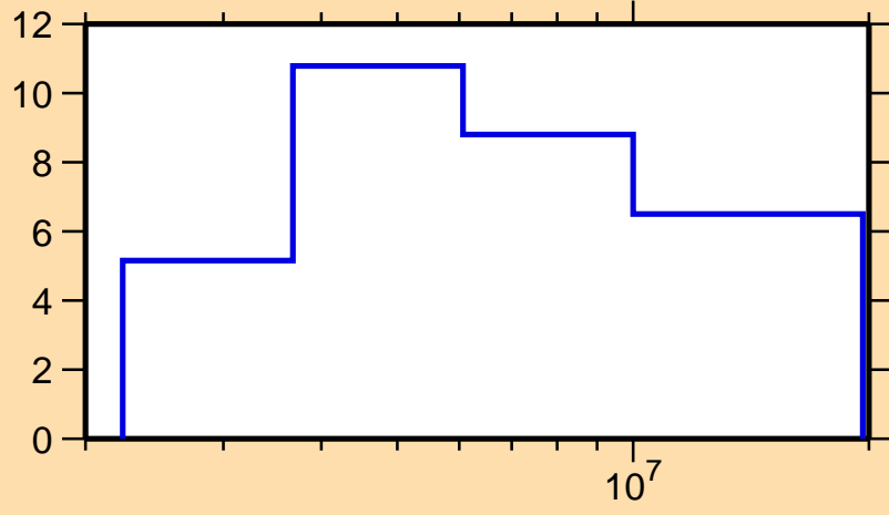
\Delta\sigma/\sigma vs. E for ^{80}\text{Ga}(n,n\text{nonel.})
