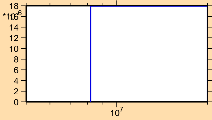
\sigma vs. E for ^{80}\text{Ga}(n,t)
