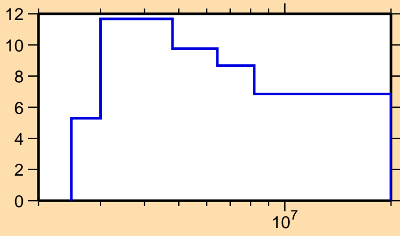
\Delta\sigma/\sigma vs. E for ^{80}\text{Ga}(n,n\text{nonel.})
