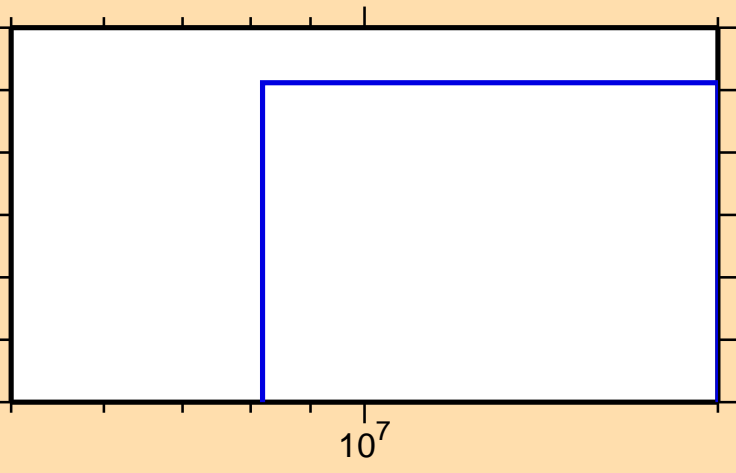
\sigma vs. E for ^{80}\text{Ga}(n,\alpha)
